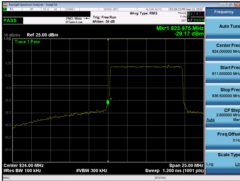
Plot 7-85. Lower Band Edge Plot (NR Band n26/5 - 10.0MHz - Full RB)
