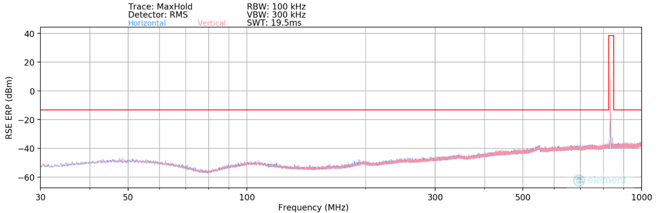
Plot 7-95. Radiated Spurious Plot (ULCA LTE Band 5 - Low channel – Below 1GHz)
