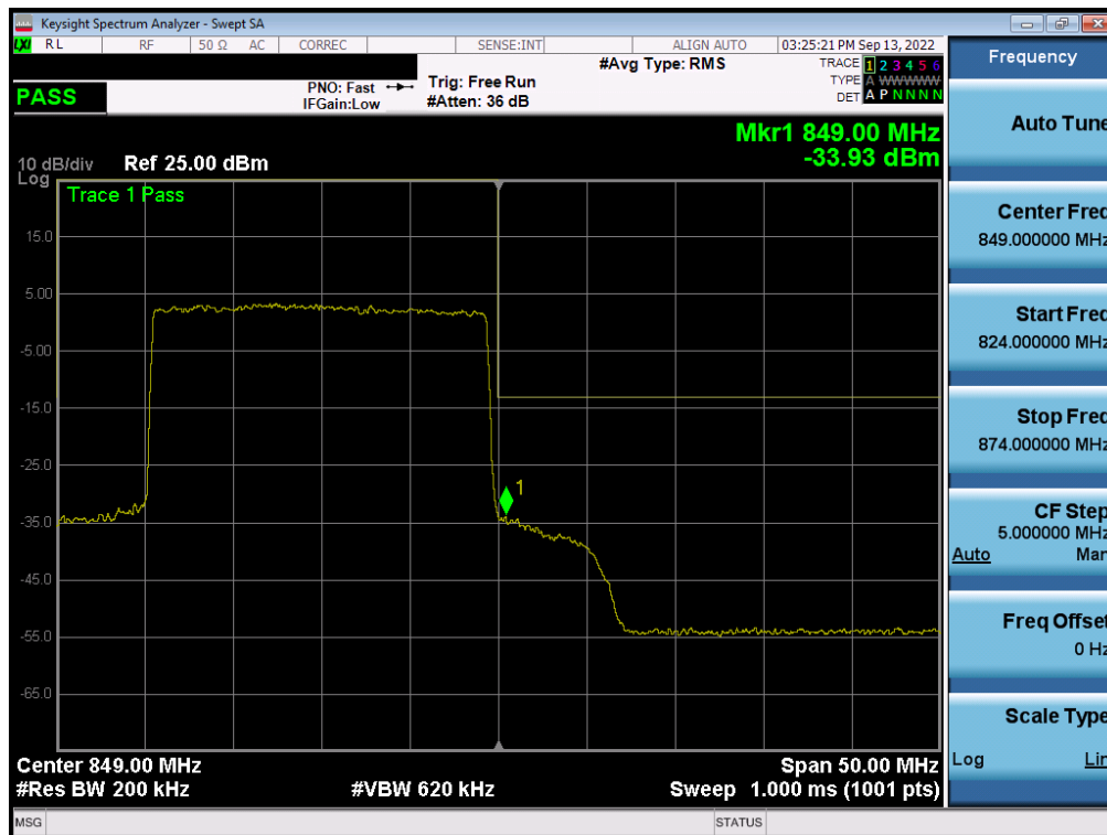
Plot 7-82. Upper Band Edge Plot (NR Band n26/5 – 20.0MHz - Full RB)
