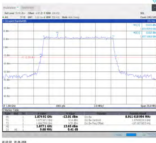
1-N2-15-10-M-2-DFT-PI2BPSK-Outer_Full-50@0-Ant0- 8.911-9.680-≤10-PASS
