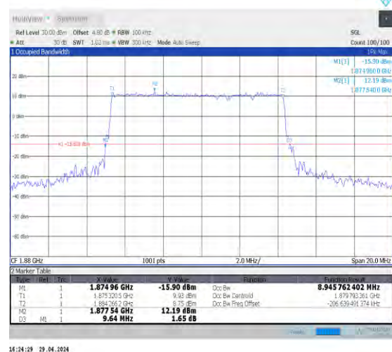
1-N2-15-10-M-3-DFT-16QAM-Outer_Full-50@0-Ant0- -8.946-9.640-≤10-PASS
