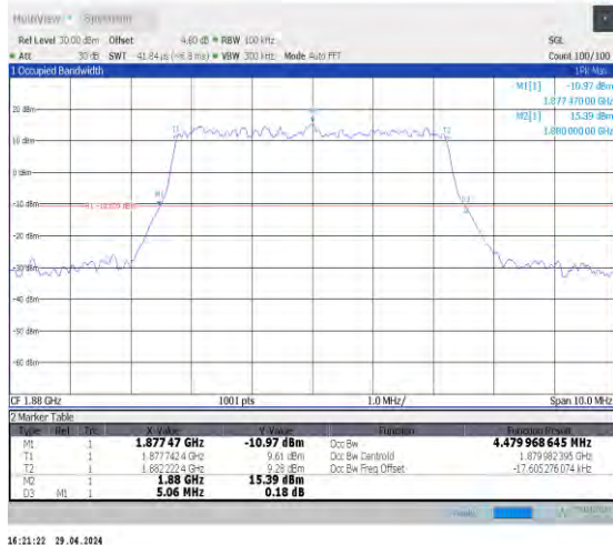
1-N2-15-5-M-3-DFT-16QAM-Outter_Full-25@0-Ant0-4. 4.48-5.060-≤5-PASS
