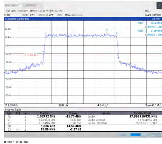
1-N2-15-20-M-3-DFT-16QAM-Outet_Full-100@0-Ant 0-17.927-18.960-≤20-PASS
