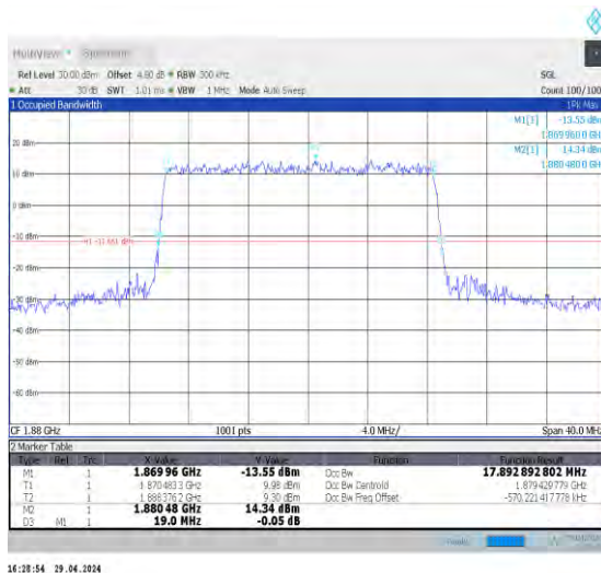
1-N2-15-20-M-4-DFT-64QAM-Outet_Full-100@0-Ant 0-17.893-19.000-≤20-PASS
