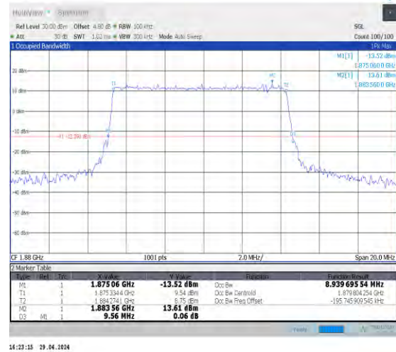
1-N2-15-10-M-1-DFT-QPSK-Outer_Full-50@0-Ant0- 8.94-9.560-≤10-PASS
