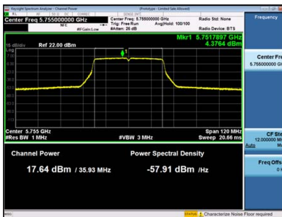
Antenna D
