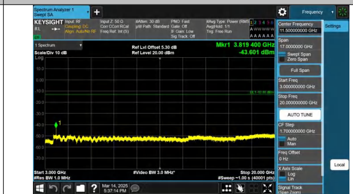
Band2-1.4MHz-QPSK-19193-1RB#5-3000~20000-PASS
