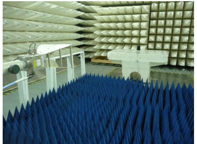
Photograph 8.2.1 Setup for radiated emission measurements, general view
