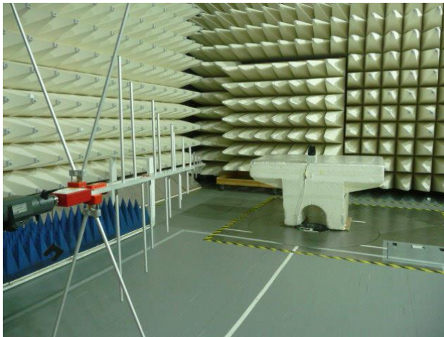
Photograph 8.2.1 Setup for radiated emission measurements, general view
