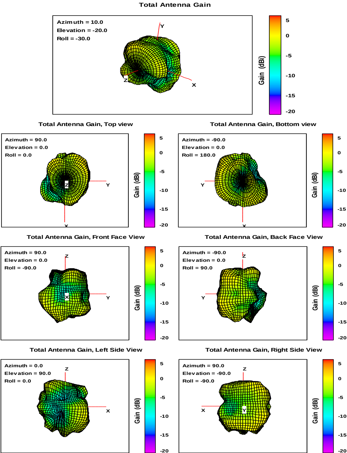
Fig. 10. BT_0 Antenna Gain, BTLE Mid Channel, 2440 MHz.
