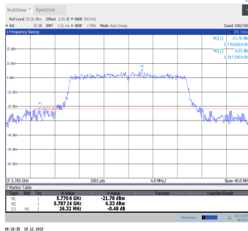
11ax20MIMO-Ant4-5785
