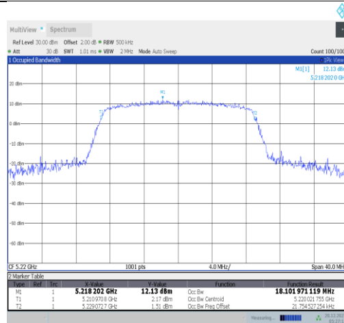
11n20SISO-Ant3-5220
