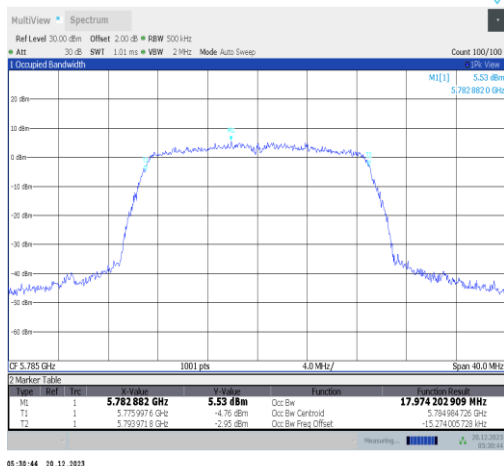
11n20SISO-Ant3-5785
