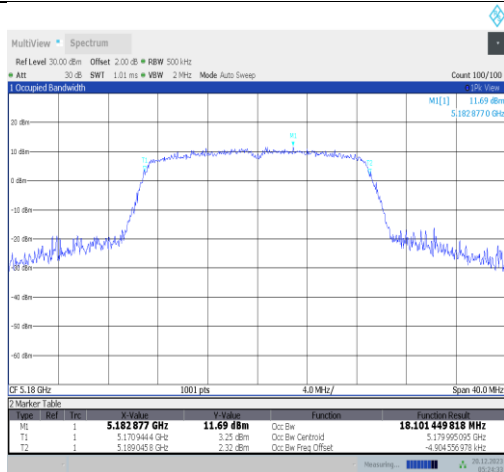
11n20SISO-Ant3-5180
