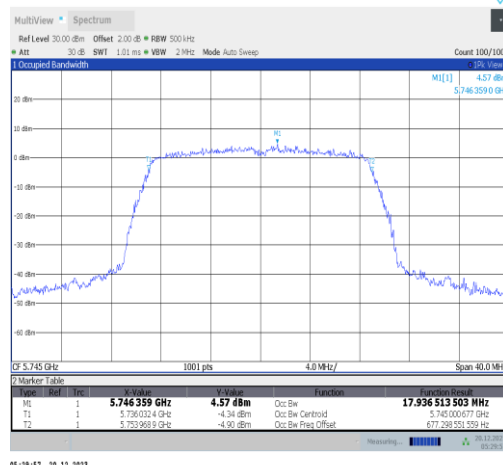
11n20SISO-Ant3-5745
