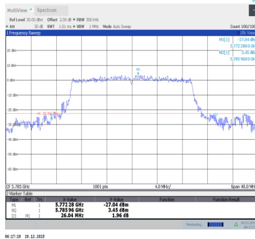
11ax20MIMO-Ant2-5785
