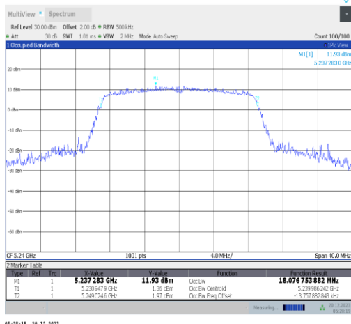
11n20SISO-Ant3-5240
