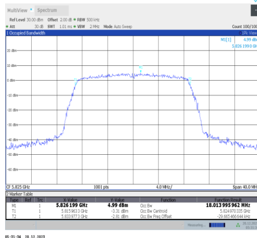
11n20SISO-Ant3-5825
