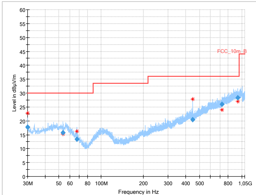
Plot 2: 30 MHz to 1 GHz, TX mode, 2446 MHz, vertical & horizontal polarization, 1 Msps
