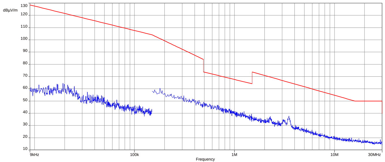
Plot 2: 9 kHz to 30 MHz, 2446 MHz, transmit mode, 1 Msps
