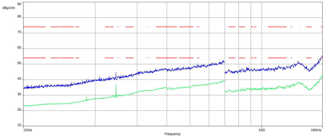
Plot 3: 1 GHz to 18 GHz, TX mode, 2446 MHz, vertical & horizontal polarization, 1 Msp/s
