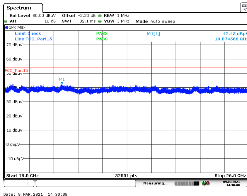
Plot 4: 18 GHz to 26 GHz, TX mode, 2446 MHz, vertical & horizontal polarization, 1 Msp/s
