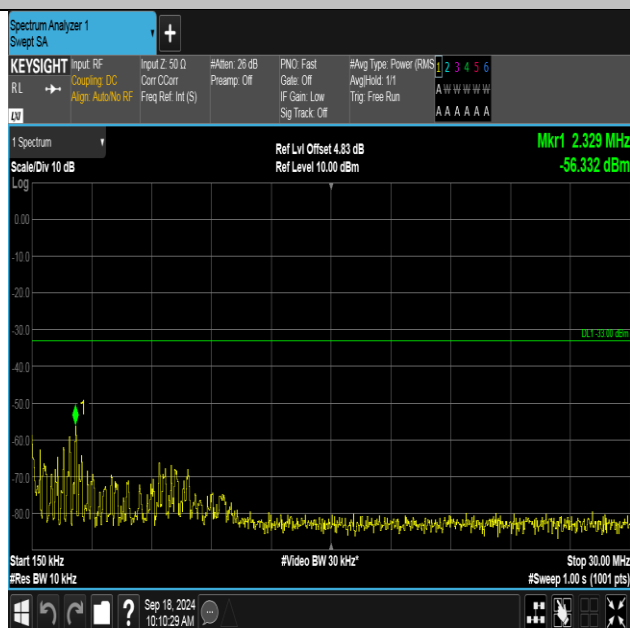
Band2-9538-5-0.15~30MHz-PASS
