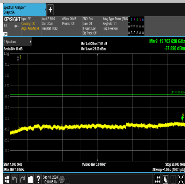
Band2-9400-5-1000~20000MHz-PASS
