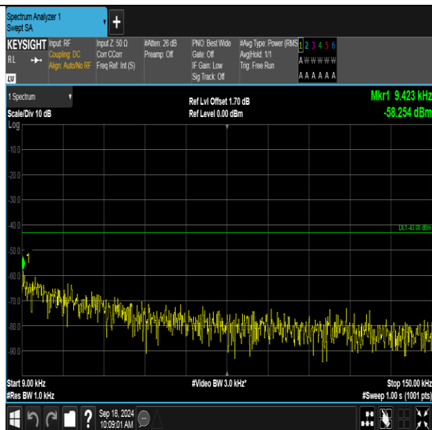
Band2-9262-5-0.009~0.15MHz-PASS
