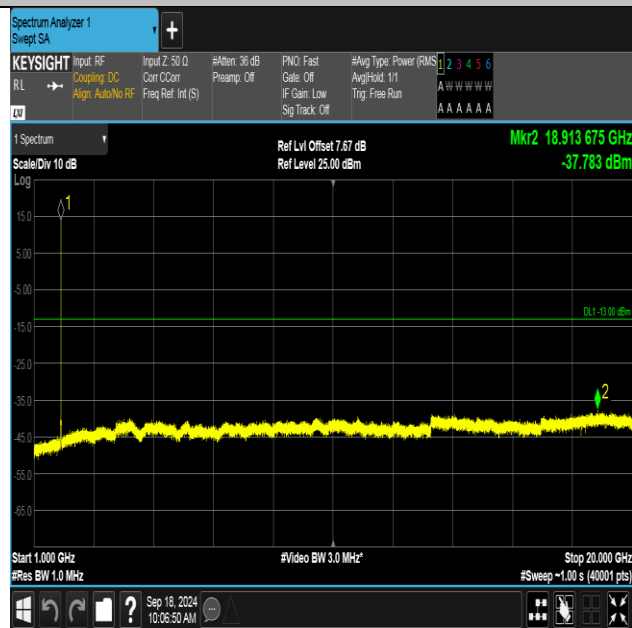
Band2-9262-4-1000~20000MHz-PASS
