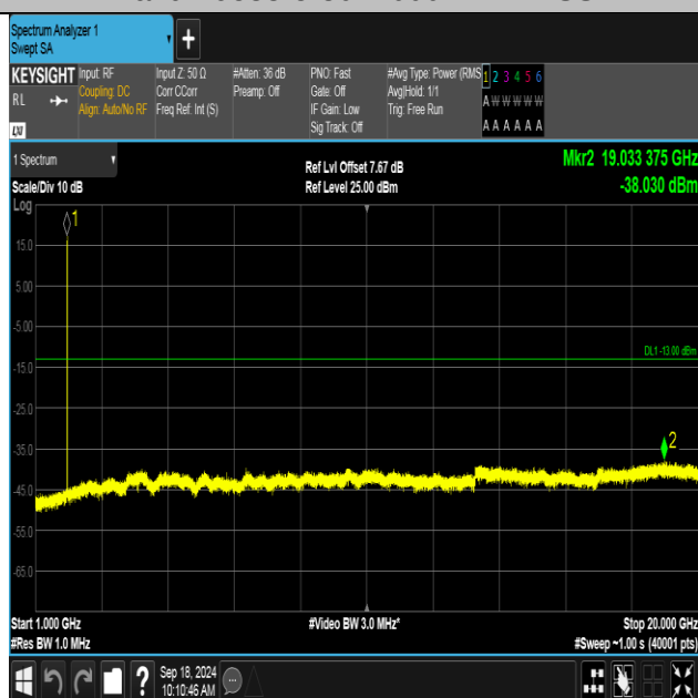
Band2-9538-5-1000~20000MHz-PASS
