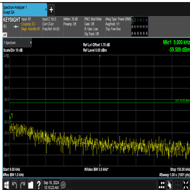
Band2-9538-5-0.009~0.15MHz-PASS
