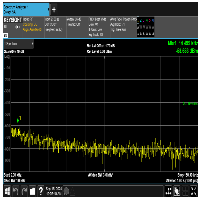
Band2-9400-4-0.009~0.15MHz-PASS
