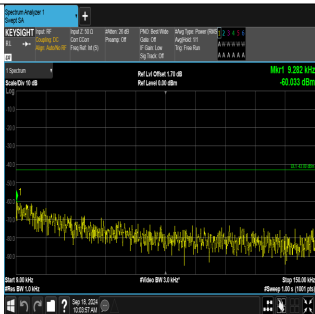
Band2-9262-3-0.009~0.15MHz-PASS
