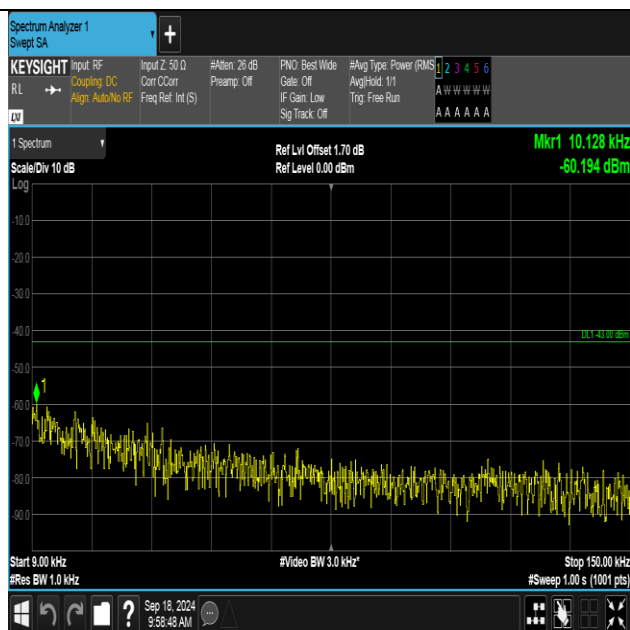
Band2-9262-1-0.009~0.15MHz-PASS
