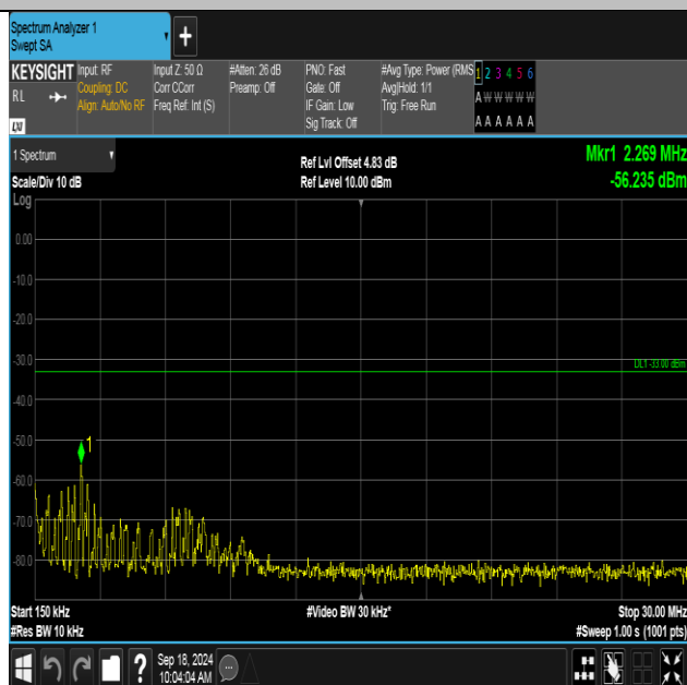
Band2-9262-3-0.15~30MHz-PASS
