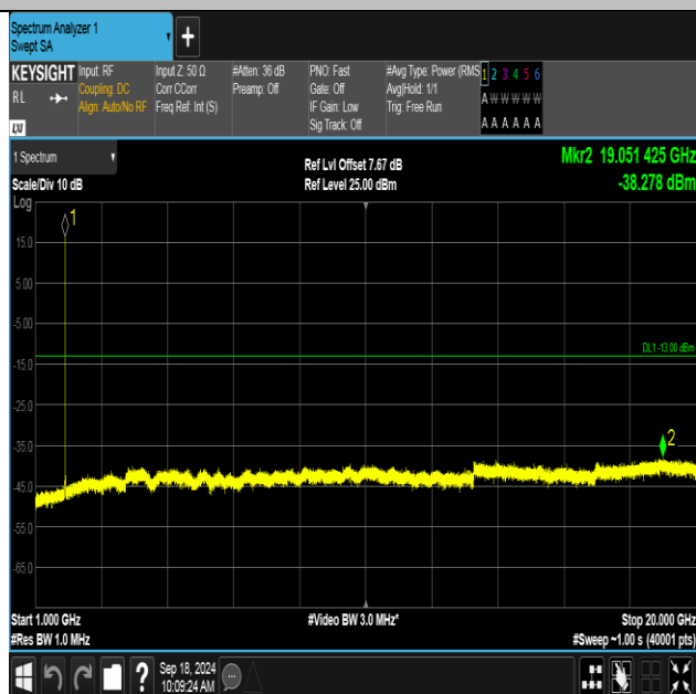
Band2-9262-5-1000~20000MHz-PASS
