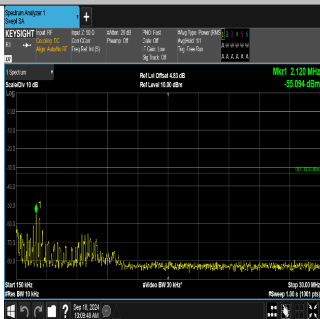
Band2-9400-5-0.15~30MHz-PASS
