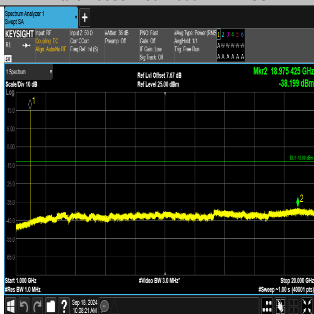
Band2-9538-4-1000~20000MHz-PASS
