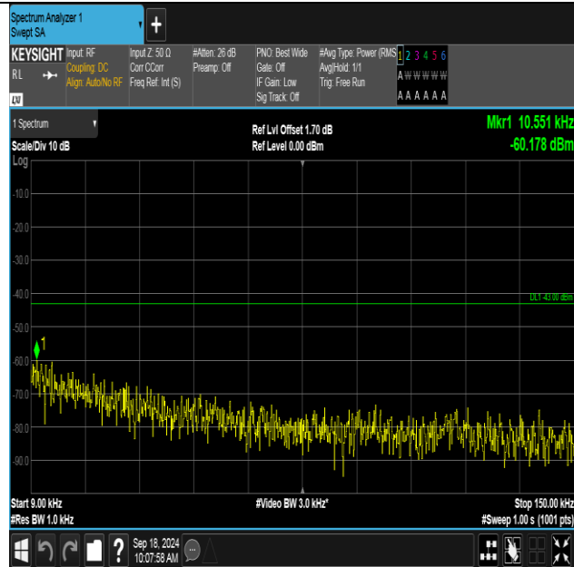
Band2-9538-4-0.009~0.15MHz-PASS
