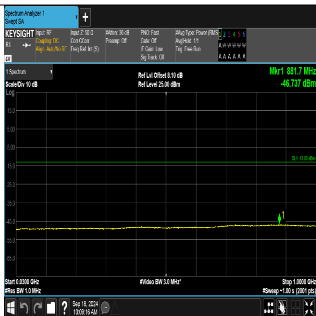
Band2-9262-5-30~1000MHz-PASS
