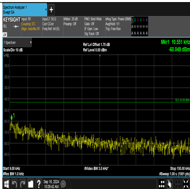
Band2-9400-5-0.009~0.15MHz-PASS
