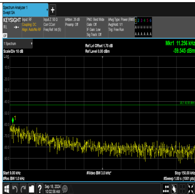
Band2-9538-2-0.009~0.15MHz-PASS
