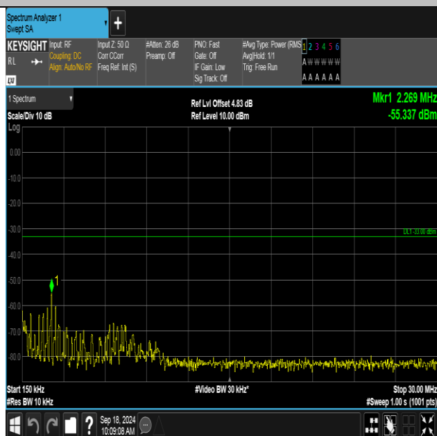
Band2-9262-5-0.15~30MHz-PASS
