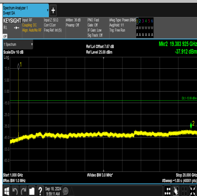
Band2-9262-1-1000~20000MHz-PASS
