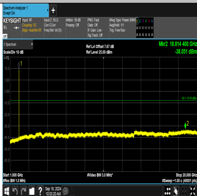
Band2-9538-2-1000~20000MHz-PASS
