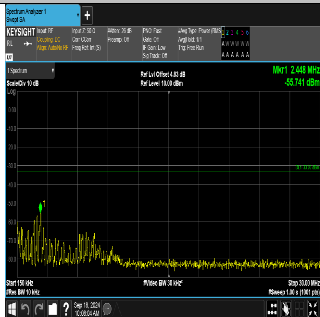
Band2-9538-4-0.15~30MHz-PASS
