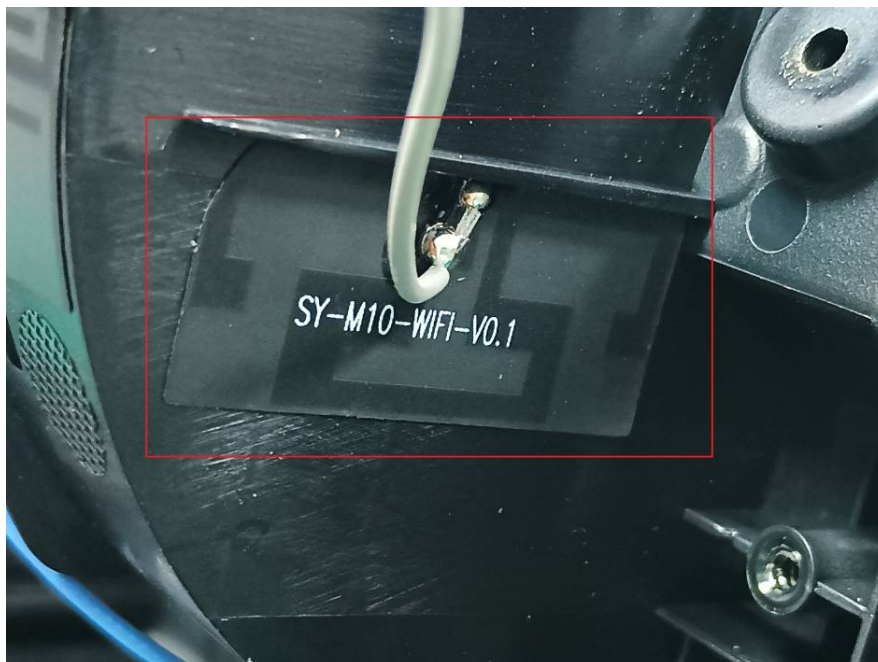
BT&BLE&Wi-Fi Antenna
