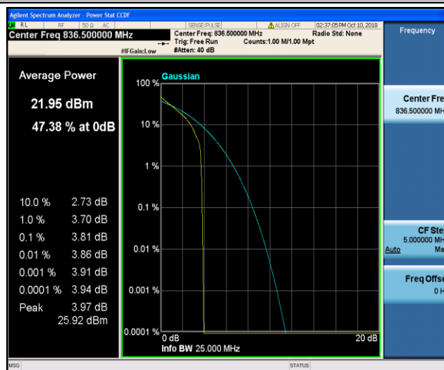
Band26_3MHz_QPSK_20525_1RB#0
