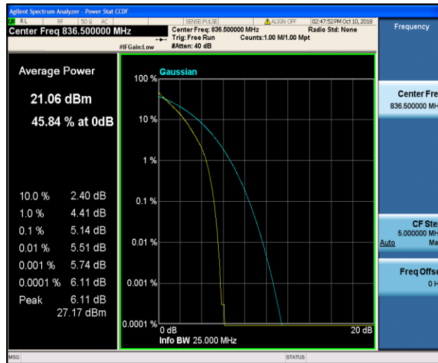
Band26_5MHz_QPSK_20525_25RB#0
