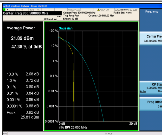
Band26_1.4MHz_QPSK_20525_1RB#0
