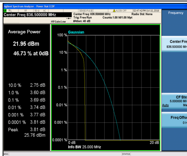
Band26_5MHz_QPSK_20525_1RB#0
