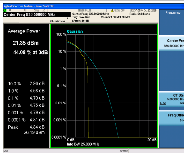
Band26_3MHz_16QAM_20525_1RB#0
