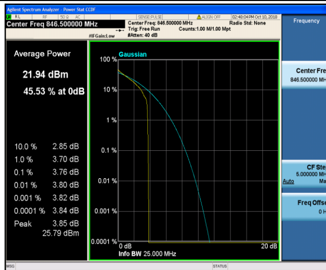
Band26_5MHz_QPSK_20625_1RB#0
