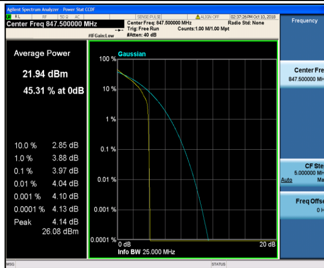
Band26_3MHz_QPSK_20635_1RB#0
