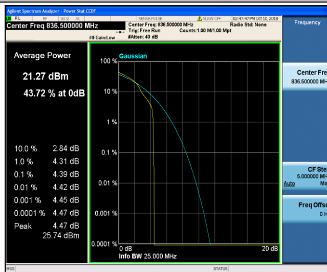
Band26_5MHz_16QAM_20525_1RB#0
