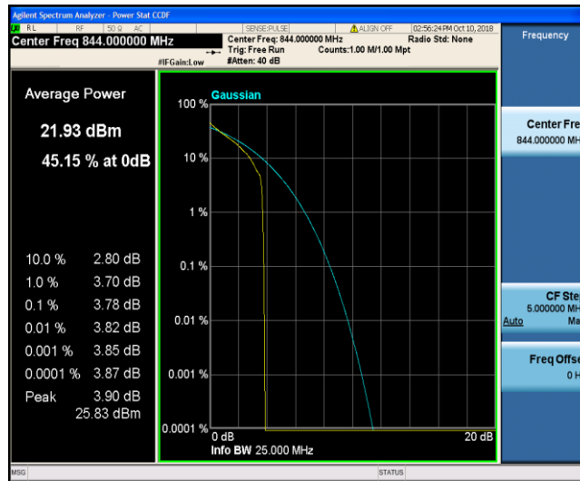
Band26_10MHz_QPSK_20600_1RB#0
