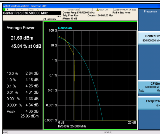
Band26_10MHz_16QAM_20525_1RB#0
