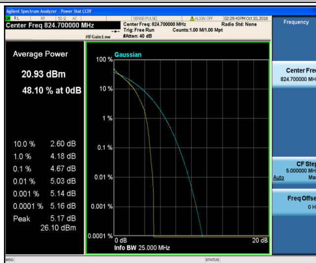
Band26_1.4MHz_QPSK_20407_6RB#0
