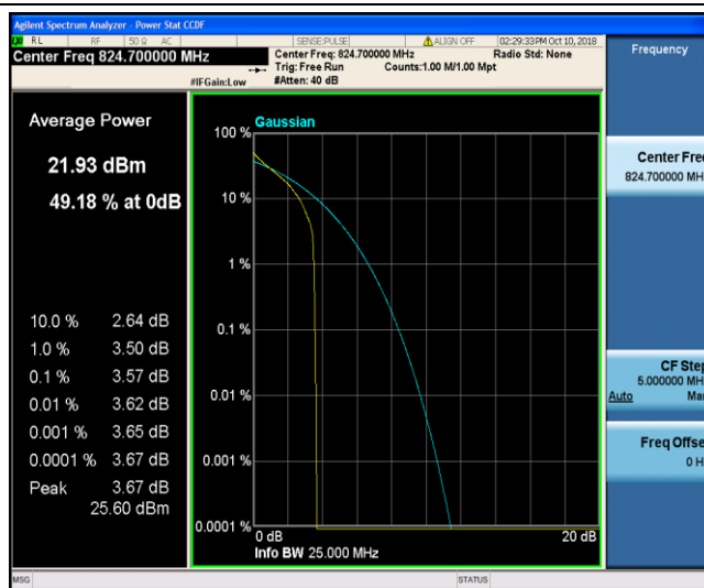
Band26_1.4MHz_QPSK_20407_1RB#0
