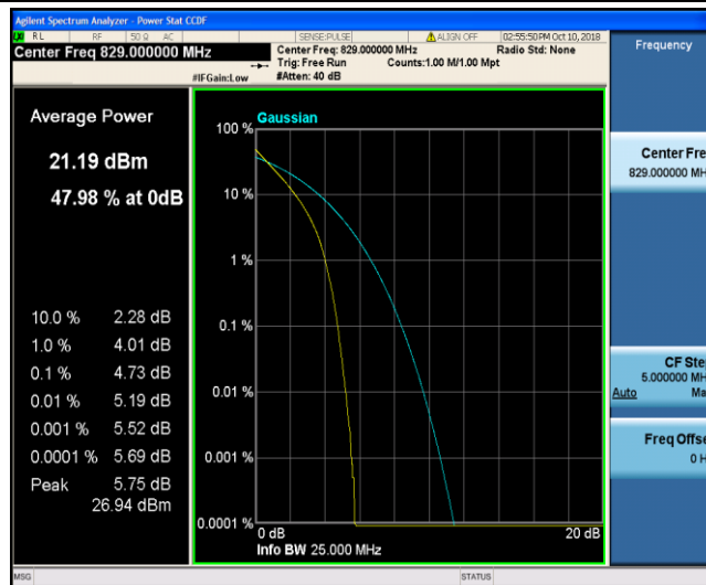
Band26_10MHz_QPSK_20450_50RB#0
