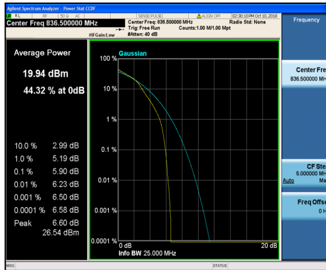
Band26_1.4MHz_16QAM_20525_6RB#0
