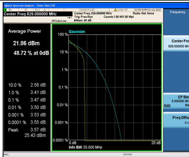
Band26_10MHz_QPSK_20450_1RB#0
