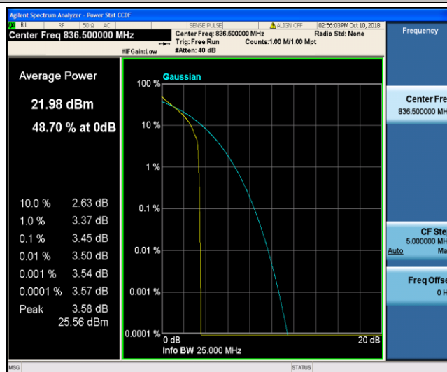
Band26_10MHz_QPSK_20525_1RB#0
