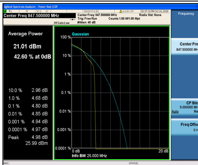
Band26_3MHz_16QAM_20635_1RB#0
