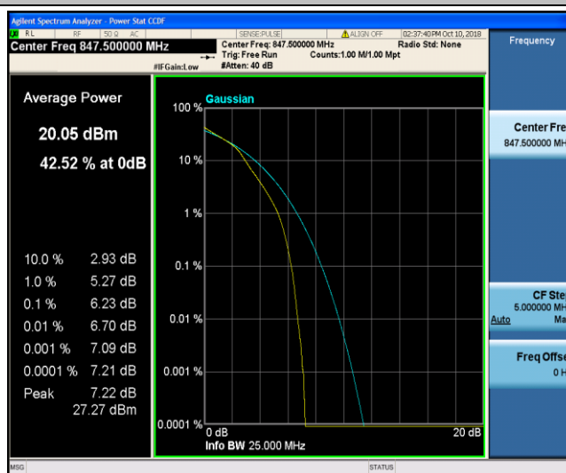
Band26_3MHz_16QAM_20635_15RB#0
