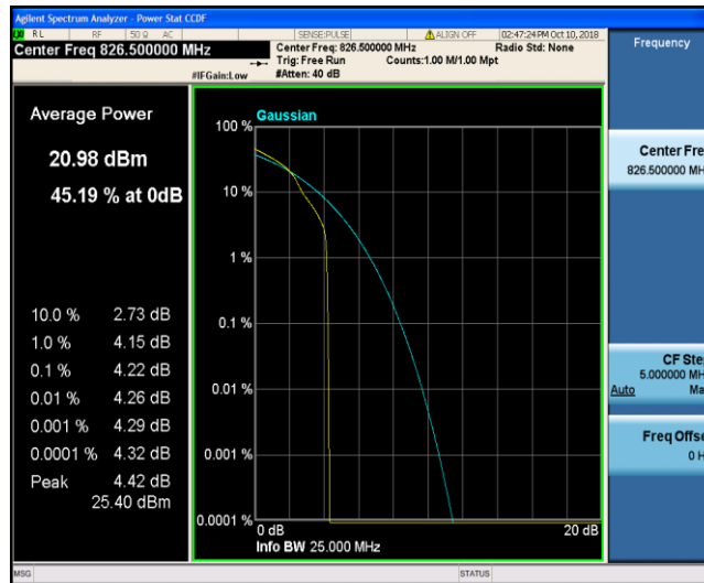
Band26_5MHz_16QAM_20425_1RB#0
