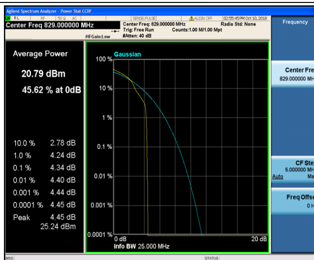
Band26_10MHz_16QAM_20450_1RB#0
