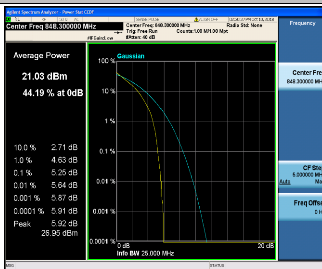
Band26_1.4MHz_QPSK_20643_6RB#0
