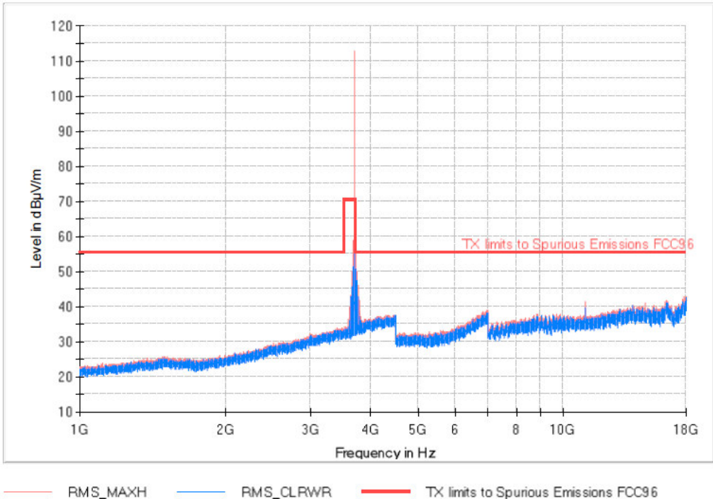
Band 48_BW5M_High Channel FREQUENCY RANGE 1-18 GHz
