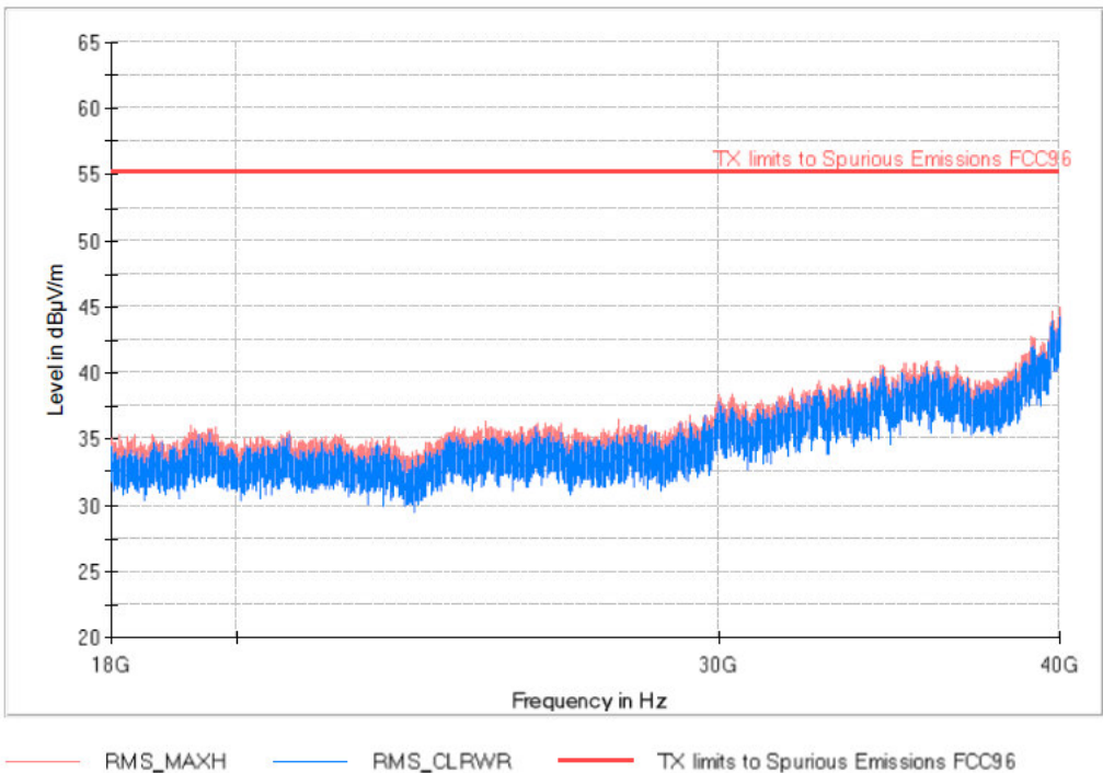
Band 43_BW10M_High Channel FREQUENCY RANGE 18-40 GHz
