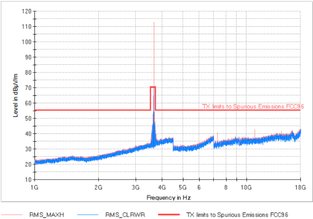
Band 43_BW5M_Middle Channel FREQUENCY RANGE 1-18 GHz
