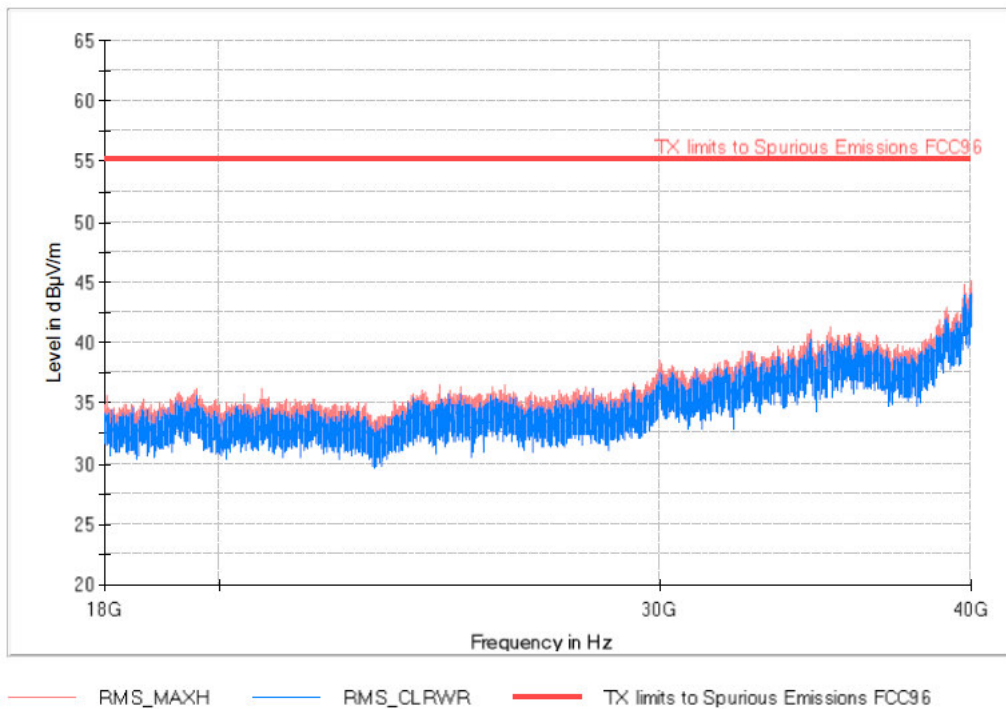
Band 42_BW10M_Middle Channel FREQUENCY RANGE 18-40 GHz
