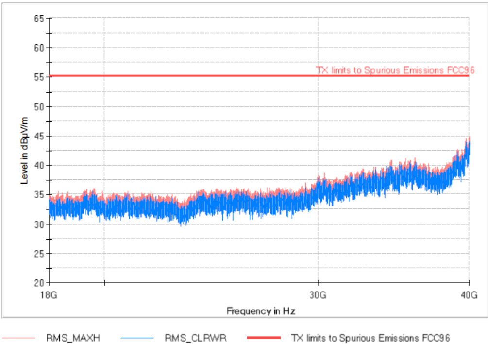
Band 48_BW5M_Low Channel FREQUENCY RANGE 18-40 GHz
