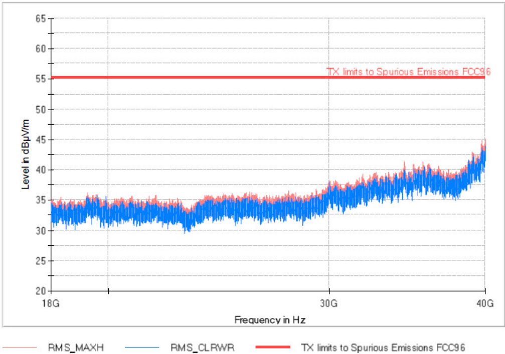
Band 48_BW15M_Low Channel FREQUENCY RANGE 18-40 GHz
