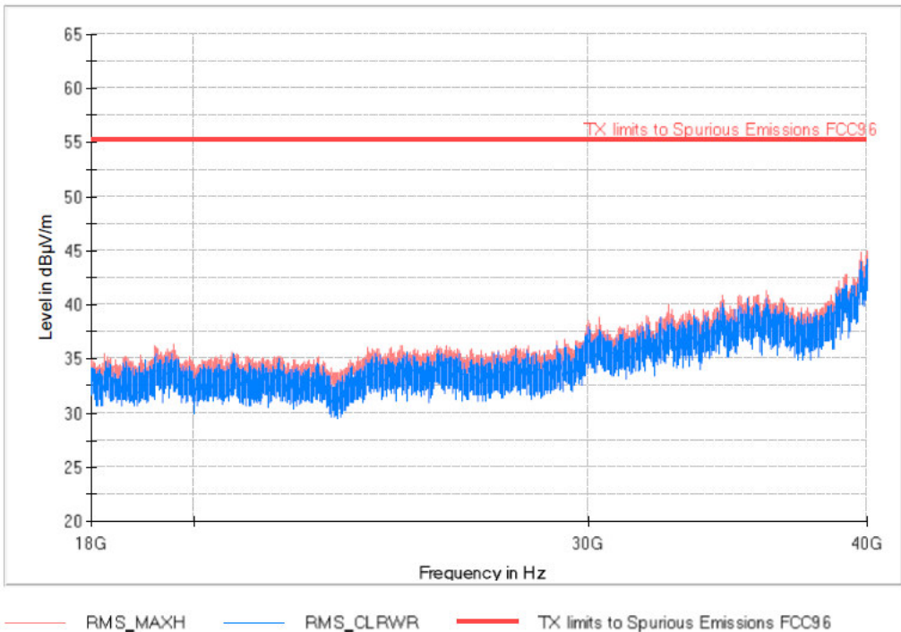
Band 43_BW10M_Middle Channel FREQUENCY RANGE 18-40 GHz
