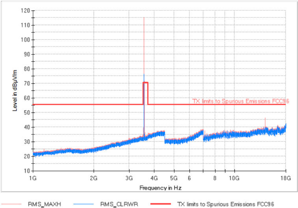
Band 42_BW15M_Low Channel FREQUENCY RANGE 1-18 GHz
