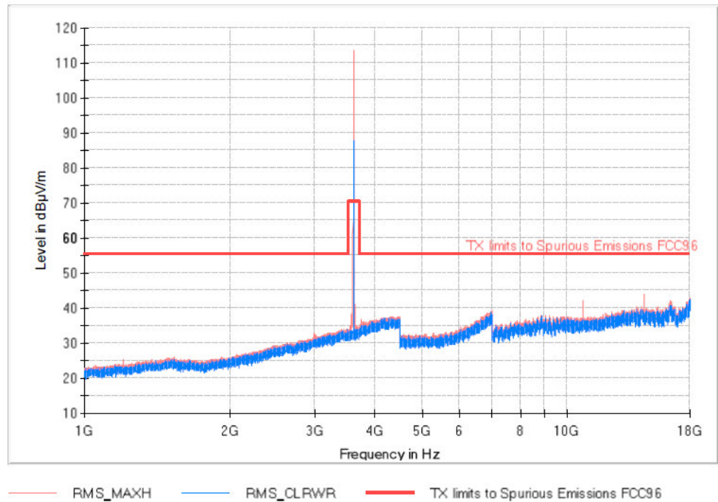
Band 43_BW10M_Low Channel FREQUENCY RANGE 1-18 GHz
