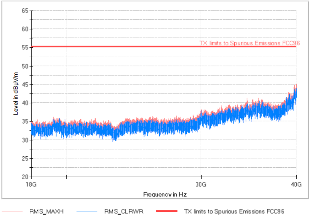
Band 42_BW15M_Low Channel FREQUENCY RANGE 18-40 GHz
