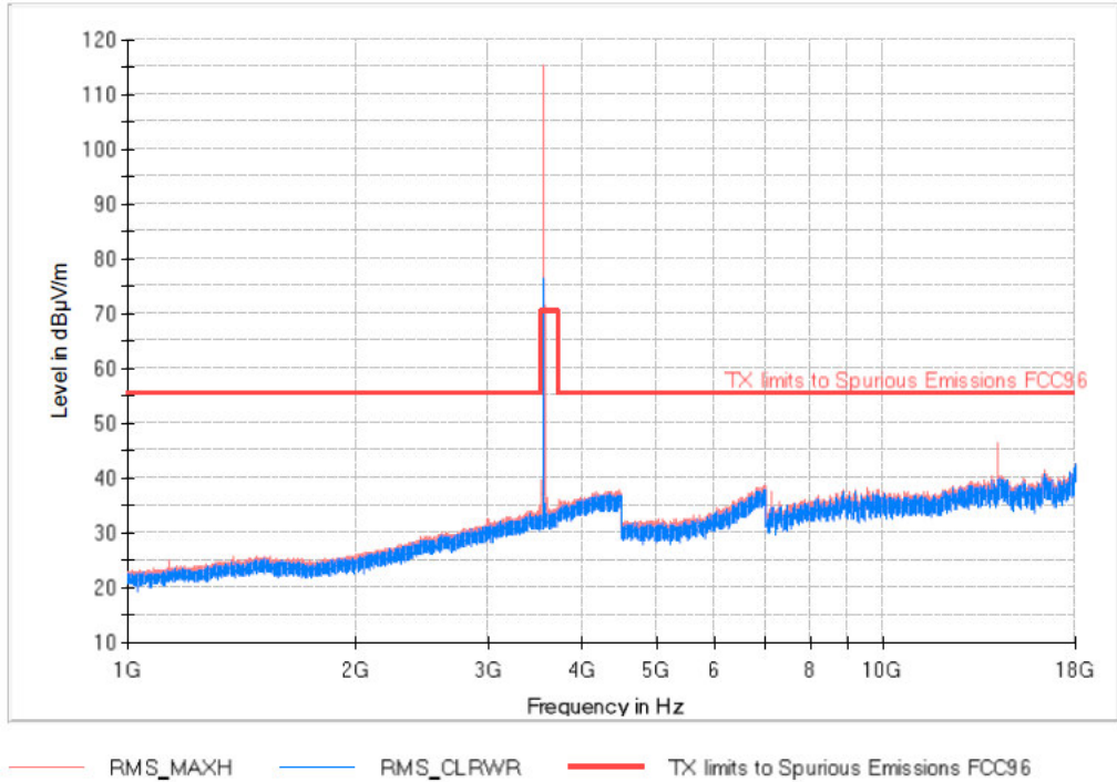
Band 48_BW15M_Low Channel FREQUENCY RANGE 1-18 GHz
