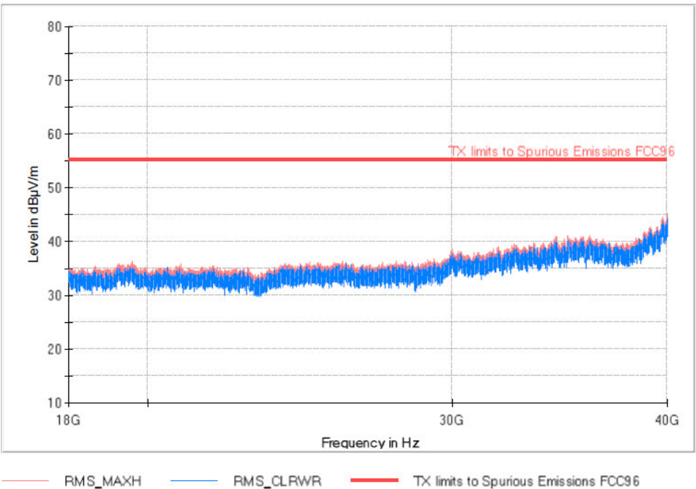
Band 42_BW5M_High Channel FREQUENCY RANGE 18-40 GHz
