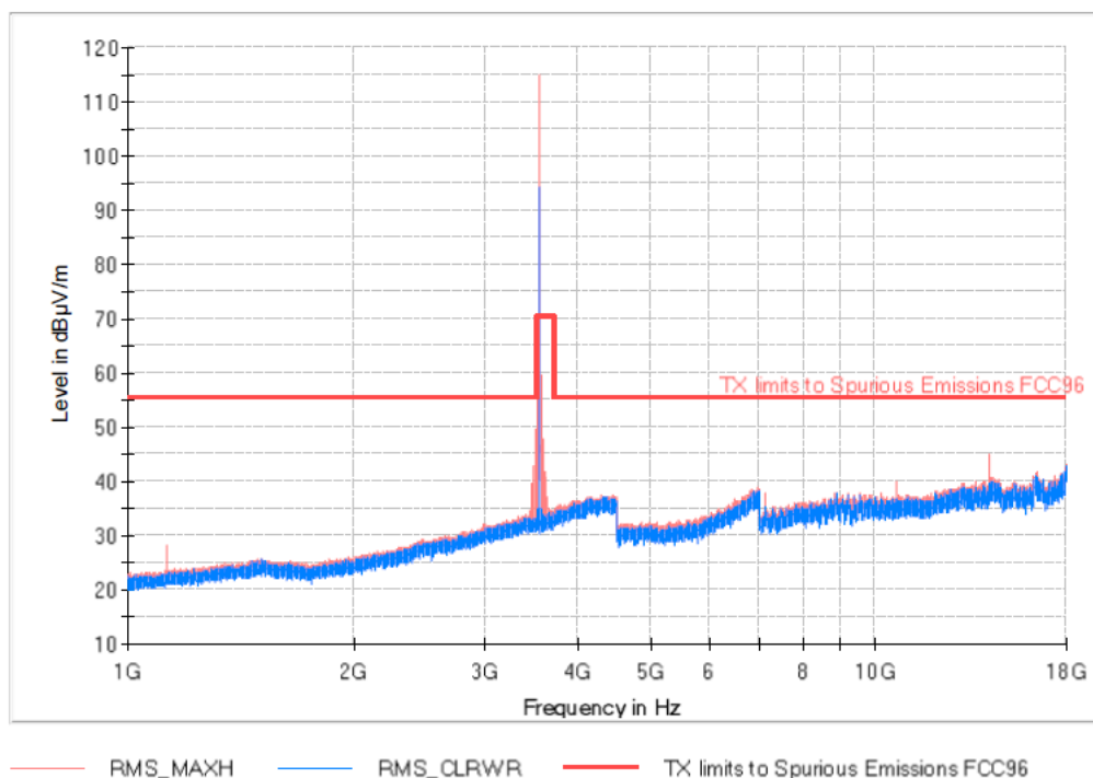
Band 42_BW5M_Low Channel FREQUENCY RANGE 1-18 GHz
