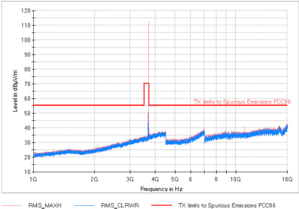
Band 48_BW10M_High Channel FREQUENCY RANGE 1-18 GHz
