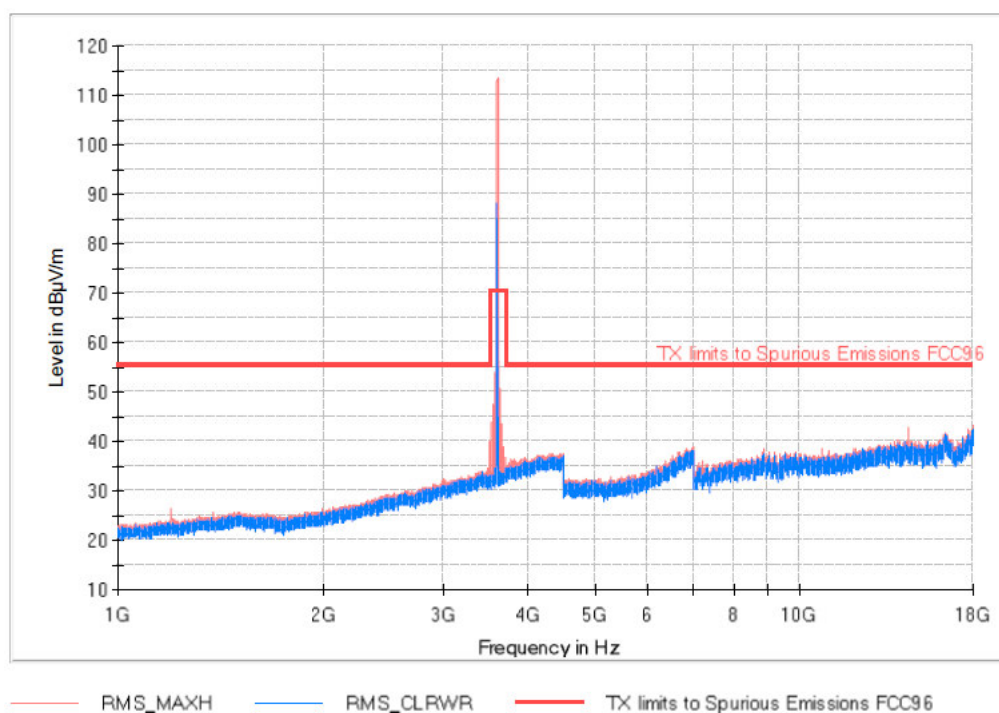
Band 43_BW5M_Low Channel FREQUENCY RANGE 1-18 GHz
