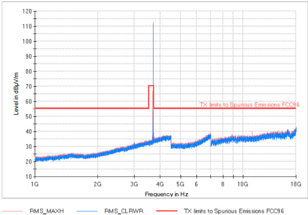
Band 48_BW15M_High Channel FREQUENCY RANGE 1-18 GHz
