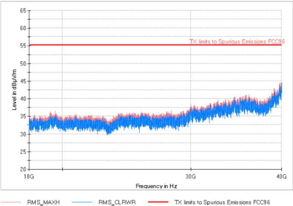
Band 48_BW10M_Low Channel FREQUENCY RANGE 18-40 GHz
