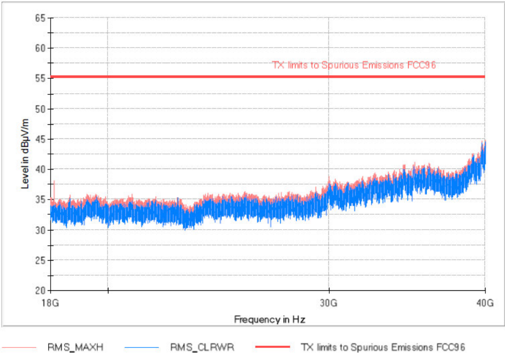
Band 48_BW5M_Middle Channel FREQUENCY RANGE 18-40 GHz
