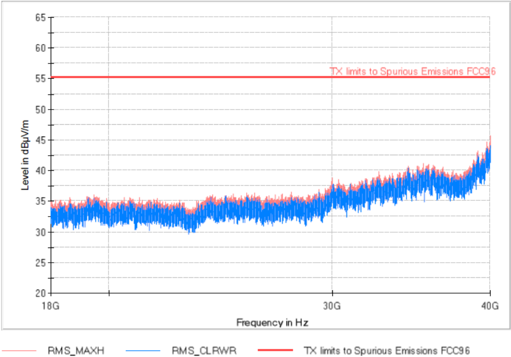
Band 48_BW5M_High Channel FREQUENCY RANGE 18-40 GHz
