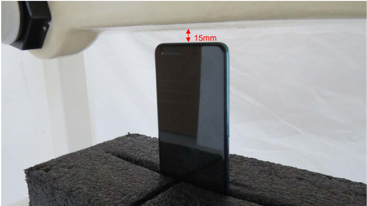
Picture 17: Top Side, the distance from handset to the bottom of the Phantom is 15mm
