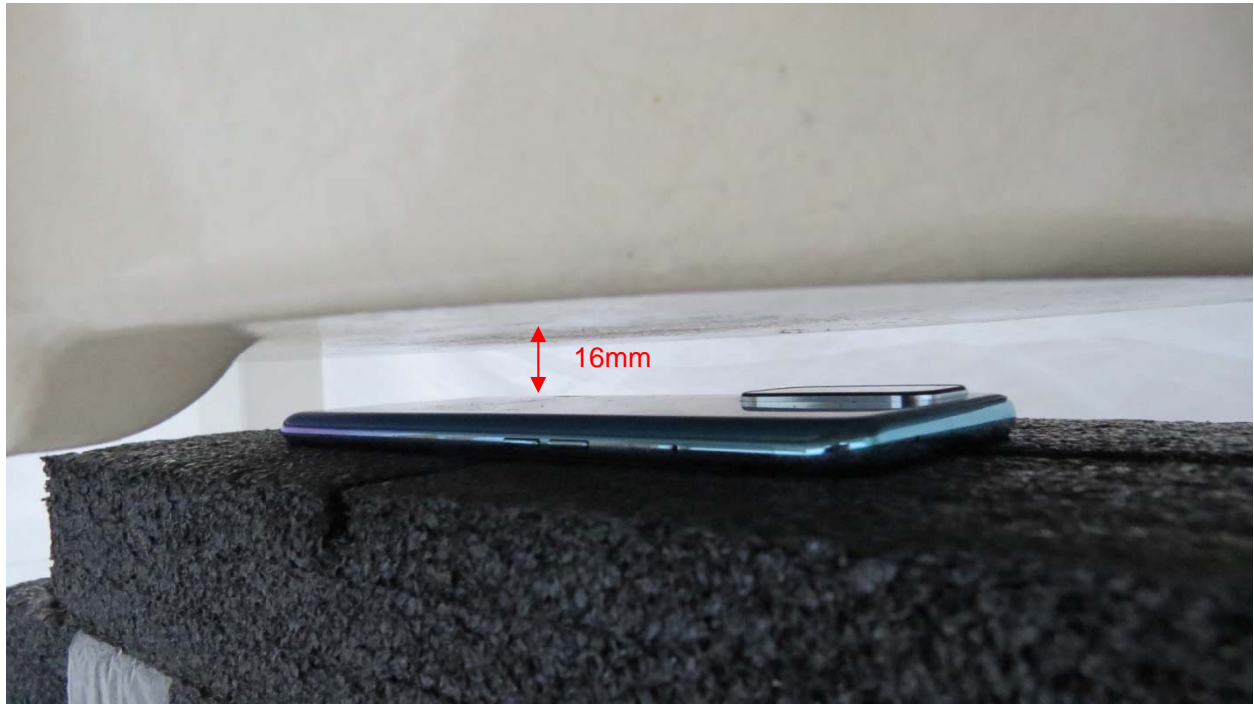
Picture 5: Back Side, the distance from handset to the bottom of the Phantom is 16mm
