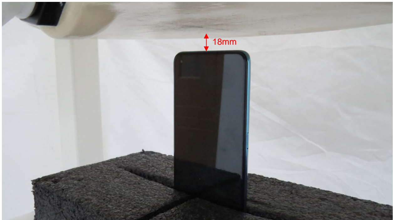
Picture 16: Top Side, the distance from handset to the bottom of the Phantom is 18mm
