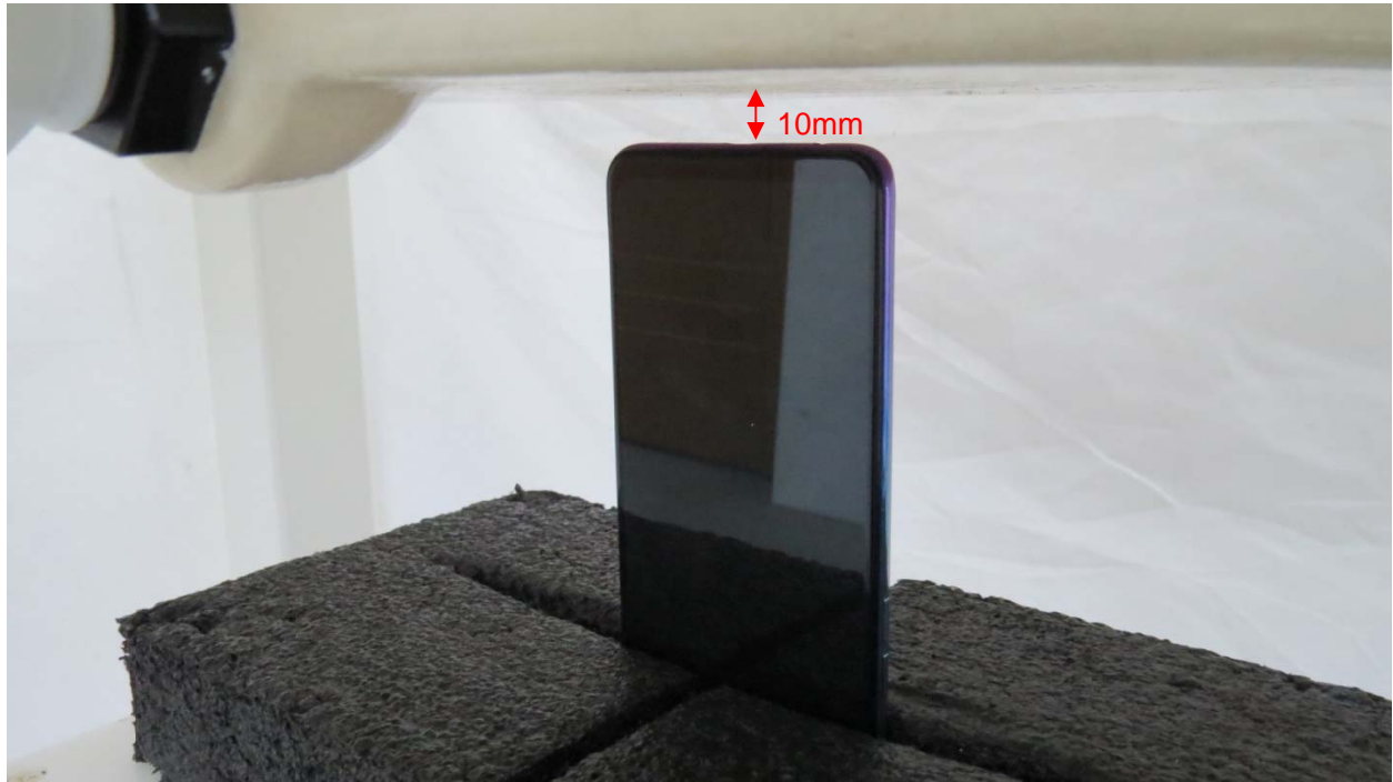
Picture 19: Bottom Edge, the distance from handset to the bottom of the Phantom is 10mm
