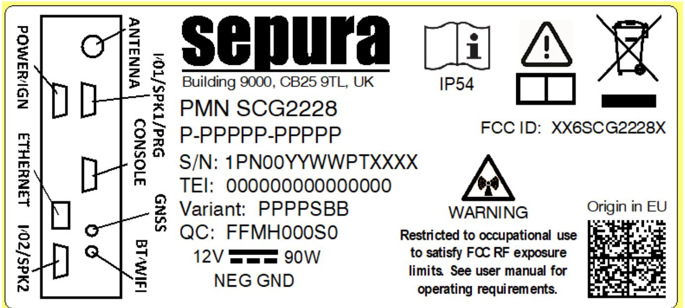
Figure 1. XX6SCG222xx sample label
