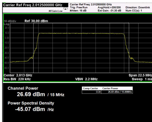
Channel: TOP, Modulation: 64QAM, BW=15MHz, Channel Power
