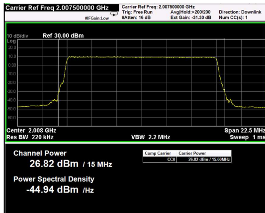
Channel: MIDDLE, Modulation: 64QAM, BW=15MHz, Channel Power
