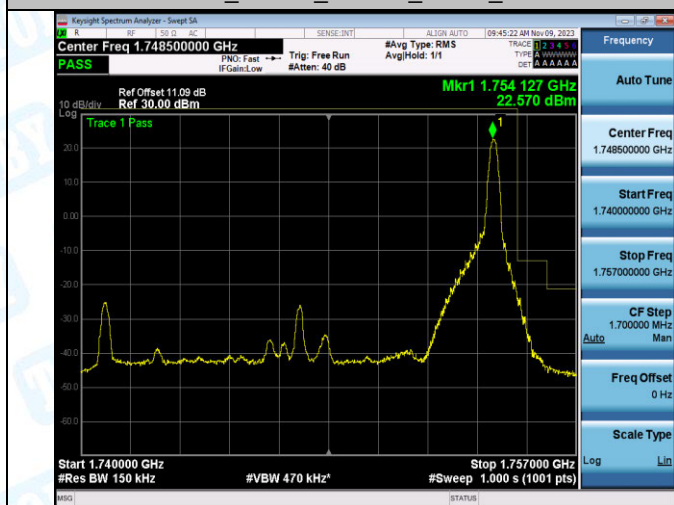
Band4_15MHz_16QAM_20325_1RB#74
