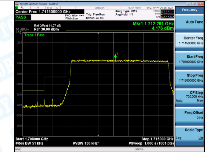
Band4_5MHz_16QAM_19975_25RB#0
