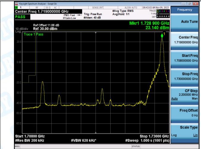
Band4_20MHz_16QAM_20050_1RB#99
