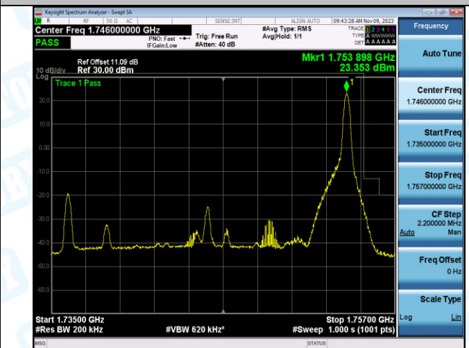
Band4_20MHz_16QAM_20300_1RB#99
