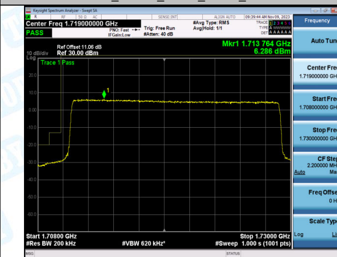
Band4_20MHz_QPSK_20050_100RB#0
