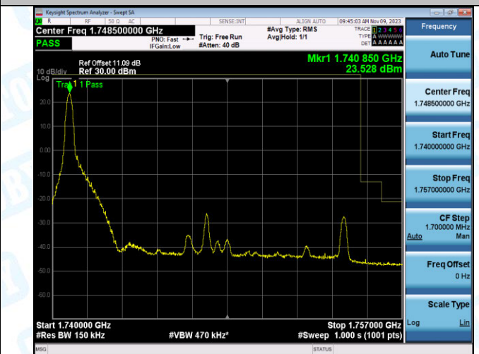
Band4_15MHz_QPSK_20325_1RB#0
