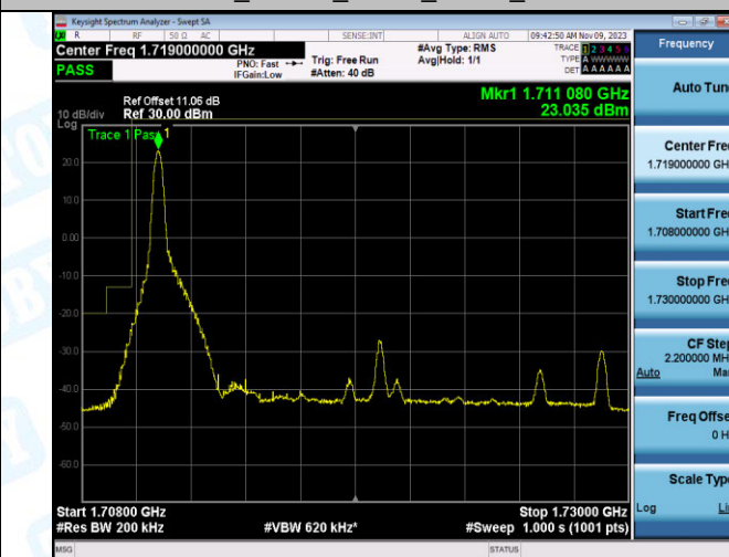
Band4_20MHz_16QAM_20050_1RB#0
