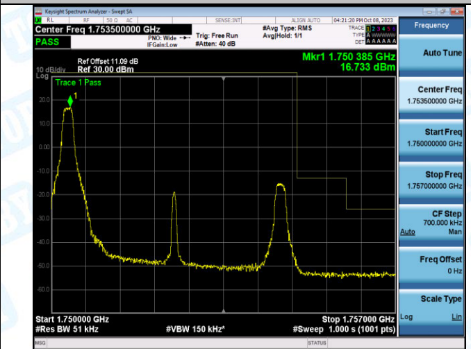
Band4_5MHz_16QAM_20375_1RB#0
