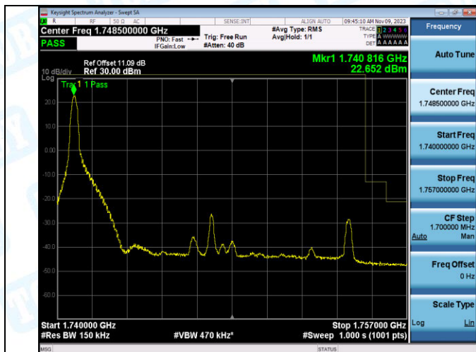
Band4_15MHz_16QAM_20325_1RB#0
