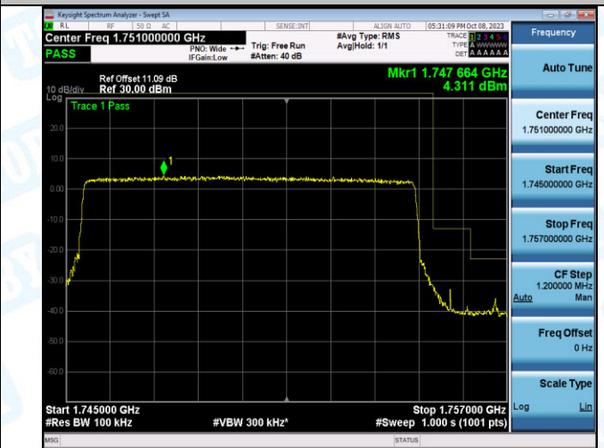
Band4_10MHz_QPSK_20350_50RB#0
