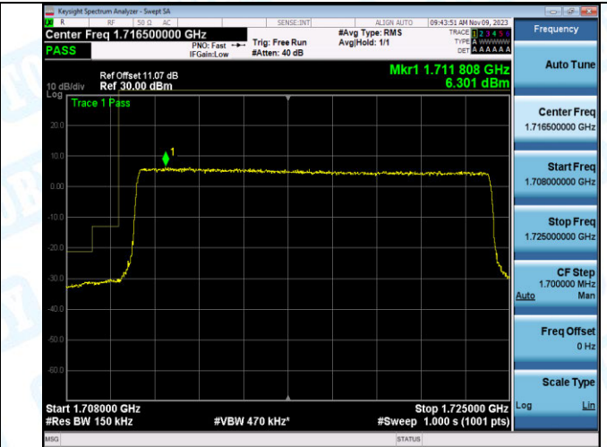
Band4_15MHz_QPSK_20025_75RB#0
