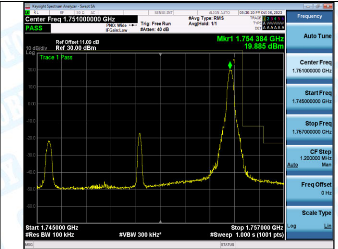
Band4_10MHz_16QAM_20350_1RB#49
