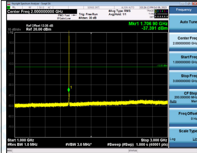
Band4_1.4MHz_16QAM_19957_1RB#0_1000~3000_1000
