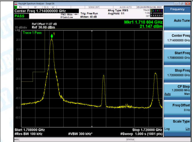
Band4_10MHz_16QAM_20000_1RB#0
