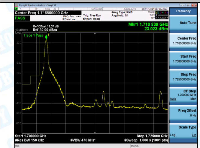
Band4_15MHz_16QAM_20025_1RB#0
