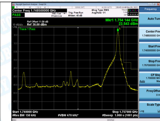
Band4_15MHz_QPSK_20325_1RB#74
