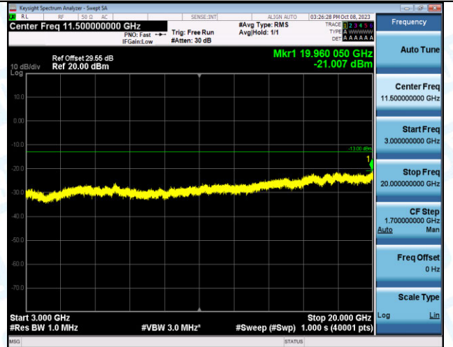
Band4_1.4MHz_16QAM_19957_1RB#0_3000~20000_3000
