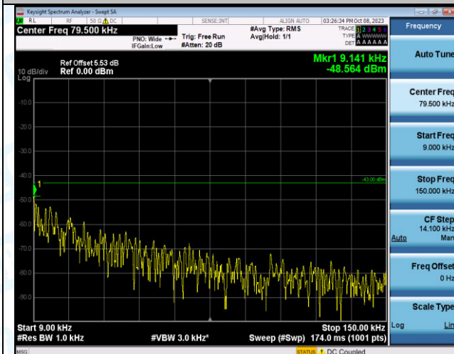
Band4_1.4MHz_QPSK_19957_6RB#0_0.009~0.15_0.009
