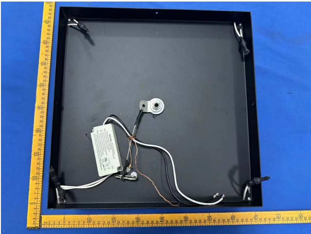
Fig.2(Model: FM-LU )
