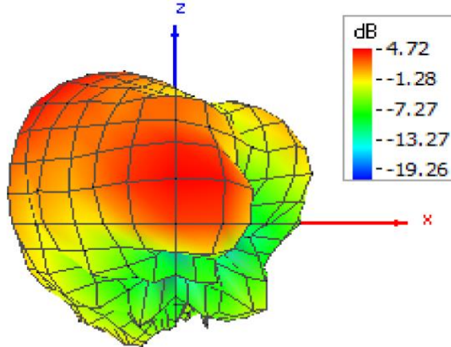
Figure A-8 Pattern at 5400 MHz
