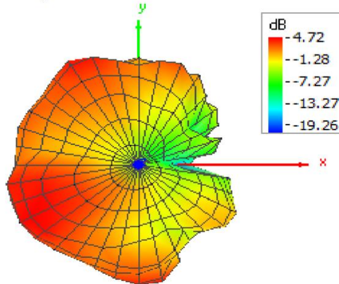
Figure A-6 Pattern at 5400 MHz
