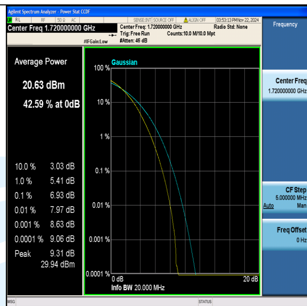
Band4-20MHz-64QAM-20050-100RB#0-PASS
