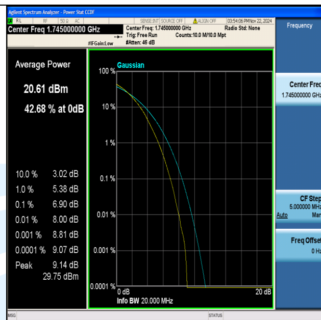
Band4-20MHz-64QAM-20300-100RB#0-PASS
