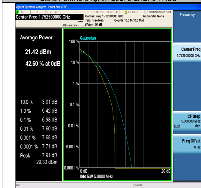
Band4-5MHz-64QAM-20375-1RB#0-PASS
