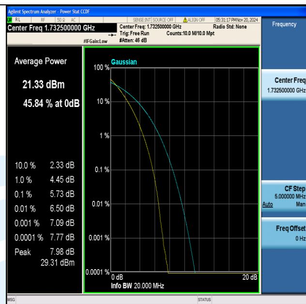
Band4-20MHz-QPSK-20175-100RB#0-PASS
