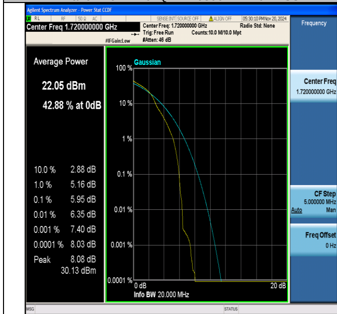
Band4-20MHz-16QAM-20050-1RB#0-PASS
