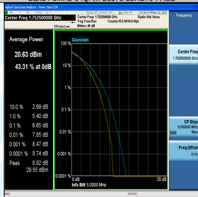
Band4-5MHz-64QAM-20375-25RB#0-PASS
