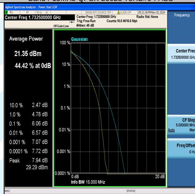
Band4-15MHz-QPSK-20175-75RB#0-PASS
