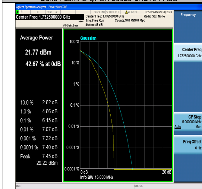
Band4-15MHz-QPSK-20175-1RB#0-PASS
