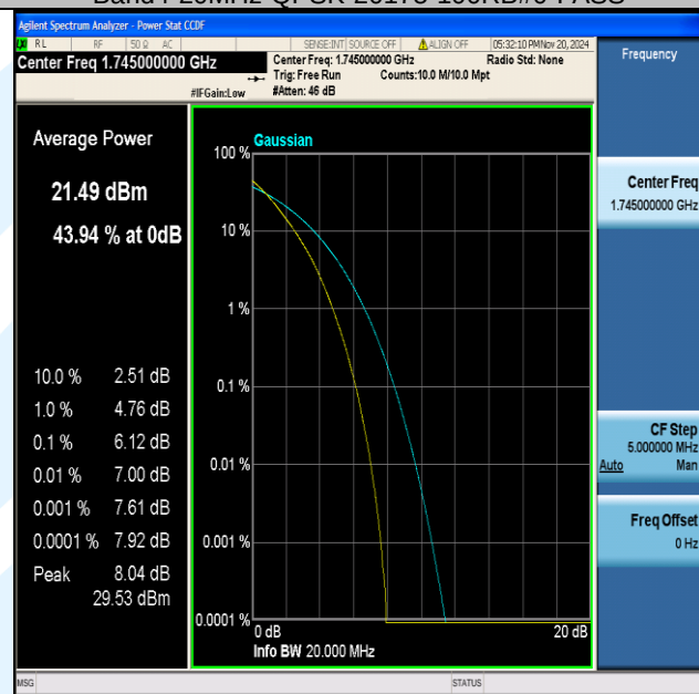
Band4-20MHz-QPSK-20300-100RB#0-PASS
