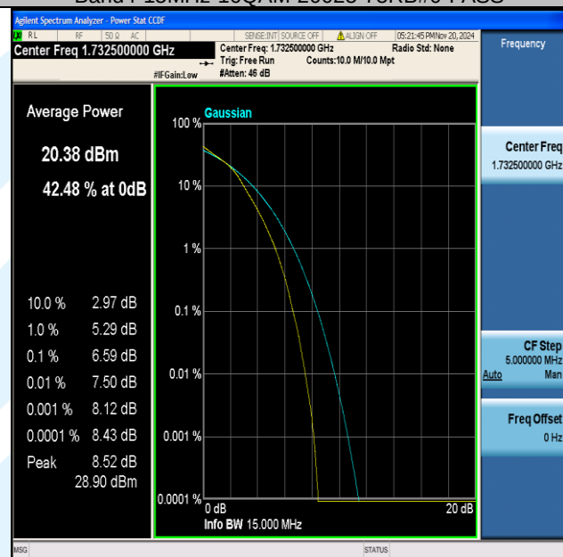
Band4-15MHz-16QAM-20175-75RB#0-PASS
