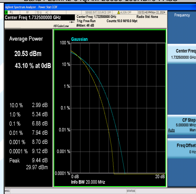
Band4-20MHz-64QAM-20175-100RB#0-PASS
