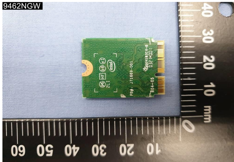
EUT Photo (1)
