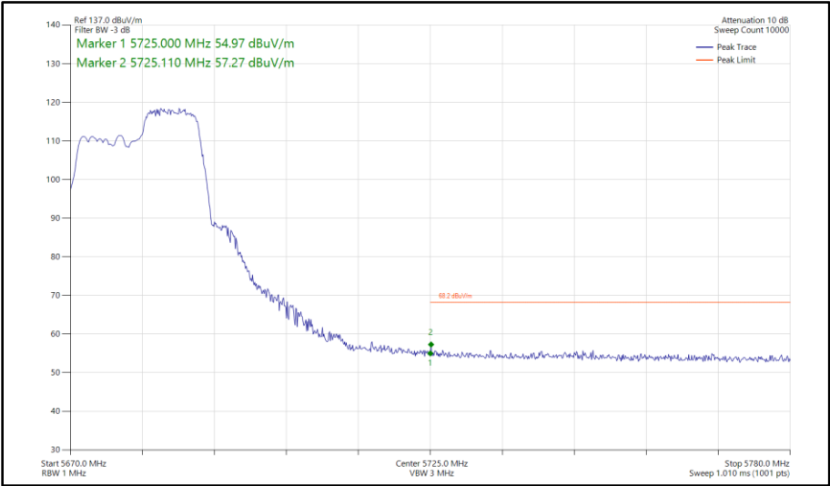
Figure 368 - 802.11ax HE20, RU 106-54, SISO, Core 0 - 5680 MHz Band Edge Frequency 5725 MHz
