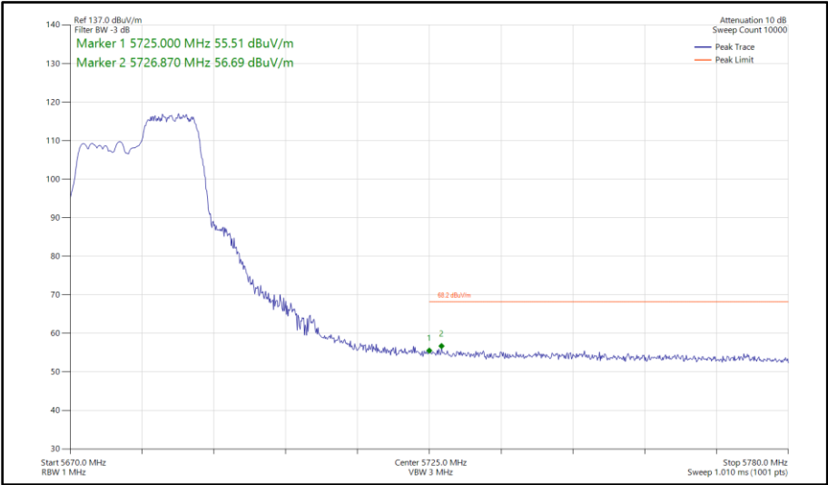
Figure 402 - 802.11ax HE20, RU 106-54, SISO, Core 1 - 5680 MHz Band Edge Frequency 5725 MHz
