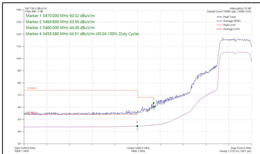
Figure 354 - 802.11ax HE20, SU, SISO, Core 0 - 5520 MHz Band Edge Frequency 5470 MHz
