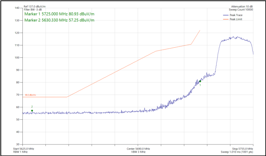
Figure 392 - 802.11n HT20, SISO, Core 1 - 5745 MHz Band Edge Frequency 5725 MHz
