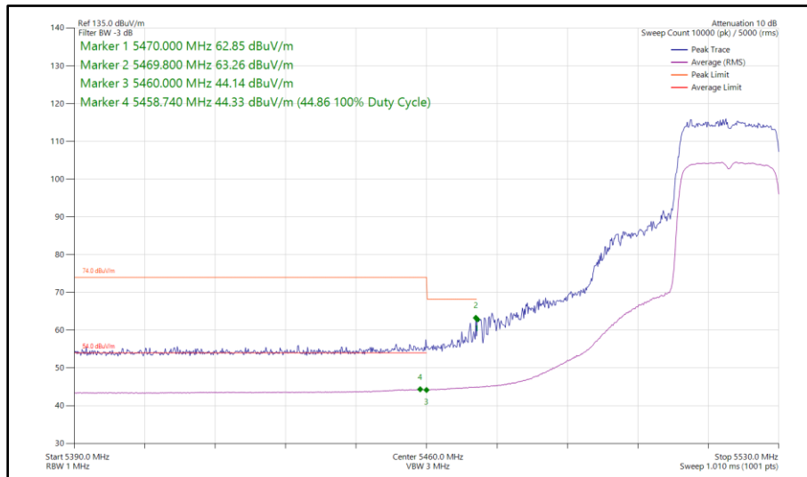
Figure 388 - 802.11ax HE20, SU, SISO, Core 1 - 5520 MHz Band Edge Frequency 5470 MHz
