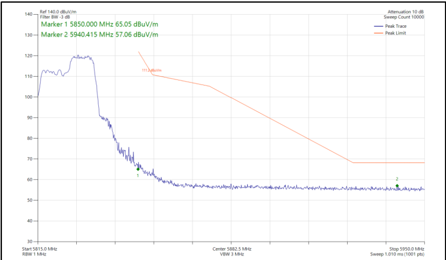
Figure 381 - 802.11ax HE20, RU 106-54, SISO, Core 0 - 5825 MHz Band Edge Frequency 5850 MHz
