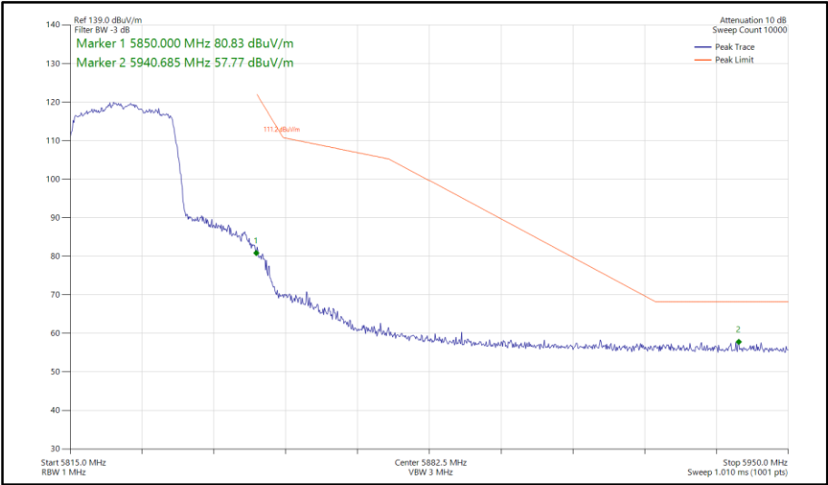
Figure 380 - 802.11ax HE20, SU, SISO, Core 0 - 5825 MHz Band Edge Frequency 5850 MHz
