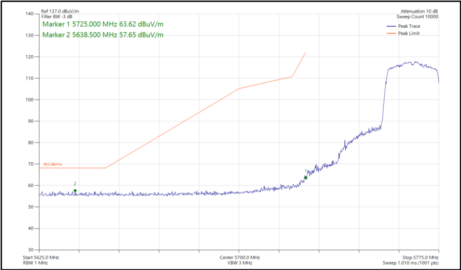
Figure 362 - 802.11ax HE20, SU, SISO, Core 0 - 5765 MHz Band Edge Frequency 5725 MHz
