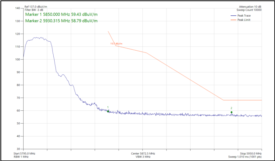
Figure 406 - 802.11a, SISO, Core 1 - 5805 MHz Band Edge Frequency 5850 MHz
