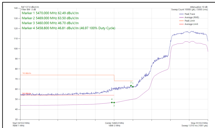
Figure 352 - 802.11ax HE20, SU, SISO, Core 0 - 5500 MHz Band Edge Frequency 5470 MHz
