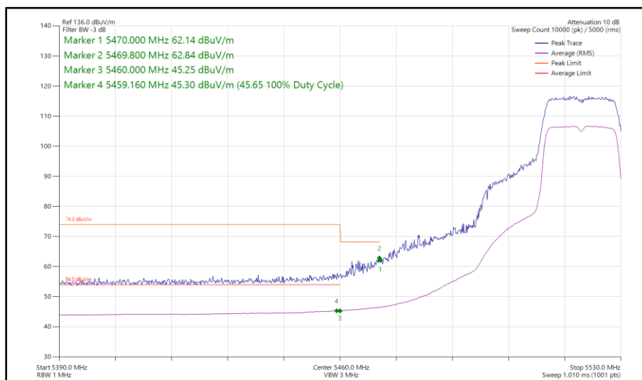
Figure 351 - 802.11n HT20, SISO, Core 0 - 5520 MHz Band Edge Frequency 5470 MHz
