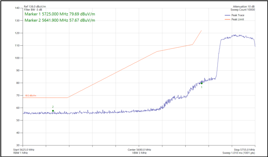
Figure 394 - 802.11ax HE20, SU, SISO, Core 1 - 5745 MHz Band Edge Frequency 5725 MHz
