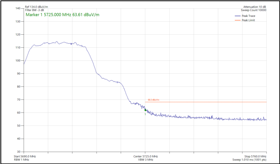
Figure 364 - 802.11a, SISO, Core 0 - 5700 MHz Band Edge Frequency 5725 MHz
