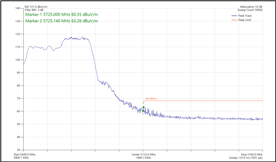
Figure 370 - 802.11ax HE20, RU 106-54, SISO, Core 0 - 5700 MHz Band Edge Frequency 5725 MHz
