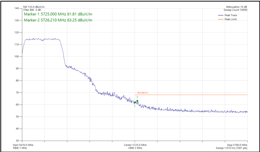
Figure 365 - 802.11n HT20, SISO, Core 0 - 5680 MHz Band Edge Frequency 5725 MHz
