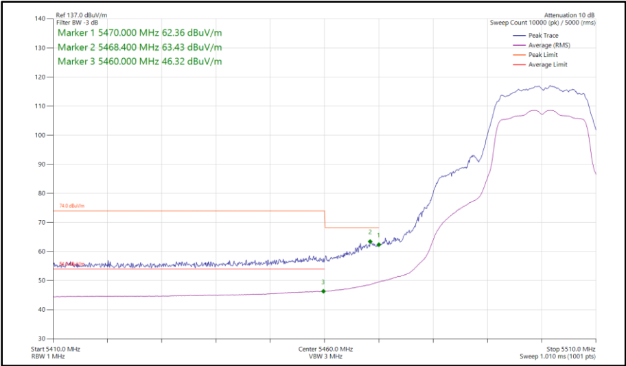
Figure 382 - 802.11a, SISO, Core 1 - 5500 MHz Band Edge Frequency 5470 MHz
