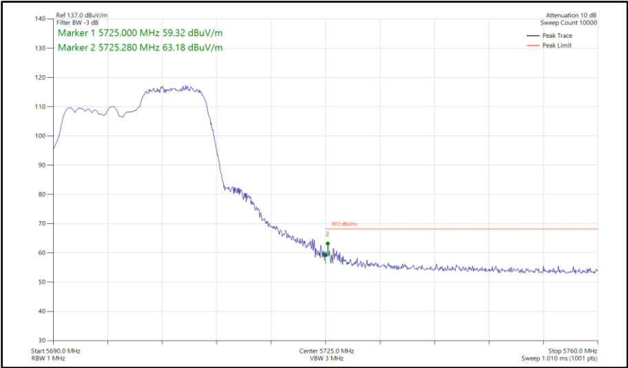
Figure 404 - 802.11ax HE20, RU 106-54, SISO, Core 1 - 5700 MHz Band Edge Frequency 5725 MHz
