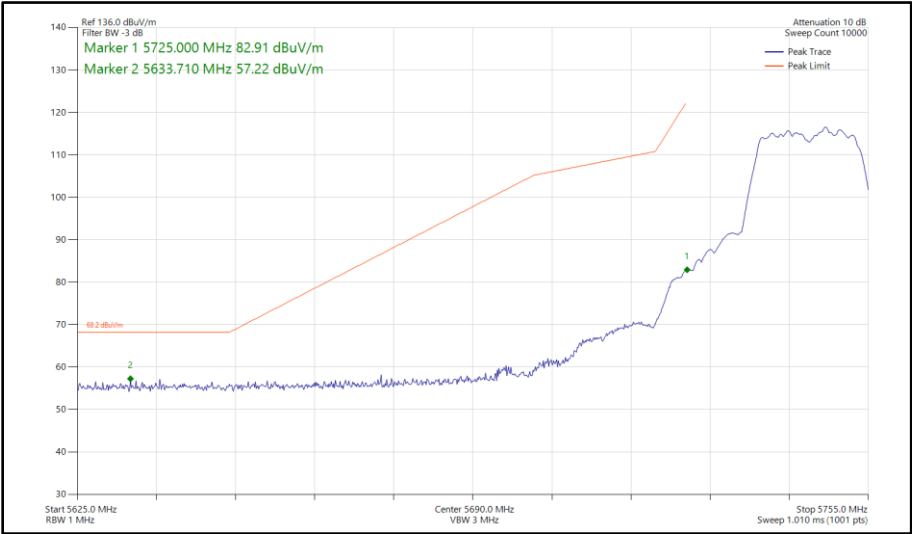
Figure 390 - 802.11a, SISO, Core 1 - 5745 MHz Band Edge Frequency 5725 MHz
