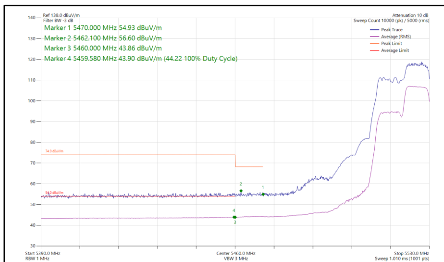
Figure 355 - 802.11ax HE20, RU 106-54, SISO, Core 0 - 5520 MHz Band Edge Frequency 5470 MHz
