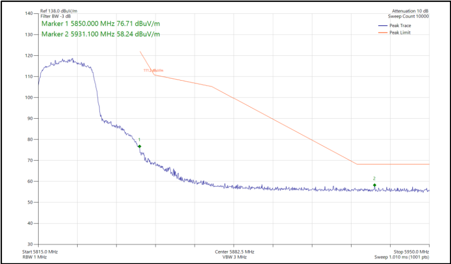
Figure 376 - 802.11n HT20, SISO, Core 0 - 5825 MHz Band Edge Frequency 5850 MHz
