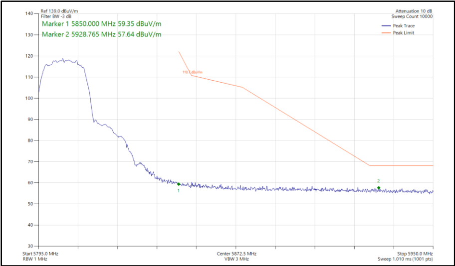
Figure 372 - 802.11a, SISO, Core 0 - 5805 MHz Band Edge Frequency 5850 MHz
