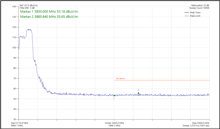
Figure 378 - 802.11ax HE20, RU 106-54, SISO, Core 0 - 5720 MHz Band Edge Frequency 5850 MHz
