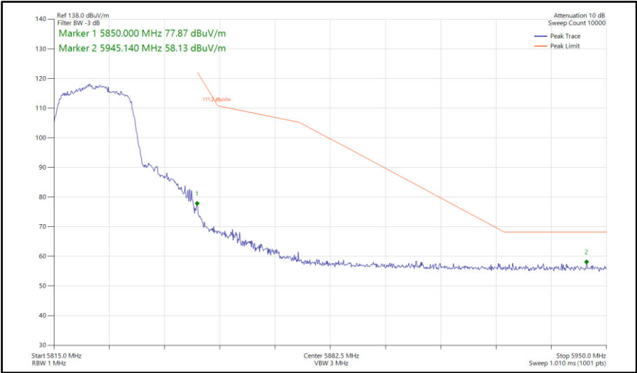
Figure 410 - 802.11n HT20, SISO, Core 1 - 5825 MHz Band Edge Frequency 5850 MHz
