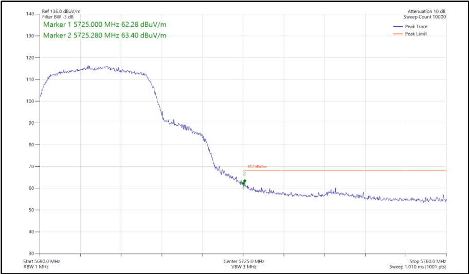
Figure 400 - 802.11n HT20, SISO, Core 1 - 5700 MHz Band Edge Frequency 5725 MHz
