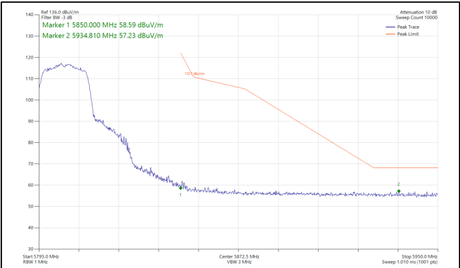
Figure 375 - 802.11n HT20, SISO, Core 0 - 5805 MHz Band Edge Frequency 5850 MHz
