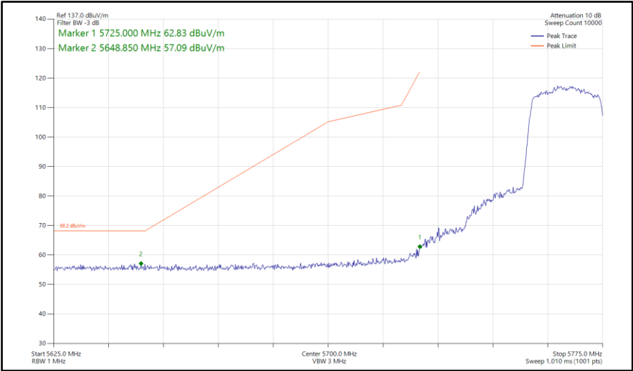
Figure 396 - 802.11ax HE20, SU, SISO, Core 1 - 5765 MHz Band Edge Frequency 5725 MHz
