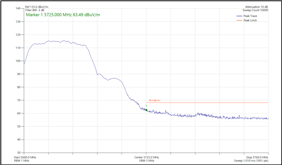
Figure 398 - 802.11a, SISO, Core 1 - 5700 MHz Band Edge Frequency 5725 MHz
