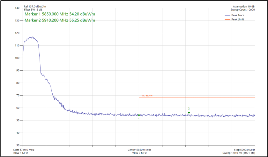
Figure 374 - 802.11n HT20, SISO, Core 0 - 5720 MHz Band Edge Frequency 5850 MHz
