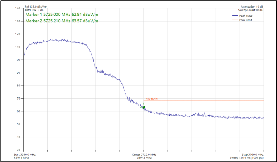
Figure 366 - 802.11n HT20, SISO, Core 0 - 5700 MHz Band Edge Frequency 5725 MHz
