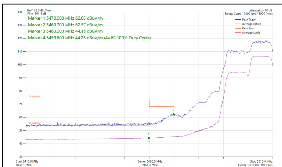
Figure 387 - 802.11ax HE20, RU 106-54, SISO, Core 1 - 5500 MHz Band Edge Frequency 5470 MHz
