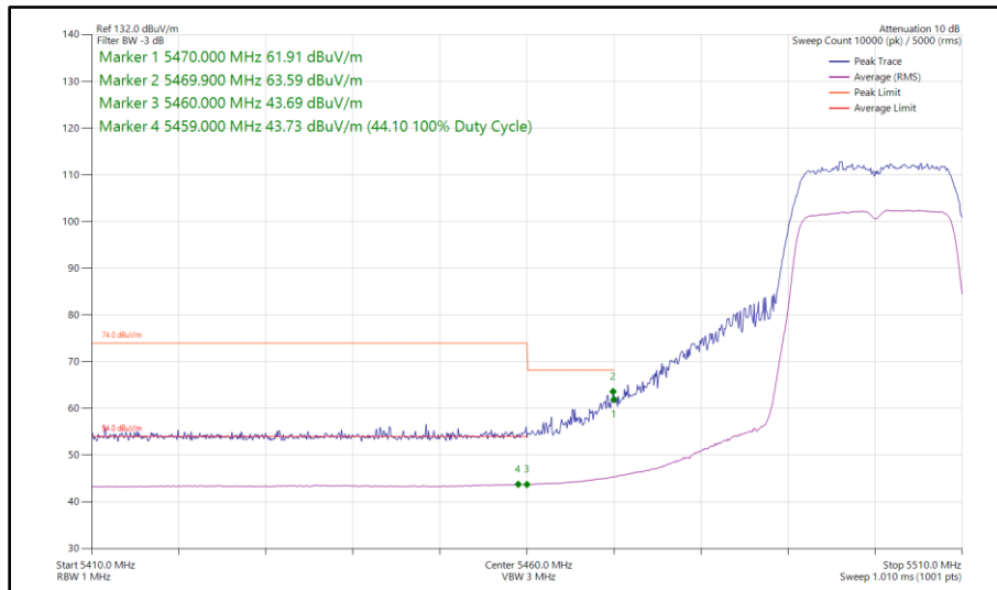
Figure 384 - 802.11n HT20, SISO, Core 1 - 5500 MHz Band Edge Frequency 5470 MHz
