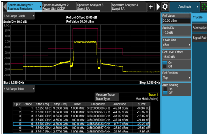
FULL (3555MHz)
