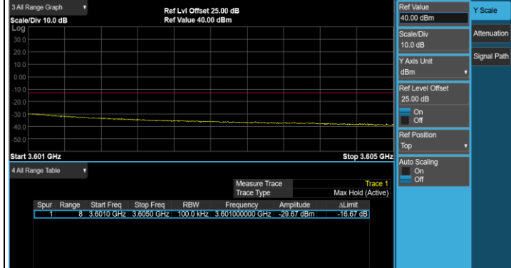
1RB#MAX (3597.5MHz)
