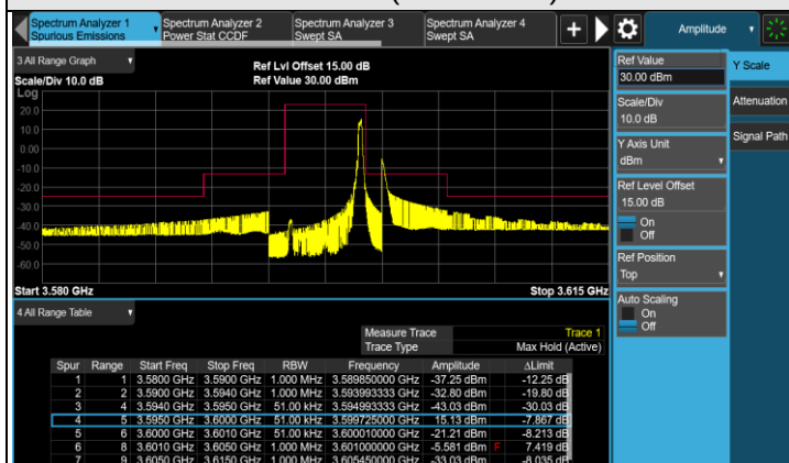
1RB#MAX (3597.5MHz)
