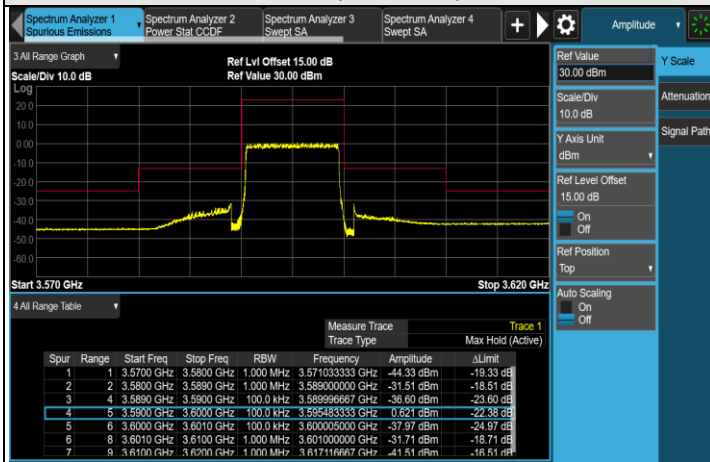
FULL (3595MHz)
