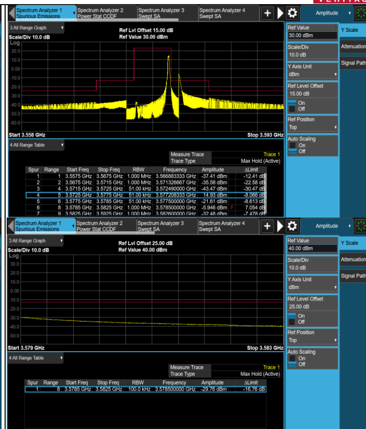
1RB#MAX (3575MHz)
