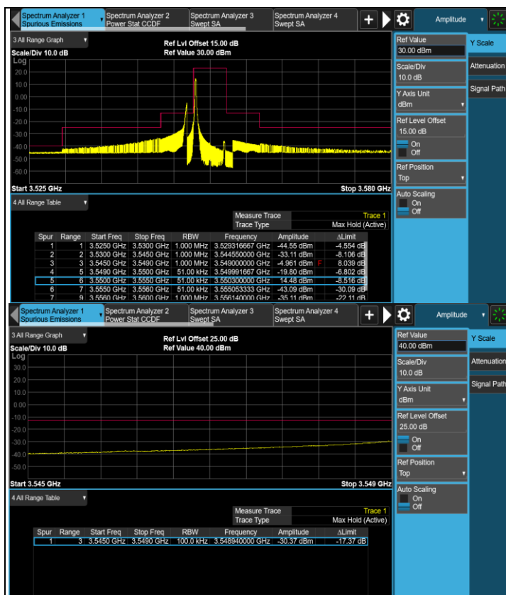
1RB#0 (3552.5MHz)
