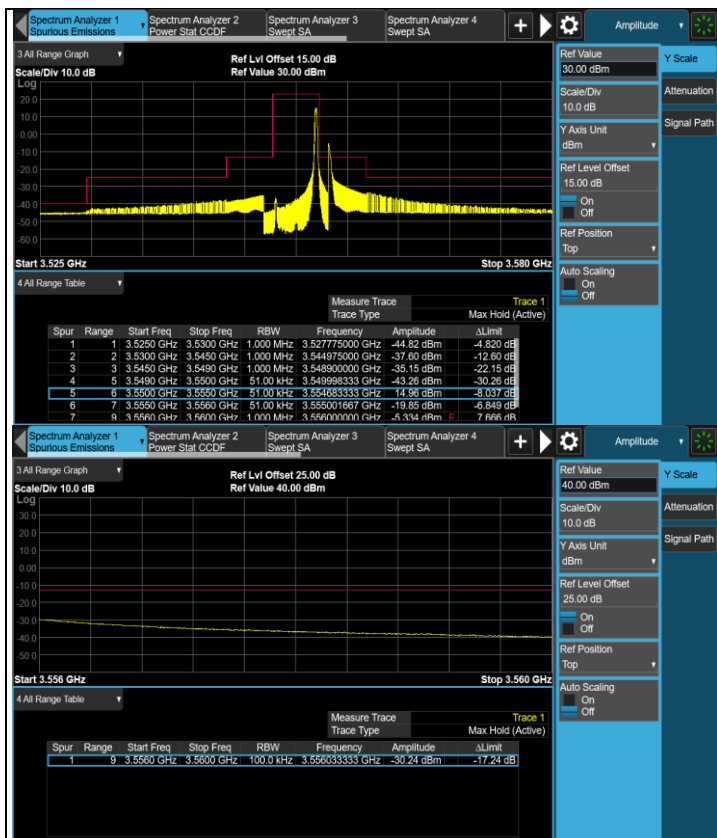
1RB#MAX (3552.5MHz)
