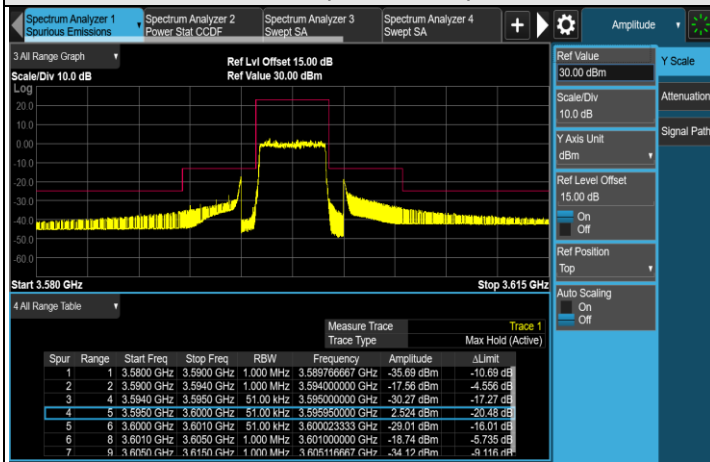
FULL (3597.5MHz)
