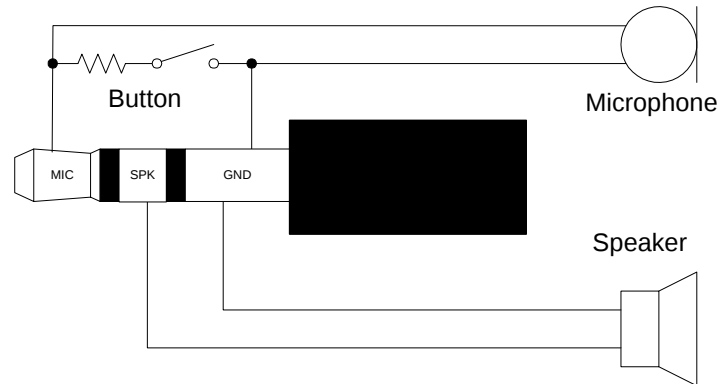
Figure 11 - Pushbutton microphone headset
