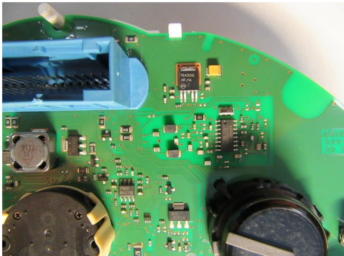
Detail PCB #2 View
