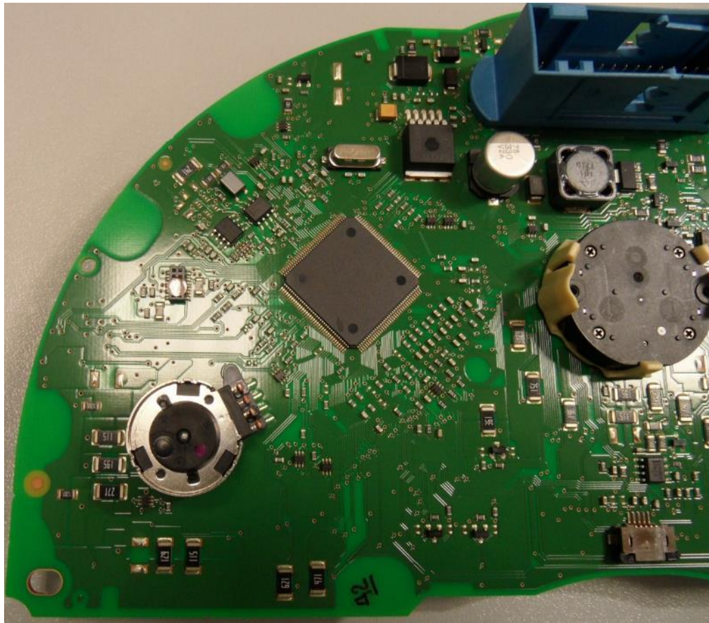
Detail PCB #4 View
