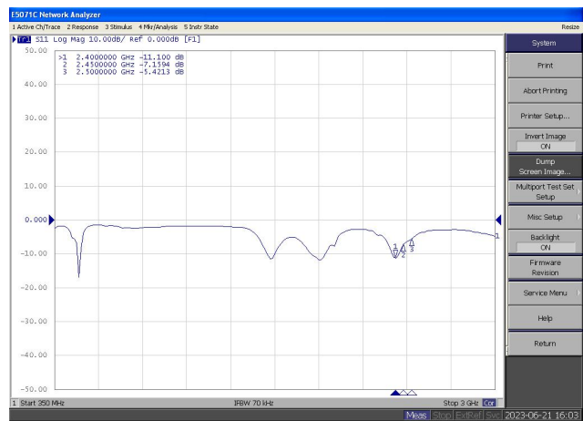
return LOSS
