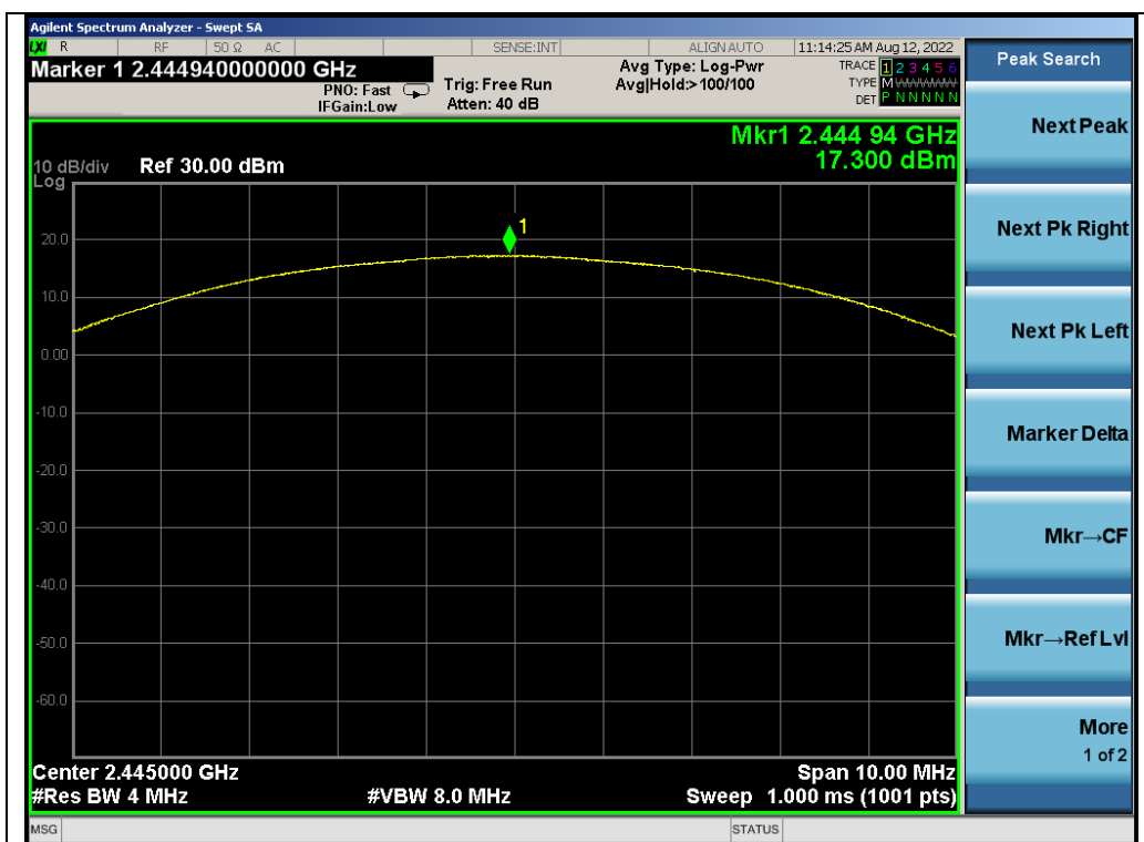
Test_Graph_GFSK_ANT1_2445_Peak Power
