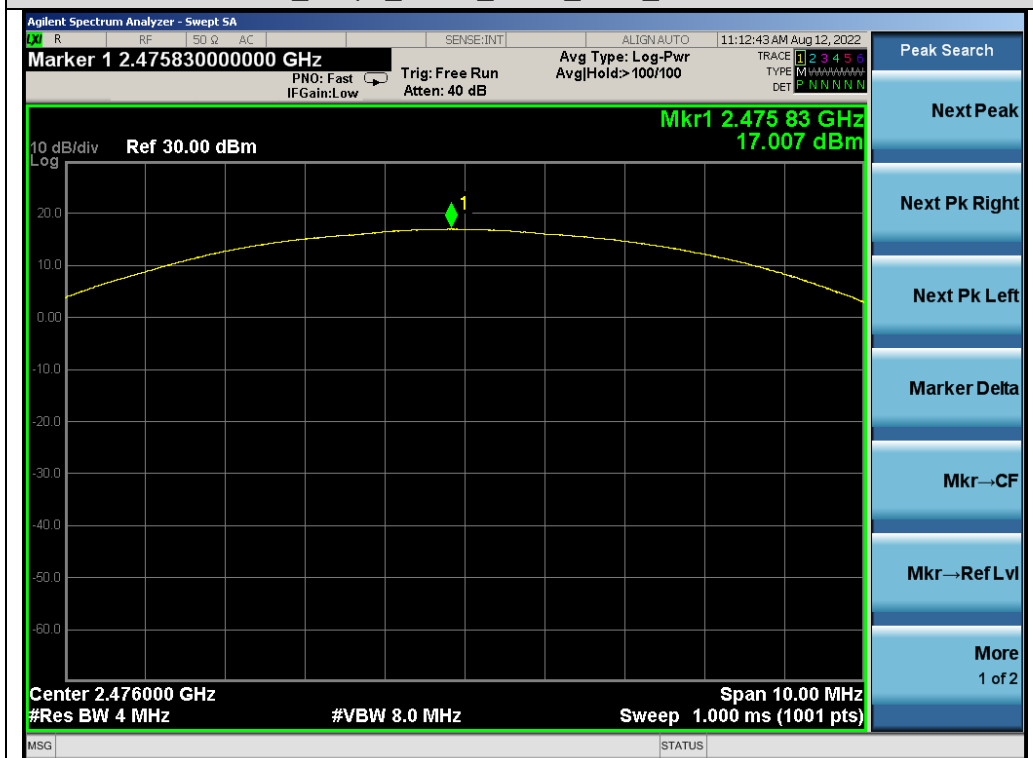
Test_Graph_GFSK_ANT1_2476_Peak Power
