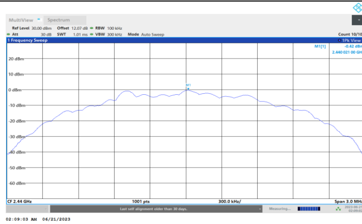
BLE_2M_Ant1_2440_0~Reference
