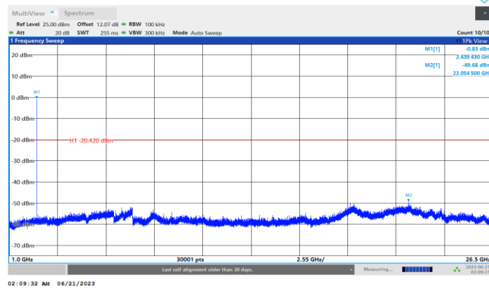
BLE_2M_Ant1_2440_1000~26500
