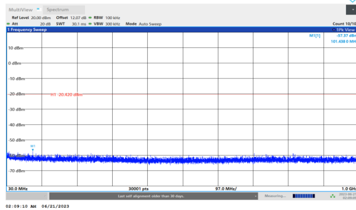
BLE_2M_Ant1_2440_30~1000
