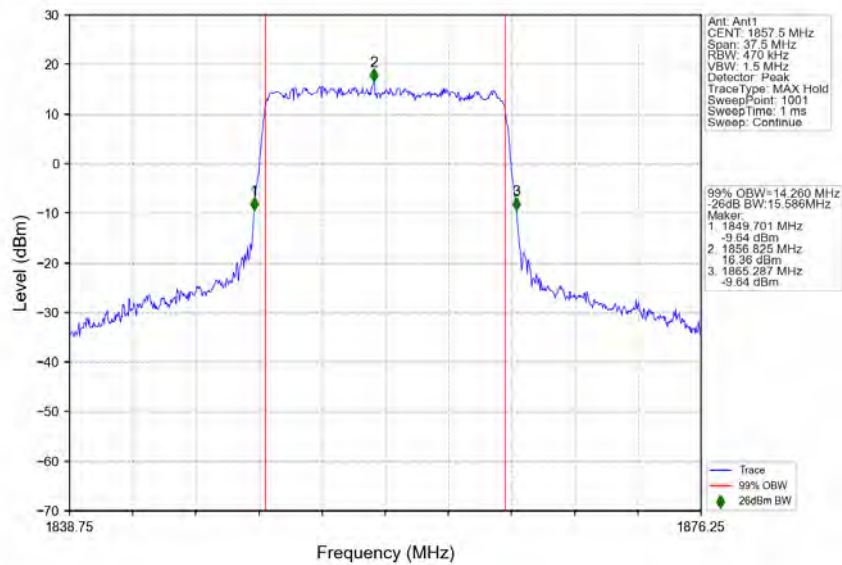
n2_15kHz_SISO_NTNV_15MHz_CP-OFDM_64_QAM_1857.5MHz_Outer_Full
