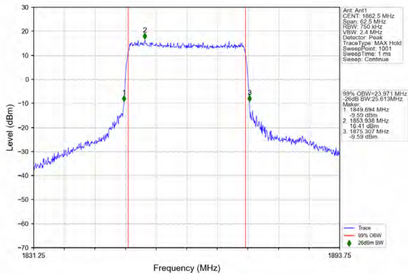
n2_15kHz_SISO_NTNV_25MHz_CP-OFDM_QPSK_1862.5MHz_Outer_Full
