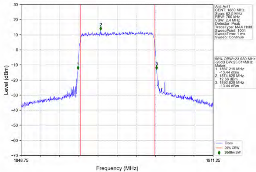
n2_15kHz_SISO_NTNV_25MHz_CP-OFDM_256_QAM_1880MHz_Outer_Full
