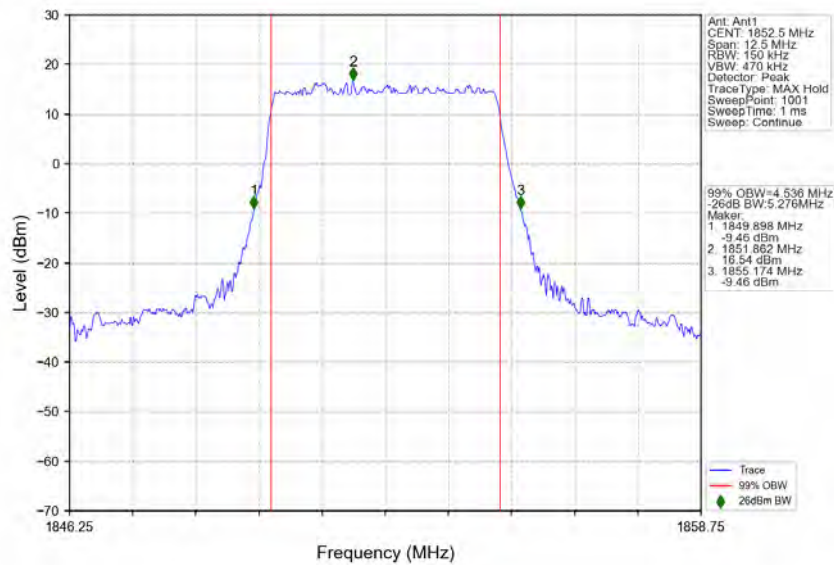
n2_15kHz_SISO_NTNV_5MHz_DFT-s-OFDM_64 QAM_1852.5MHz_Outer_Full
