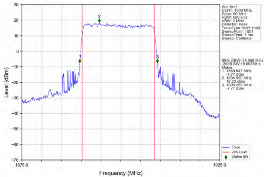
n2_15kHz_SISO_NTNV_20MHz_DFT-s-OFDM_QPSK_1900MHz_Outer_Full
