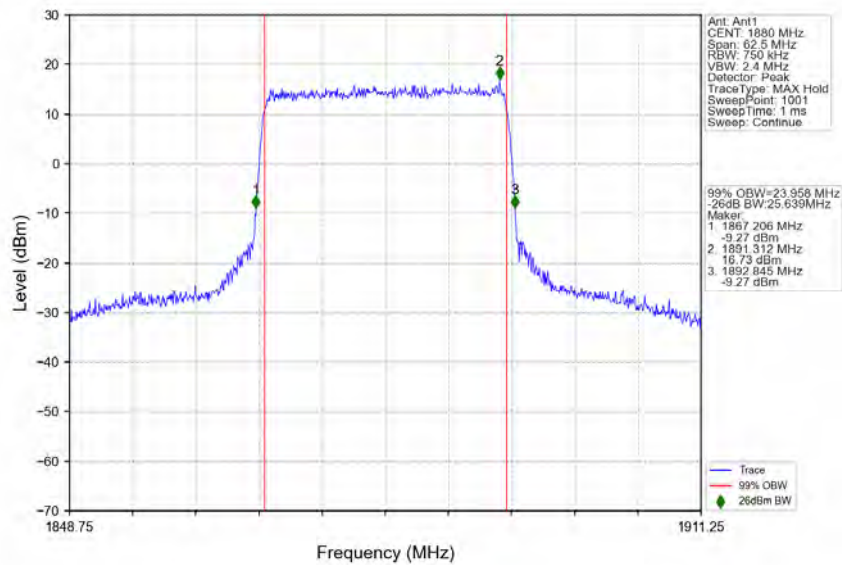
n2_15kHz_SISO_NTNV_25MHz_CP-OFDM_16_QAM_1880MHz_Outer_Full
