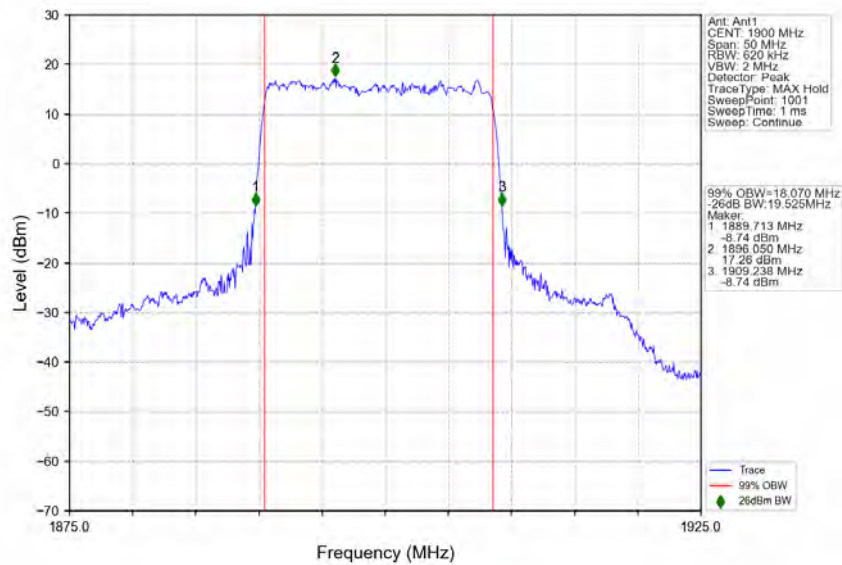
n2_15kHz_SISO_NTNV_20MHz_DFT-s-OFDM_64_QAM_1900MHz_Outer_Full
