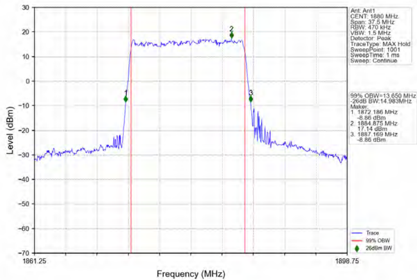
n2_15kHz_SISO_NTNV_15MHz_DFT-s-OFDM_16_QAM_1880MHz_Outer_Full
