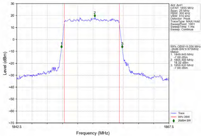
n2_15kHz_SISO_NTNV_10MHz_DFT-s-OFDM QPSK 1855MHz_Outer_Full
