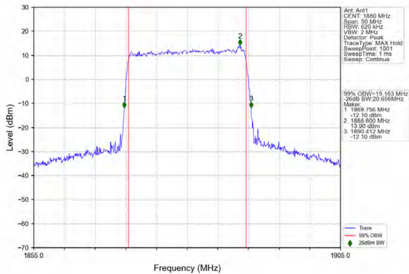
n2_15kHz_SISO_NTNV_20MHz_CP-OFDM_256_QAM_1880MHz_Outer_Full
