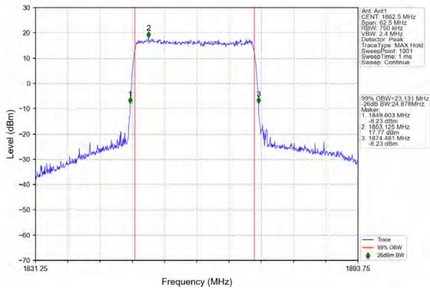
n2_15kHz_SISO_NTNV_25MHz_DFT-s-OFDM_QPSK_1862.5MHz_Outer_Full
