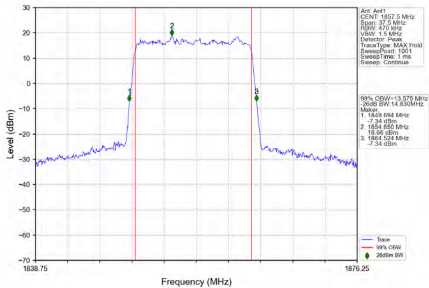
n2_15kHz_SISO_NTNV_15MHz_DFT-s-OFDM_QPSK_1857.5MHz_Outer_Full
