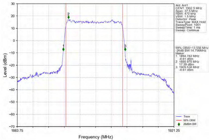
n2_15kHz_SISO_NTNV_15MHz_DFT-s-OFDM_64_QAM_1902.5MHz_Outer_Full
