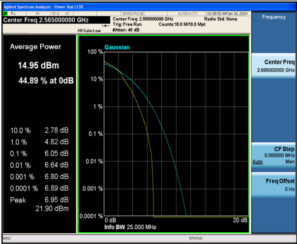
Band7-10MHz-16QAM-21400-1RB#0-PASS
