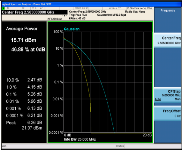
Band7-10MHz-QPSK-21400-1RB#0-PASS
