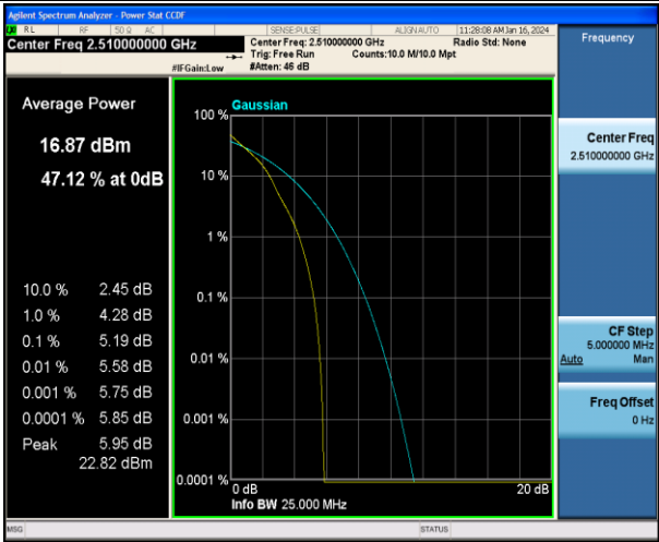
Band7-20MHz-QPSK-20850-1RB#0-PASS
