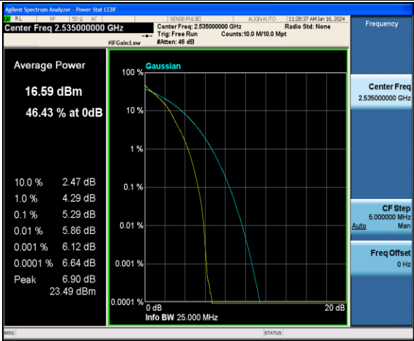
Band7-20MHz-QPSK-21100-1RB#0-PASS
