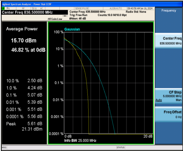
Band5-10MHz-QPSK-20525-1RB#0-PASS
