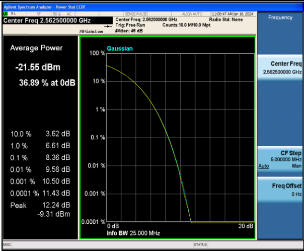
Band7-15MHz-QPSK-21375-1RB#0-PASS
