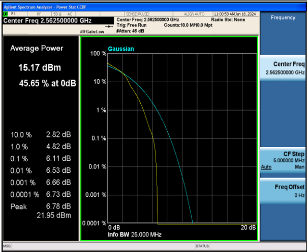
Band7-15MHz-16QAM-21375-1RB#0-PASS
