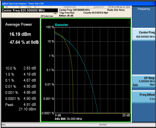
Band5-3MHz-16QAM-20415-1RB#0-PASS
