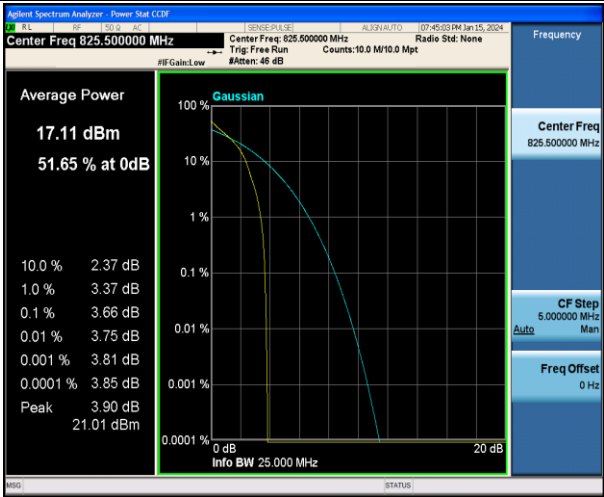
Band5-3MHz-QPSK-20415-1RB#0-PASS
