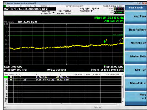
LoRa (100kHz) MIDDLE CHANNEL, SPURIOUS 3 GHz ~ 25 GHz
