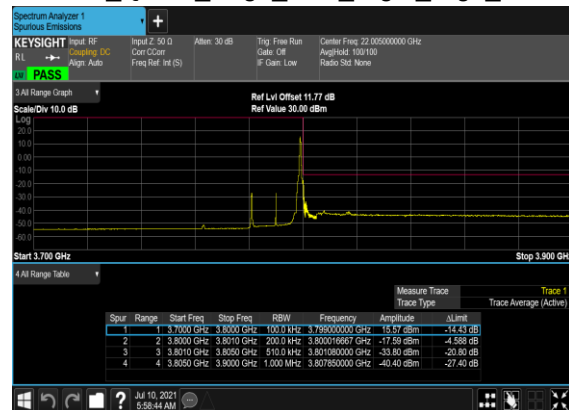
N78(20M)_DFT-s- OFDM_QPSK_Edge_1RB_Right_High_CH
