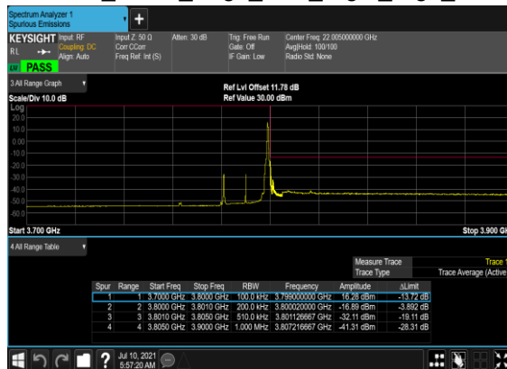
N78(20M)_DFT-s- OFDM_BPSK_Edge_1RB_Right_High_CH
