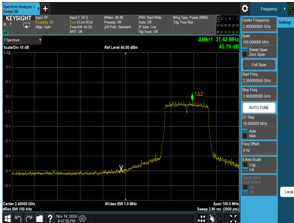
Plot 7-18. Band Edge Antenna WF8 (802.11ax OFDMA – RU242 – Ch. 4)
