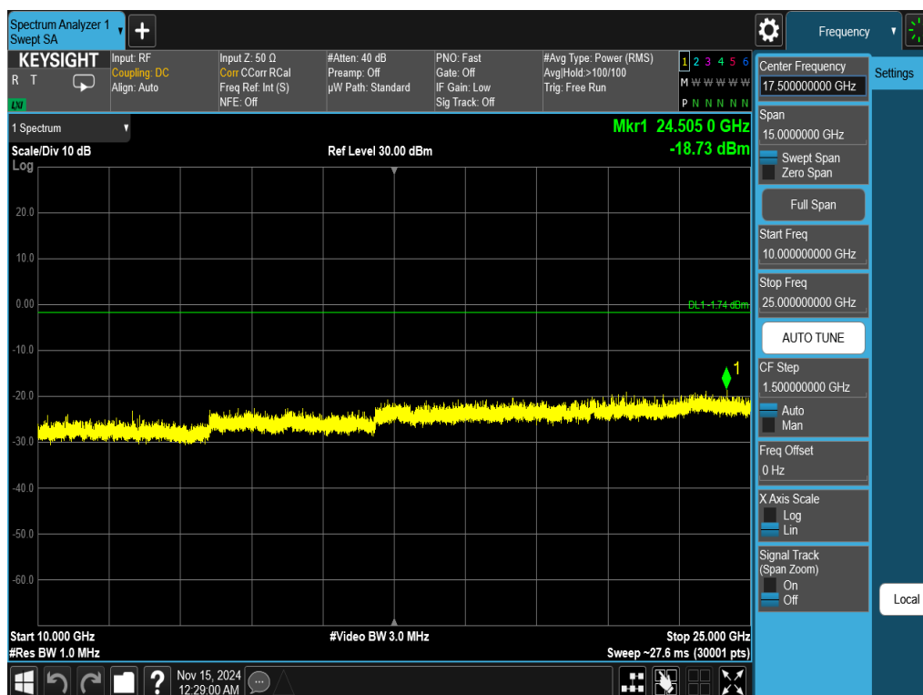
Plot 7-56. Conducted Spurious Plot Antenna WF7b (802.11ax OFDMA – RU26 – Ch. 1)
