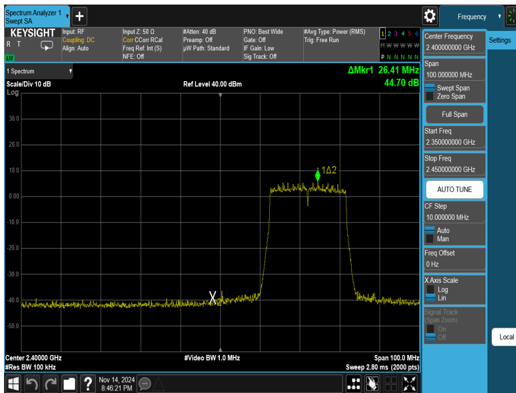
Plot 7-17. Band Edge Antenna WF8 (802.11ax OFDMA – RU242 – Ch. 3)
