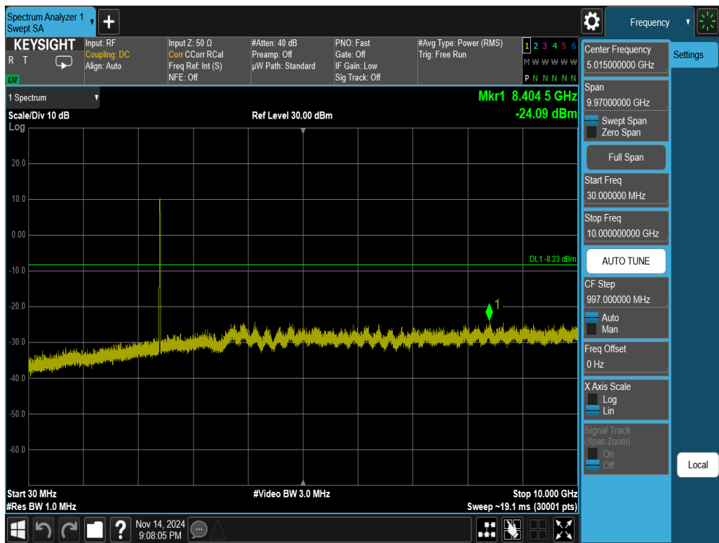
Plot 7-49. Conducted Spurious Plot Antenna WF8 (802.11ax OFDMA – RU242 – Ch. 1)
