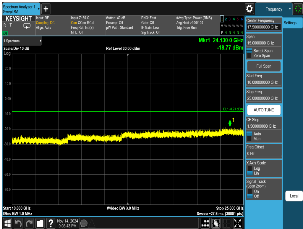
Plot 7-50. Conducted Spurious Plot Antenna WF8 (802.11ax OFDMA – RU242 – Ch. 1)
