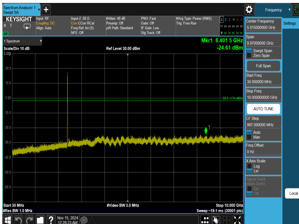
Plot 7-55. Conducted Spurious Plot Antenna WF7b (802.11ax OFDMA – RU26 – Ch. 1)
