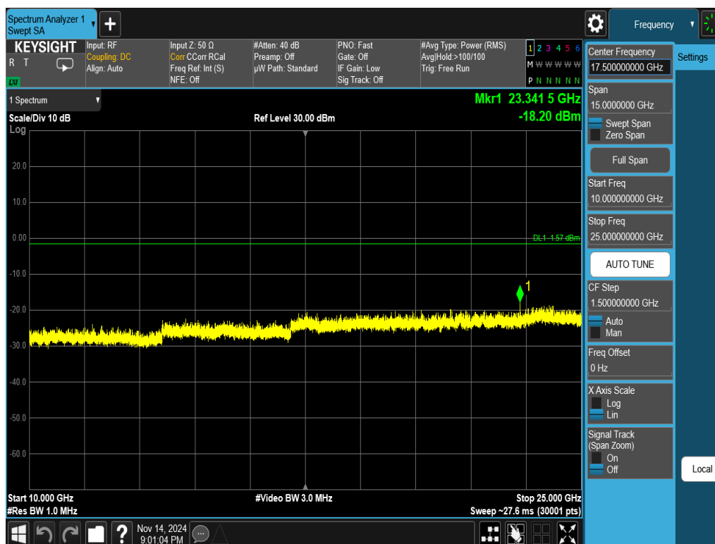
Plot 7-46. Conducted Spurious Plot Antenna WF8 (802.11ax OFDMA – RU26 – Ch. 6)
