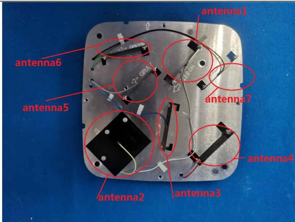
(9) EUT Photo (AP460S12C)
