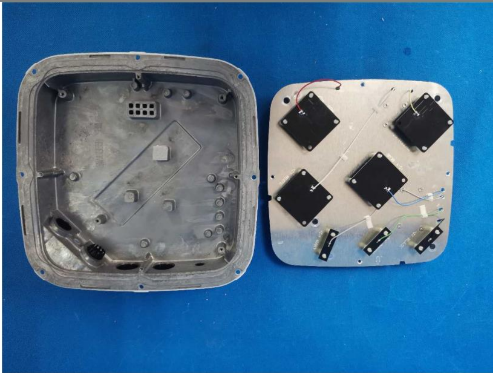
(4) EUT Photo (AP460S6C)
