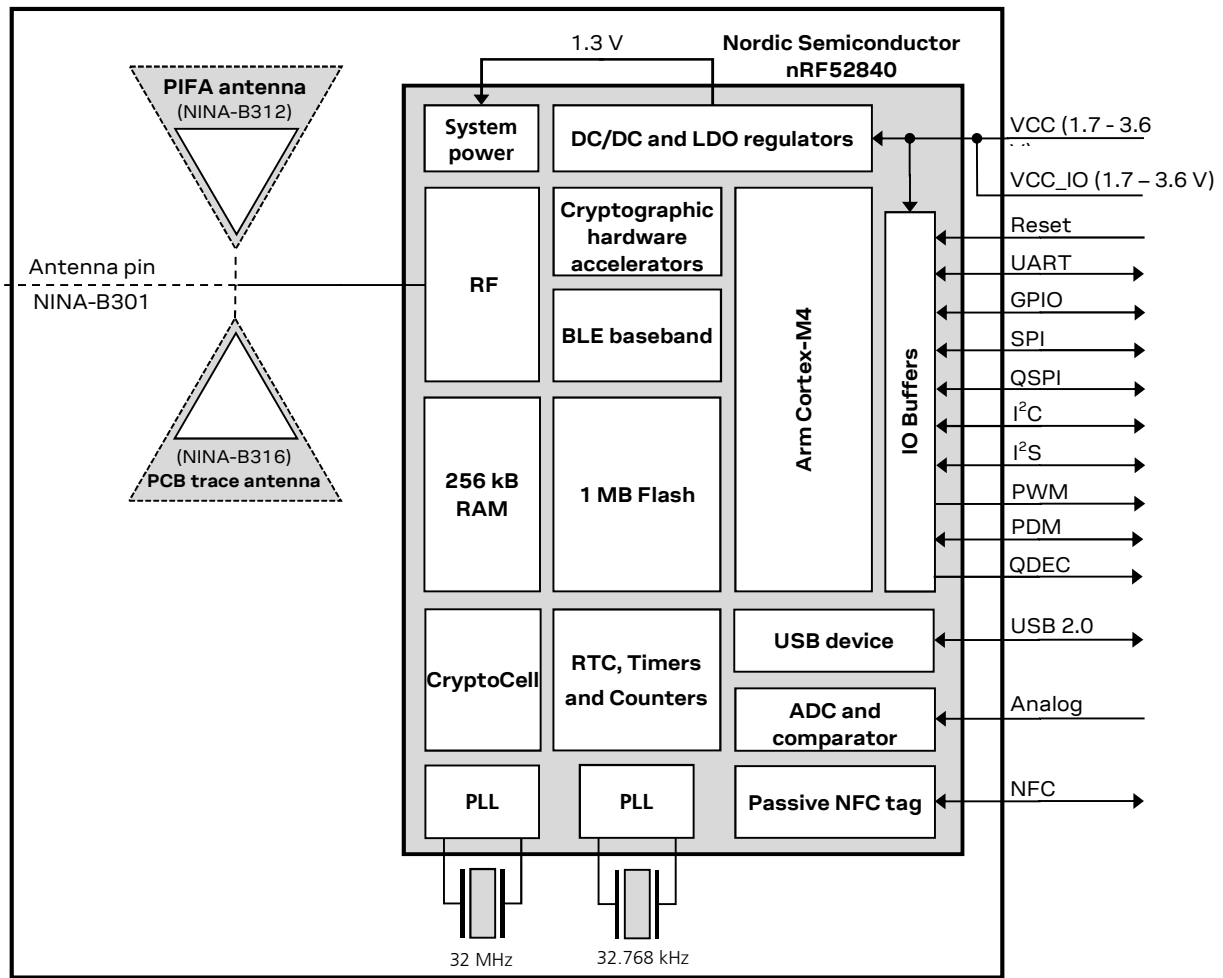
Figure 1: NINA-B31 series block diagram
