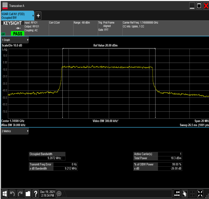
n66_10MHz_15kHz_1745MHz_DFT-s-OFDM 256 QAM_RB50@0
