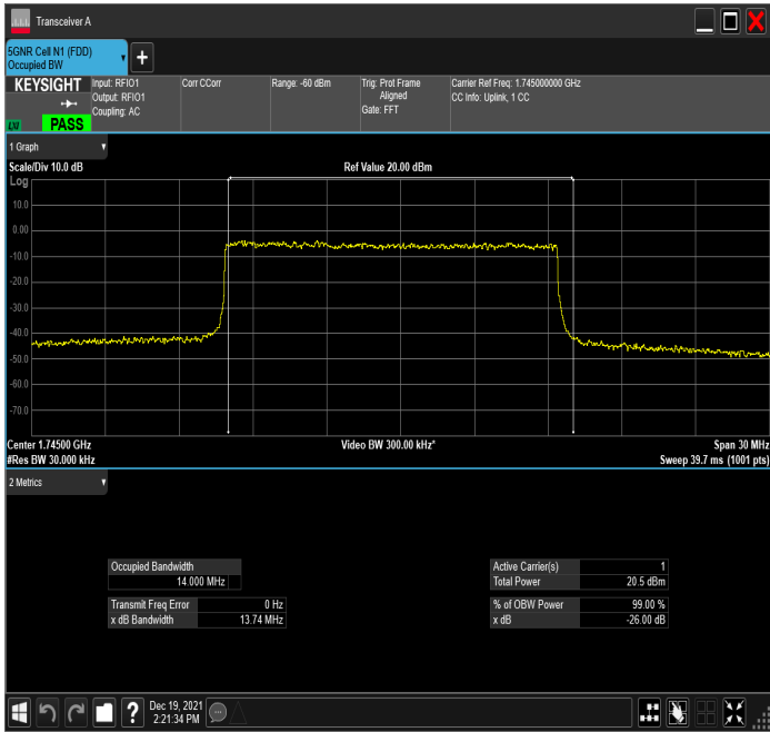
n66_15MHz_15kHz_1745MHz_DFT-s-OFDM 64 QAM_RB75@0
