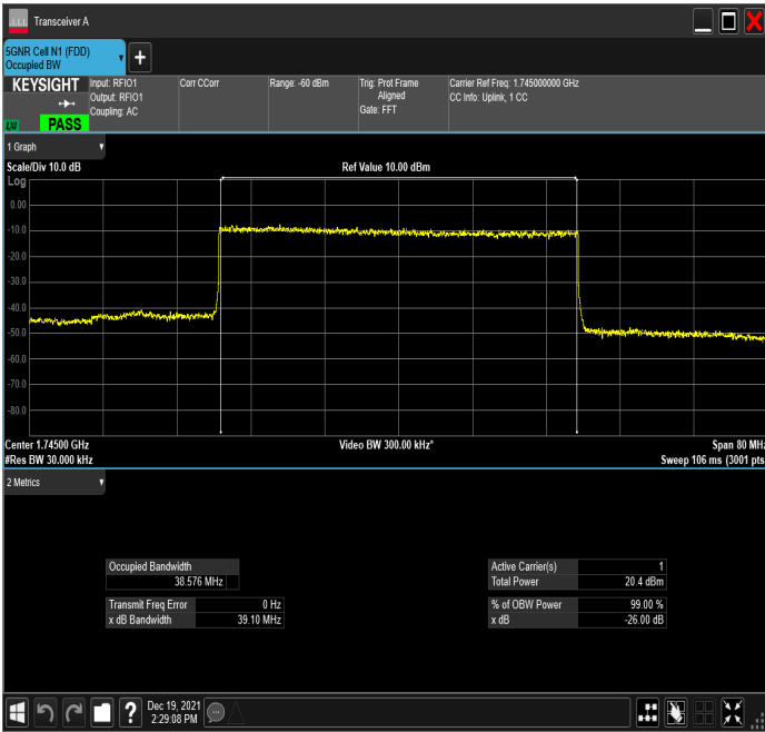
n66_40MHz_15kHz_1745MHz_DFT-s-OFDM 64 QAM_RB216@0
