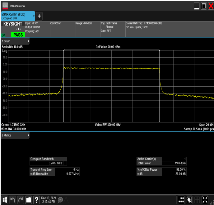
n66_10MHz_15kHz_1745MHz_CP-OFDM 16 QAM_RB52@0
