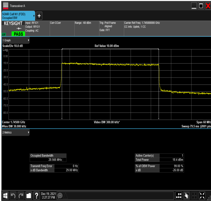
n66_30MHz_15kHz_1745MHz_DFT-s-OFDM 256 QAM_RB160@0
