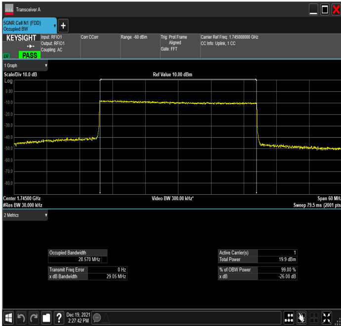
n66_30MHz_15kHz_1745MHz_CP-OFDM 16 QAM_RB160@0
