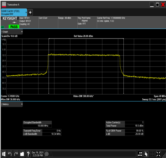
n66_20MHz_15kHz_1745MHz_DFT-s-OFDM 256 QAM_RB100@0
