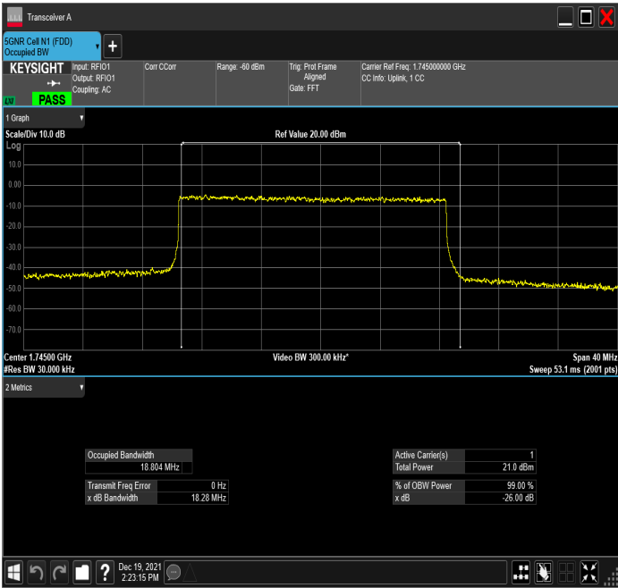
n66_20MHz_15kHz_1745MHz_DFT-s-OFDM 16 QAM_RB100@0
