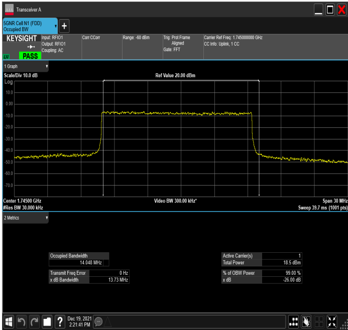
n66_15MHz_15kHz_1745MHz_DFT-s-OFDM 256 QAM_RB75@0
