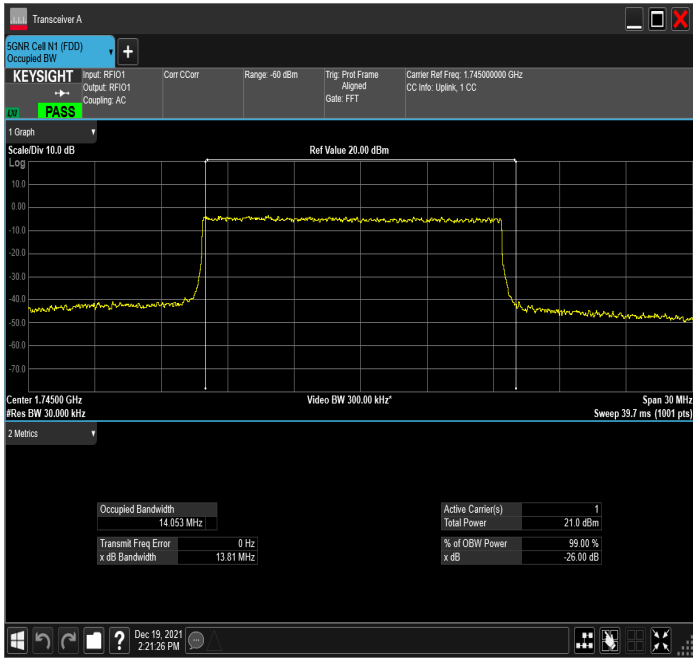
n66_15MHz_15kHz_1745MHz_DFT-s-OFDM 16 QAM_RB75@0
