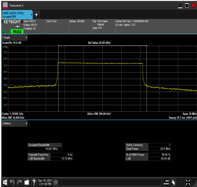
n66_15MHz_15kHz_1745MHz_CP-OFDM QPSK_RB75@0
