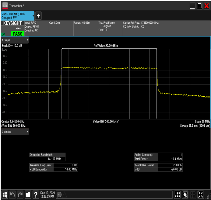
n66_15MHz_15kHz_1745MHz_CP-OFDM 64 QAM_RB79@0
