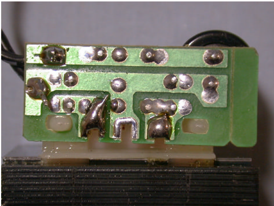
(32) EUT Photo
