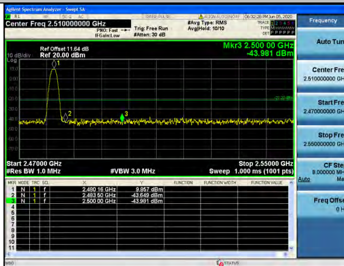
DH5_Ant2_High_2480_Peak
