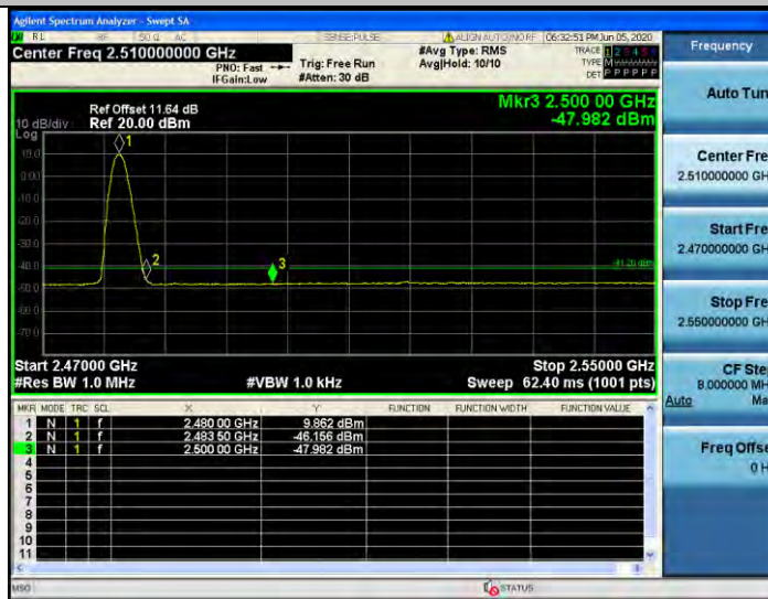
DH5_Ant2_High_2480_Peak
