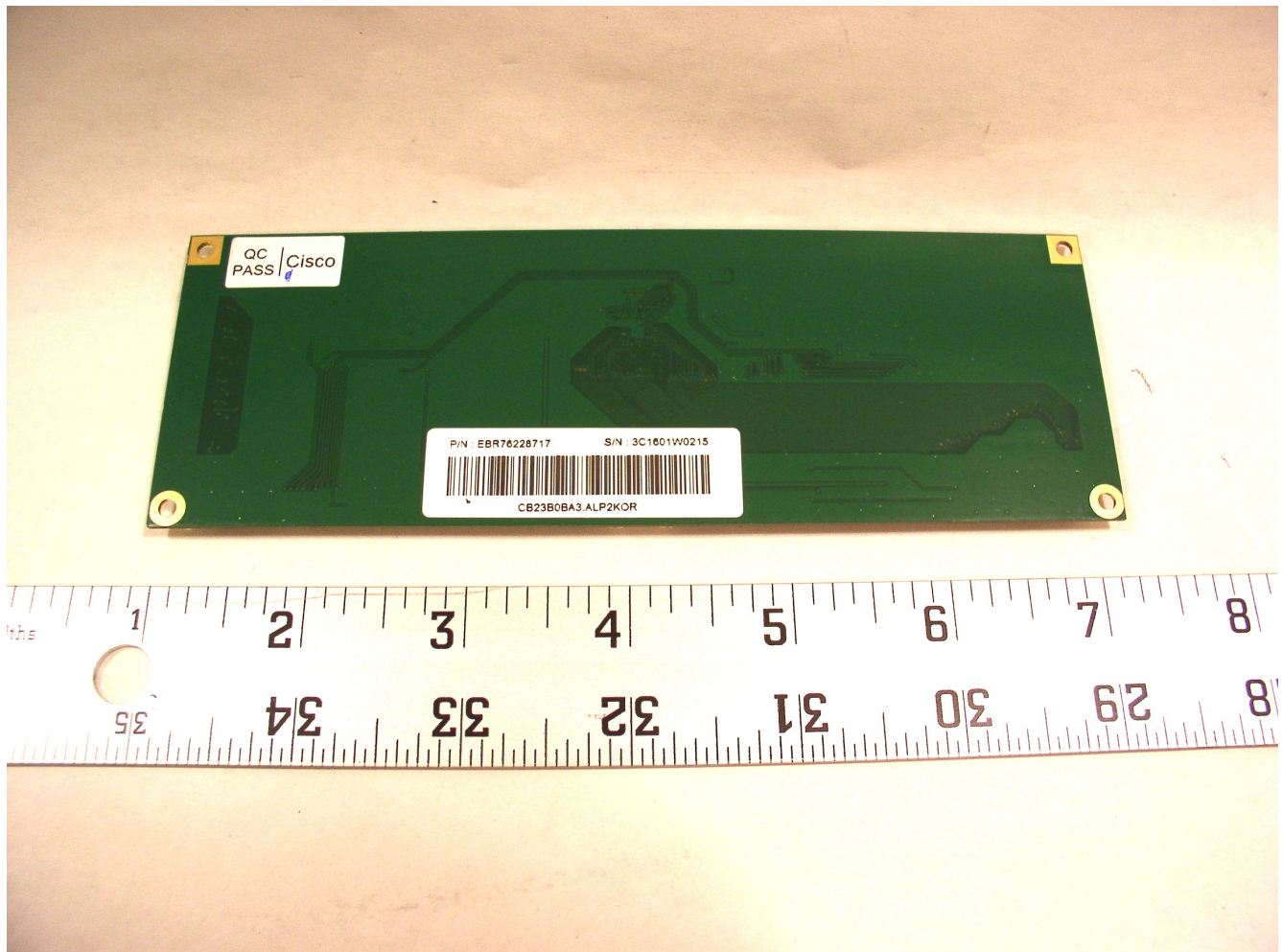
CP-DX80 : Internal PCB touch screen controller (Botom view)
