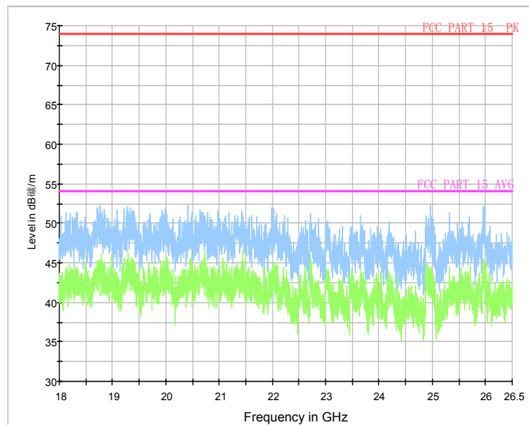
Fig.87. Radiated emission: 8DPSK, 18 GHz - 26 GHz
