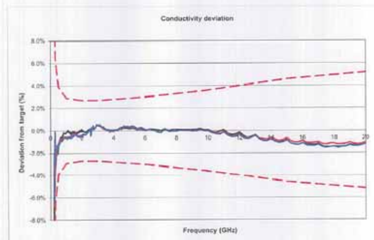
Fig. 3.2 Methanol conductivity deviation from target, 200 MHz – 20 GHz Conductivity error can be high at low frequencies due to the low absolute conductivity values
