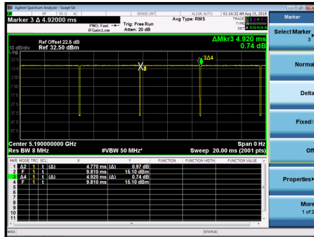
802.11ac-VHT40 (T = 4.780ms)
