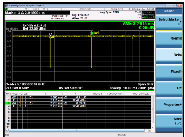
802.11ax-HE20 (T = 2.865ms)
