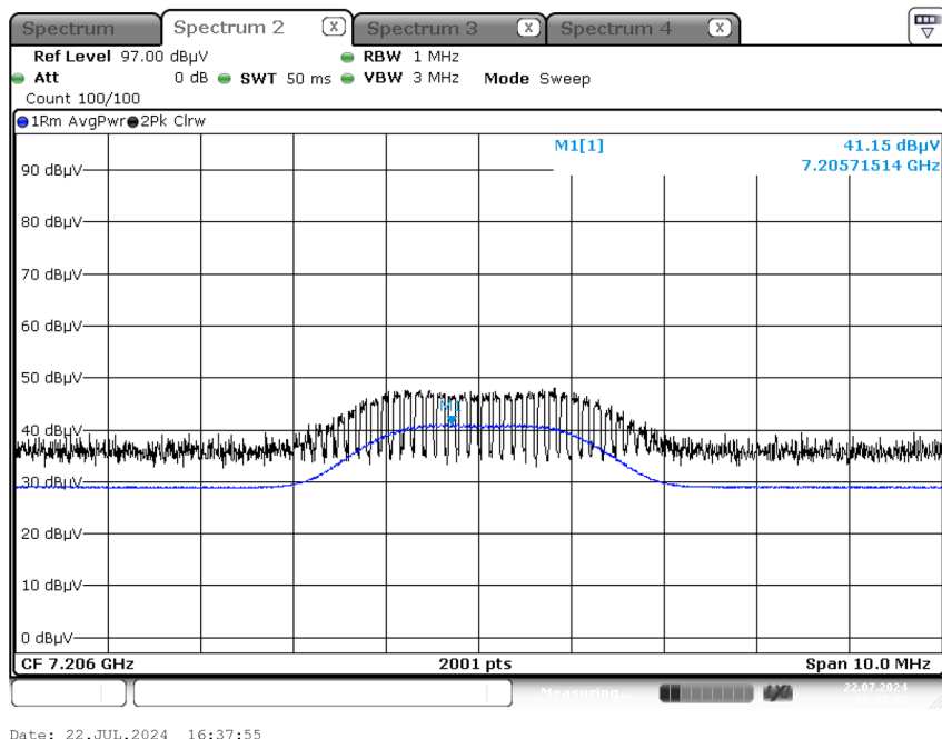
Radiated Spurious Emissions plot – Average Result (Ch.0 3rd Harmonic)
