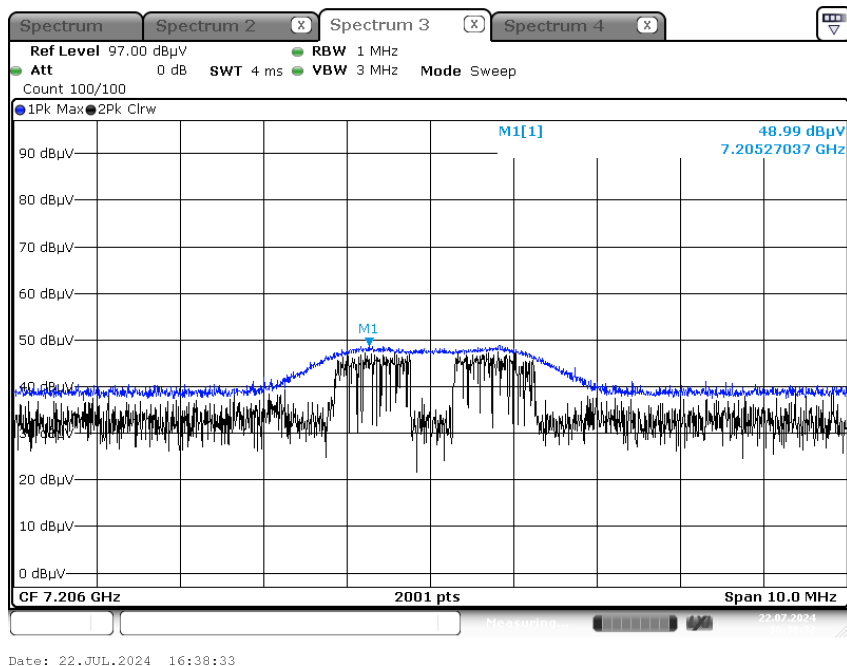
Radiated Spurious Emissions plot – Peak Result (Ch.0 3rd Harmonic)
