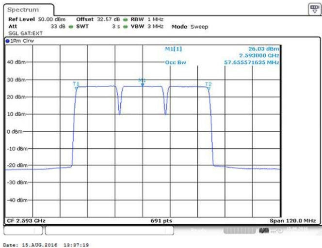
Figure 63 Occupied Bandwidth–64QAM (2573/ 2593/ 2613 MHz) (3 X 20 MHz Channel BW)
