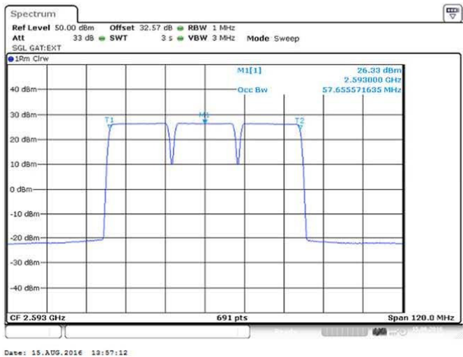
Figure 66 Occupied Bandwidth–64QAM (2573/ 2593/ 2613 MHz) (3 X 20 MHz Channel BW)
