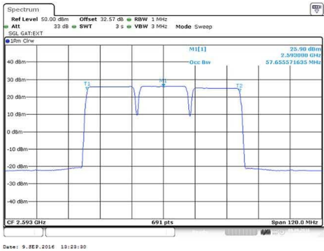
Figure 74 Occupied Bandwidth–QPSK (2573/ 2593/ 2613 MHz) (3 X 20 MHz Channel BW)
