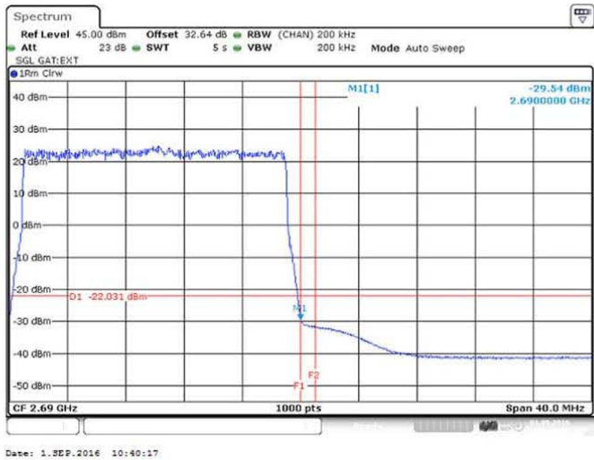
Figure 92 Spurious Emissions (Upper Band Edge) – 16QAM (2680.0 MHz) (20MHz Channel BW)
