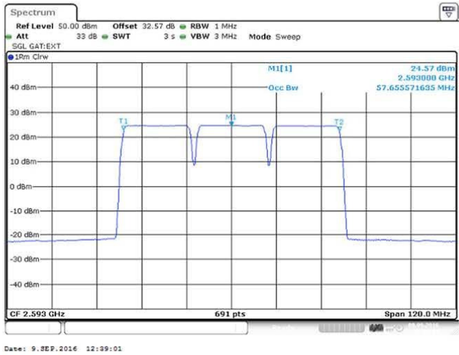
Figure 78 Occupied Bandwidth–64QAM (2573/ 2593/ 2613 MHz) (3 X 20 MHz Channel BW)
