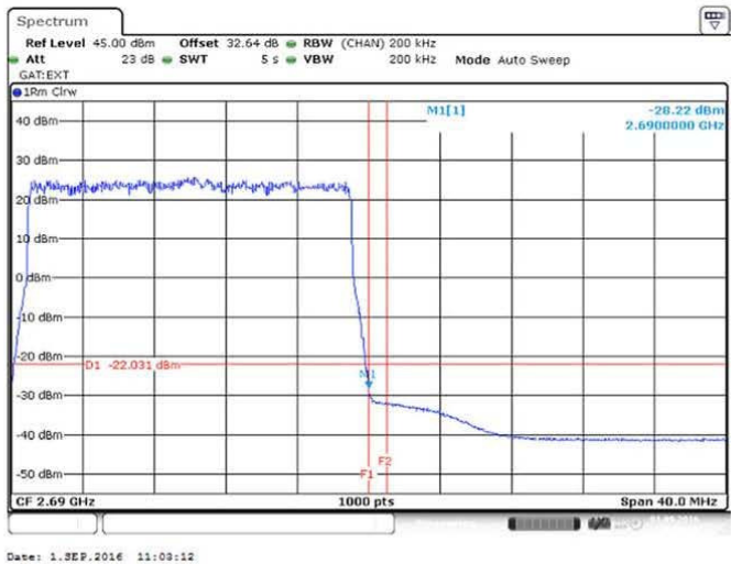
Figure 116 Spurious Emissions (Upper Band Edge) – 16QAM (2680.0 MHz) (20MHz Channel BW)
