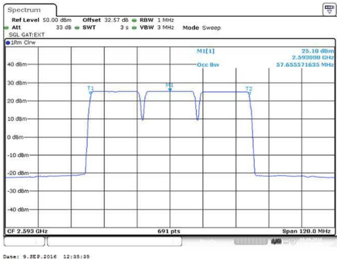
Figure 77 Occupied Bandwidth–QPSK (2573/ 2593/ 2613 MHz) (3 X 20 MHz Channel BW)
