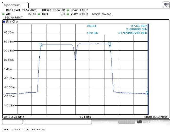
Figure 44 Occupied Bandwidth –QPSK (2583/ 2603 MHz) (2 X 20MHz Channel BW)
