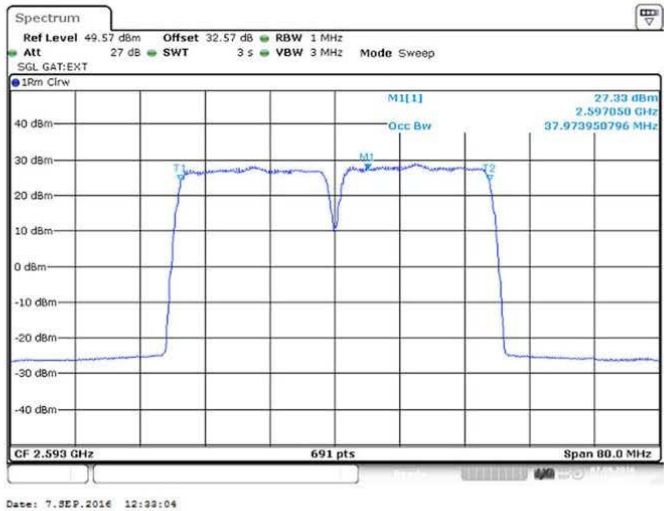
Figure 58 Occupied Bandwidth –16QAM (2583/ 2603 MHz) (2 X 20 MHz Channel BW)
