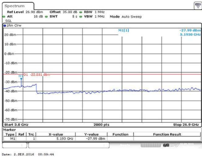
Figure 11842 Spurious Emissions (3GHz – 26.900GHz) – 16QAM (2593.0 MHz) (20MHz Channel BW)
