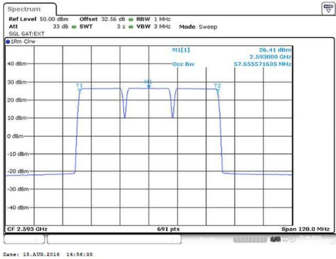
Figure 75 Occupied Bandwidth–64QAM (2573/ 2593/ 2613 MHz) (3 X 20 MHz Channel BW)
