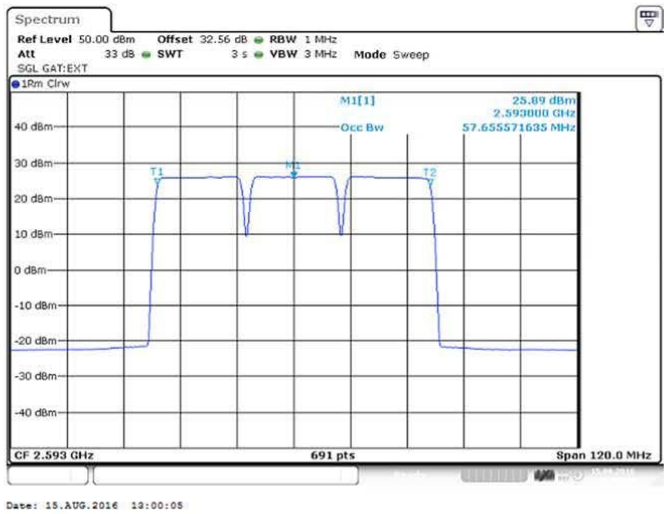
Figure 59 Occupied Bandwidth–QPSK (2573/ 2593/ 2613 MHz) (3 X 20 MHz Channel BW)
