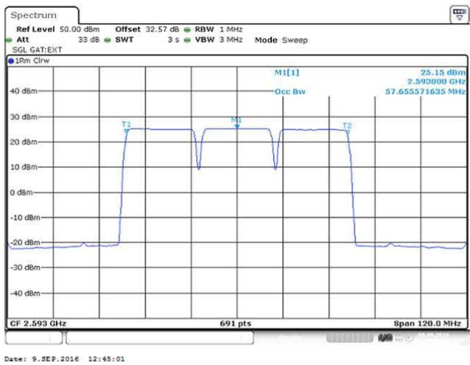
Figure 80 Occupied Bandwidth–QPSK (2573/ 2593/ 2613 MHz) (3 X 20 MHz Channel BW)
