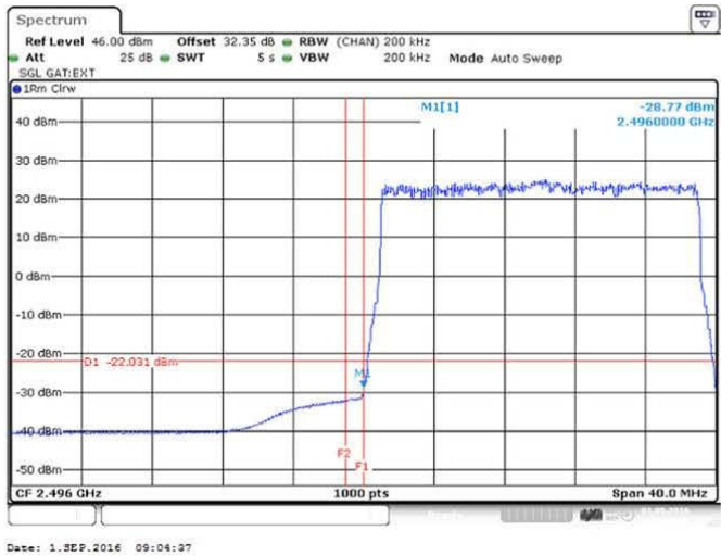
Figure 115 Spurious Emissions (LowerBand Edge) – 16QAM (2506.0 MHz) (20MHz Channel BW)
