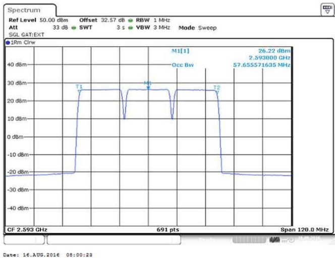
Figure 81 Occupied Bandwidth–64QAM (2573/ 2593/ 2613 MHz) (3 X 20 MHz Channel BW)
