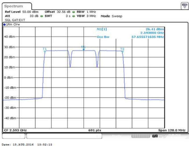
Figure 65 Occupied Bandwidth–QPSK (2573/ 2593/ 2613 MHz) (3 X 20 MHz Channel BW)
