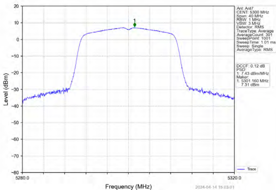
802.11ac(VHT20)_MCH_5300MHz_Ant7_NTNV
