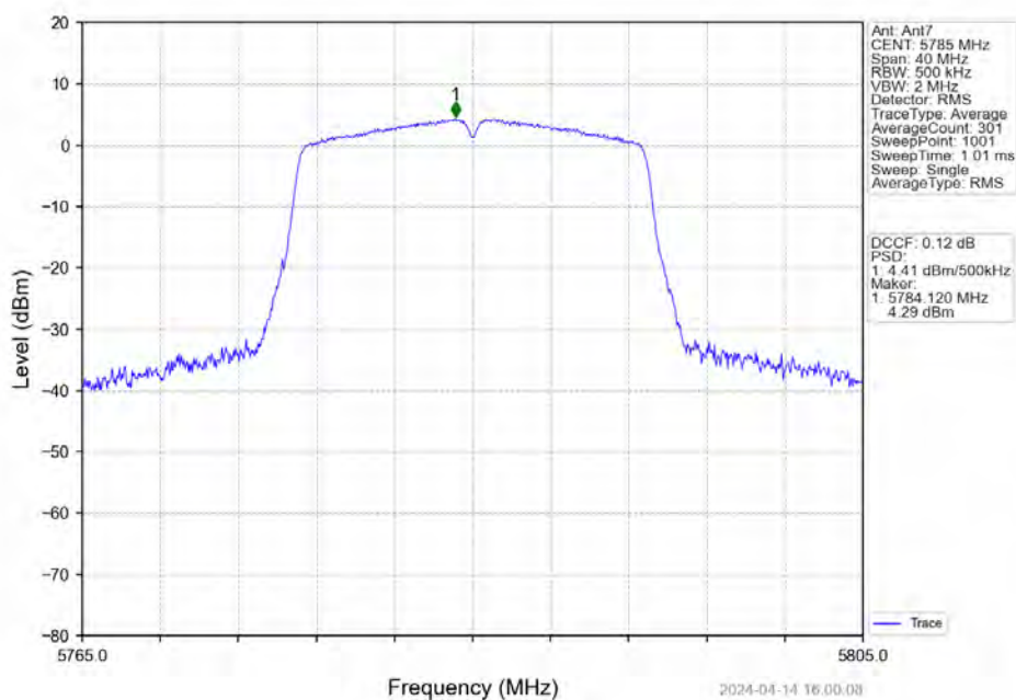
802.11ac(VHT20)_MCH_5785MHz_Ant7_NTNV
