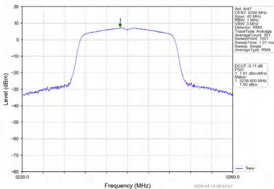
802.11ac(VHT20)_HCH_5240MHz_Ant7_NTNV
