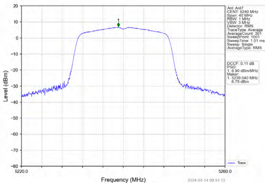
802.11n(HT20)_HCH_5240MHz_Ant7_NTNV
