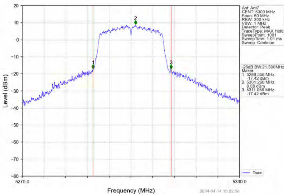
802.11ac(VHT20)_MCH_5300MHz_Ant7_NTNV
