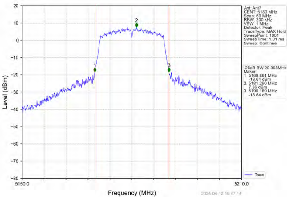
802.11ac(VHT20)_LCH_5180MHz_Ant7_NTNV
