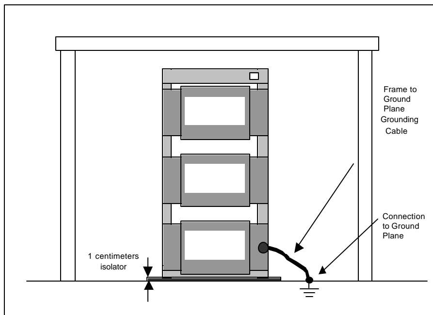
Figure 4-2: System grounding
