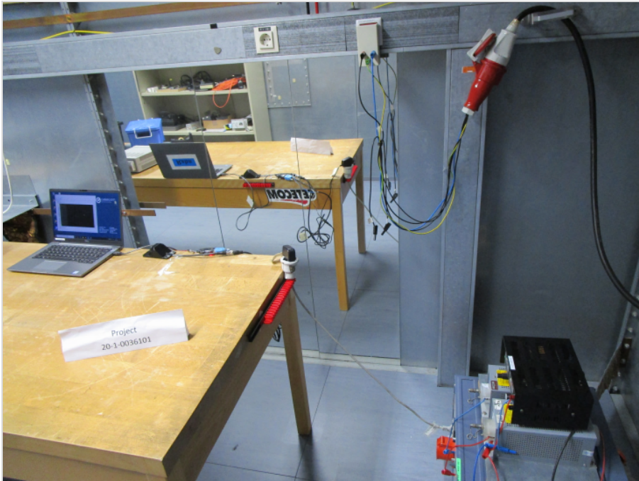
Photograph 1: EUT Test Setup in the AC-Power line conducted emission, close up view
