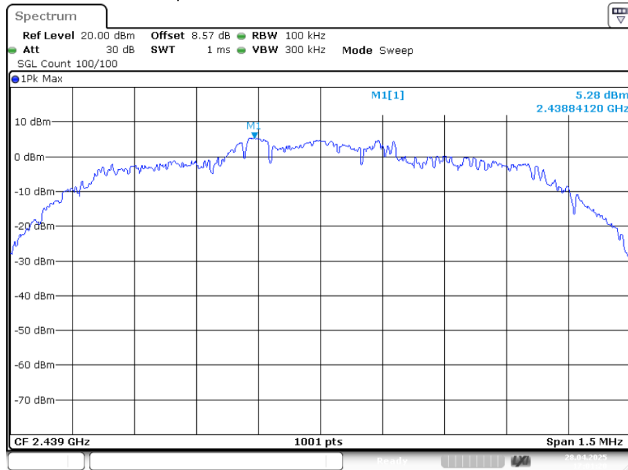
Tx. Spurious NVNT GFSK 2439MHz Ant1 Ref
