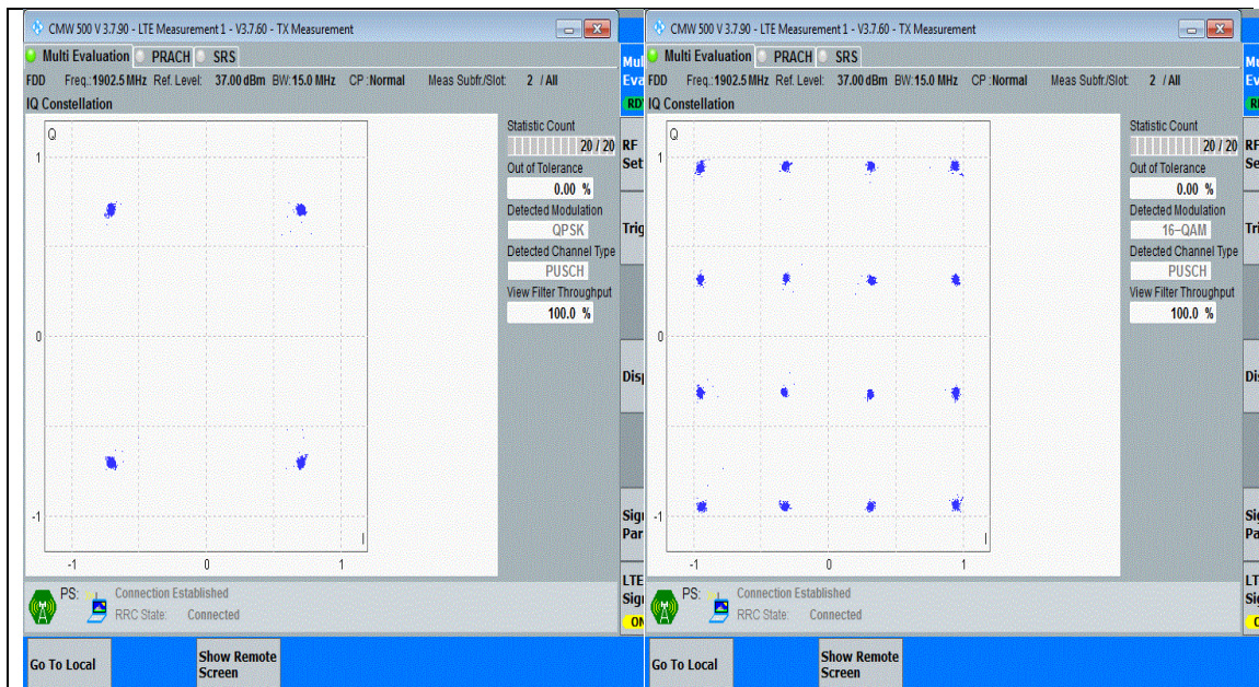
Band2-15MHz-QPSK-19125-75RB#0-PASS
