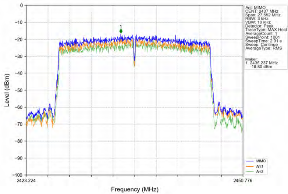
802.11ax(HEW20)_MCH_2437MHz_RU242_Left MIMO NTV
