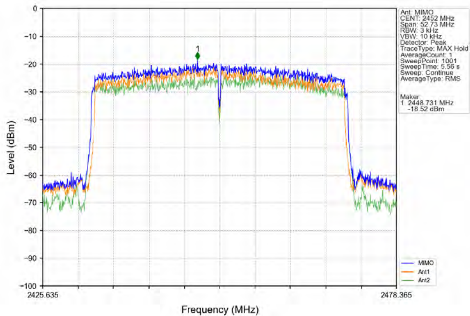
802.11ax(HEW40)_HCH_2452MHz_RU484_Left MIMO NTV
