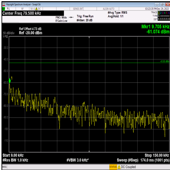
Band2_20MHz_16QAM_19100_1RB#0_0.009~0.15_0.009~0.15 15
