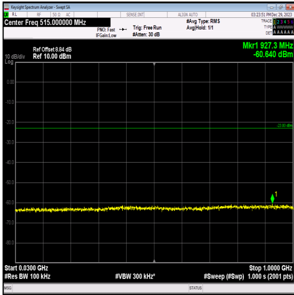
Band2_20MHz_16QAM_19100_1RB#0_30~1000_30~1000
