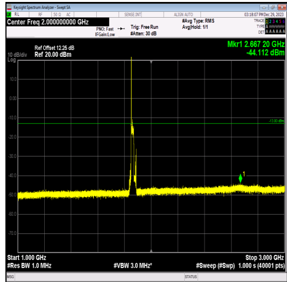
Band2_20MHz_16QAM_18700_1RB#0_1000~3000_1000~3000
