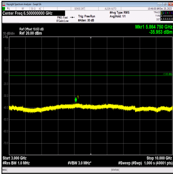
Band5_1.4MHz_QPSK_20407_1RB#0_3000~10000_3000~10000
