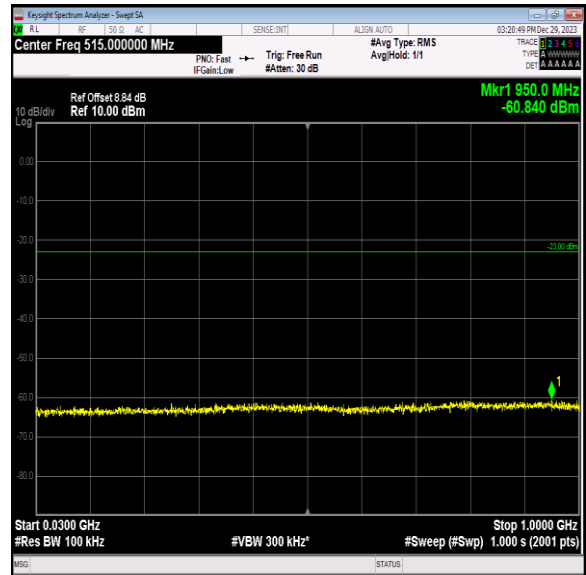
Band2_20MHz_16QAM_18900_1RB#0_30~1000_30~1000
