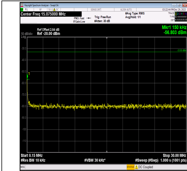
Band2_20MHz_QPSK_19100_1RB#0_0.15~30_0.15~30
