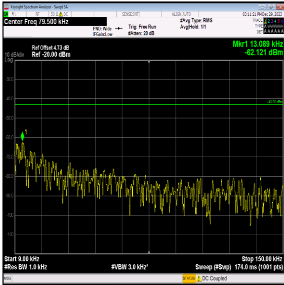
Band2_15MHz_16QAM_18900_1RB#0_0.009~0.15_0.009~0.15
