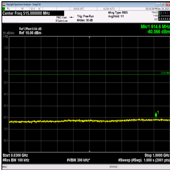
Band2_15MHz_64QAM_19125_1RB#0_30~1000_30~1000
