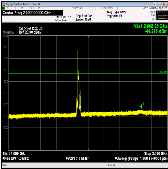
Band2_20MHz_16QAM_18900_1RB#0_1000~3000_1000~3000 00
