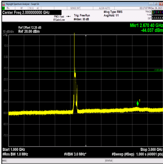
Band2_20MHz_QPSK_18700_1RB#0_1000~3000_1000~3000 0
