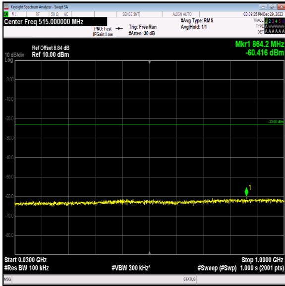
Band2_15MHz_64QAM_18675_1RB#0_30~1000_30~1000
