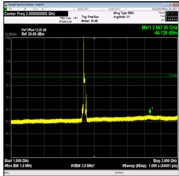
Band2_20MHz_64QAM_18900_1RB#0_1000~3000_1000~3000
