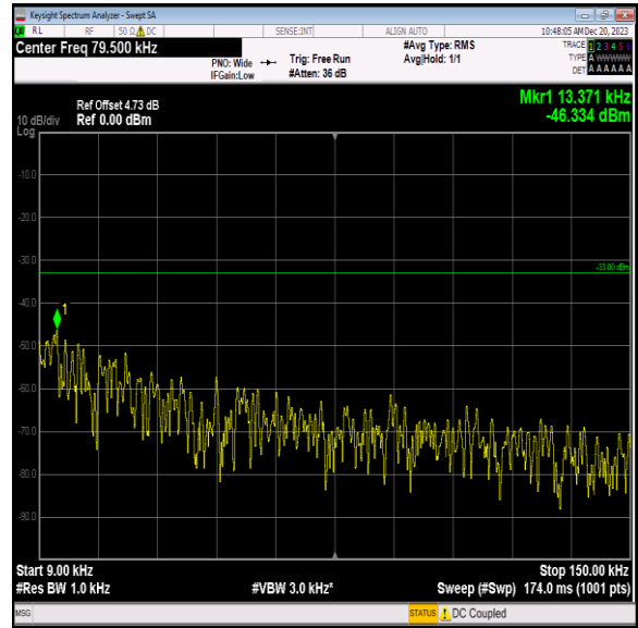
Band5_1.4MHz_QPSK_20525_1RB#0_0.009~0.15_0.009~0.15
