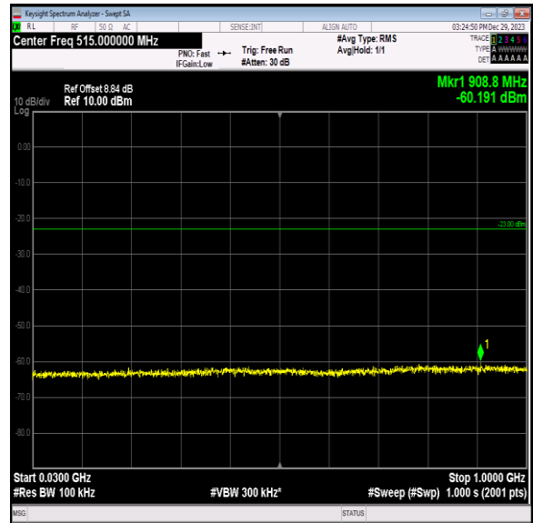
Band2_20MHz_64QAM_19100_1RB#0_30~1000_30~1000
