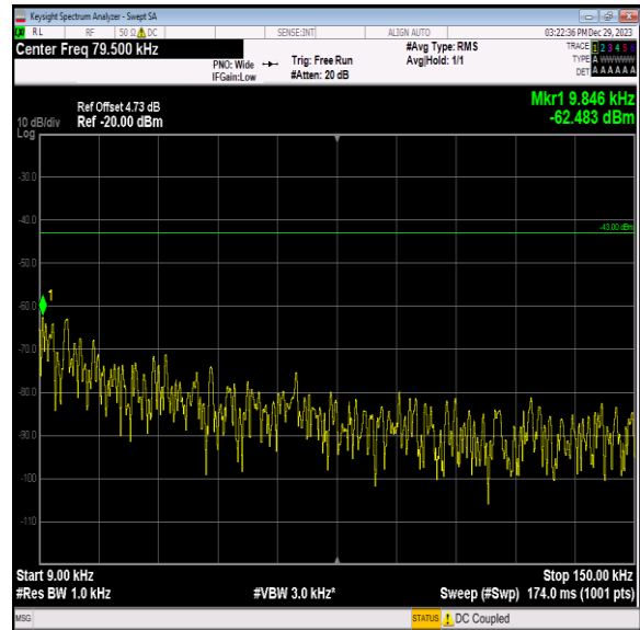
Band2_20MHz_QPSK_19100_1RB#0_0.009~0.15_0.009~0.15 5
