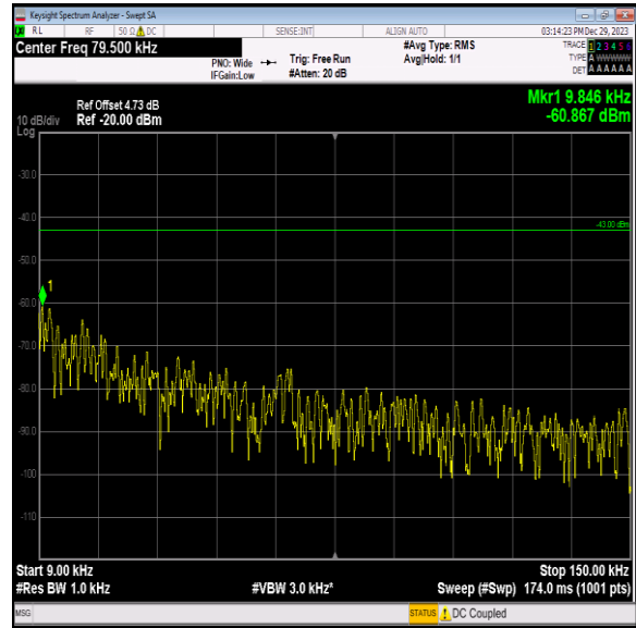
Band2_15MHz_16QAM_19125_1RB#0_0.009~0.15_0.009~0. 15
