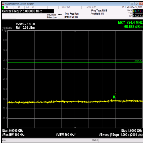
Band2_20MHz_64QAM_18900_1RB#0_30~1000_30~1000
