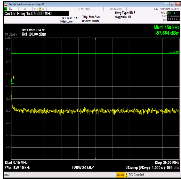
Band2_20MHz_64QAM_18900_1RB#0_0.15~30_0.15~30
