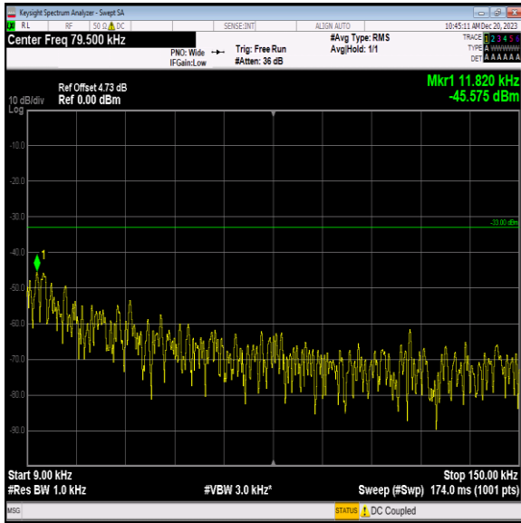
Band5_1.4MHz_QPSK_20407_1RB#0_0.009~0.15_0.009~0.1 5
