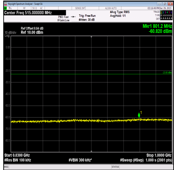
Band2_20MHz_QPSK_18700_1RB#0_30~1000_30~1000
