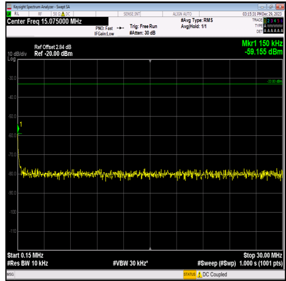
Band2_15MHz_64QAM_19125_1RB#0_0.15~30_0.15~30
