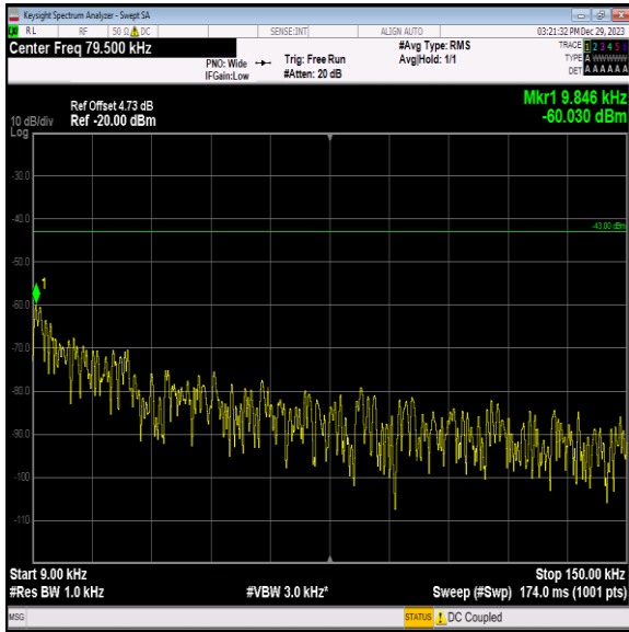
Band2_20MHz_64QAM_18900_1RB#0_0.009~0.15_0.009~0.15
