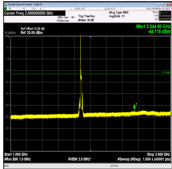
Band2_15MHz_16QAM_18900_1RB#0_1000~3000_1000~3000
