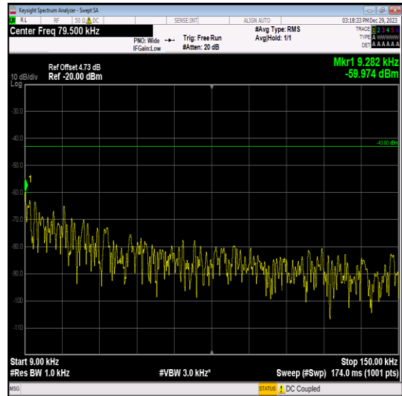
Band2_20MHz_64QAM_18700_1RB#0_0.009~0.15_0.009~0.15
