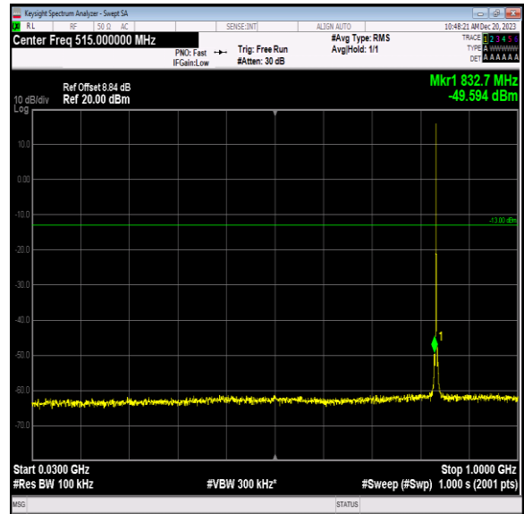
Band5_1.4MHz_QPSK_20525_1RB#0_30~1000_30~1000
