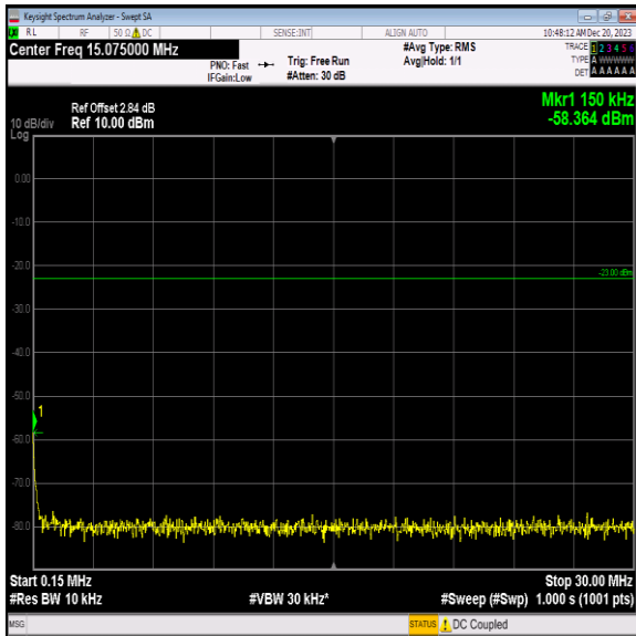
Band5_1.4MHz_QPSK_20525_1RB#0_0.15~30_0.15~30
