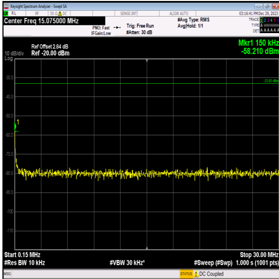
Band2_20MHz_QPSK_18700_1RB#0_0.15~30_0.15~30
