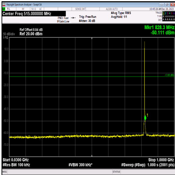
Band5_1.4MHz_QPSK_20407_1RB#0_30~1000_30~1000
