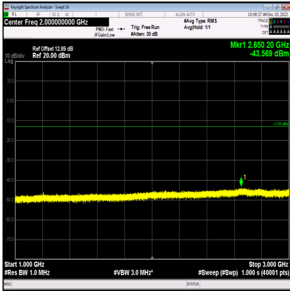
Band5_1.4MHz_QPSK_20525_1RB#0_1000~3000_1000~3000 0
