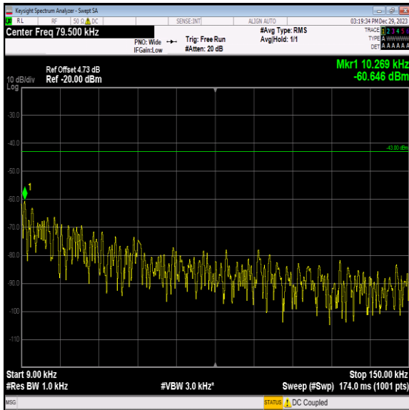
Band2_20MHz_QPSK_18900_1RB#0_0.009~0.15_0.009~0.15 5
