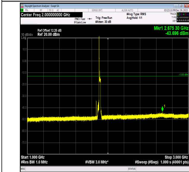
Band2_20MHz_QPSK_19100_1RB#0_1000~3000_1000~300
