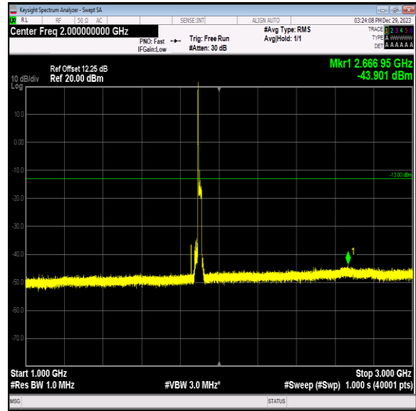
Band2_20MHz_16QAM_19100_1RB#0_1000~3000_1000~3000
