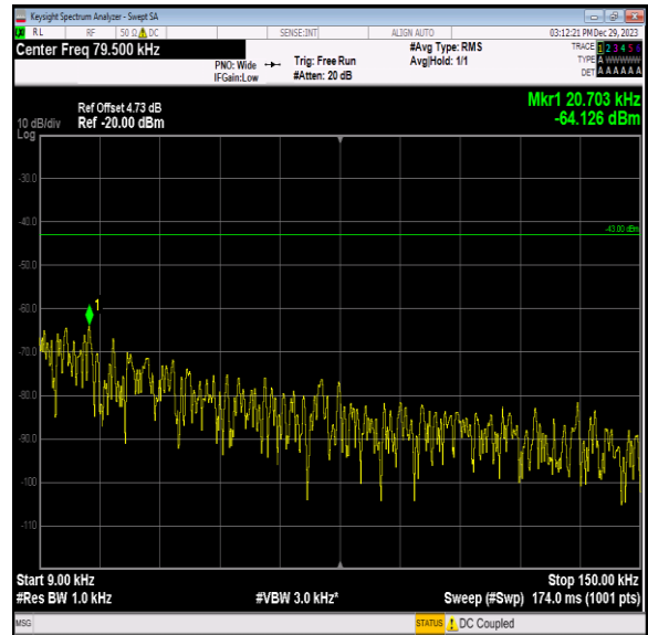
Band2_15MHz_64QAM_18900_1RB#0_0.009~0.15_0.009~0.15
