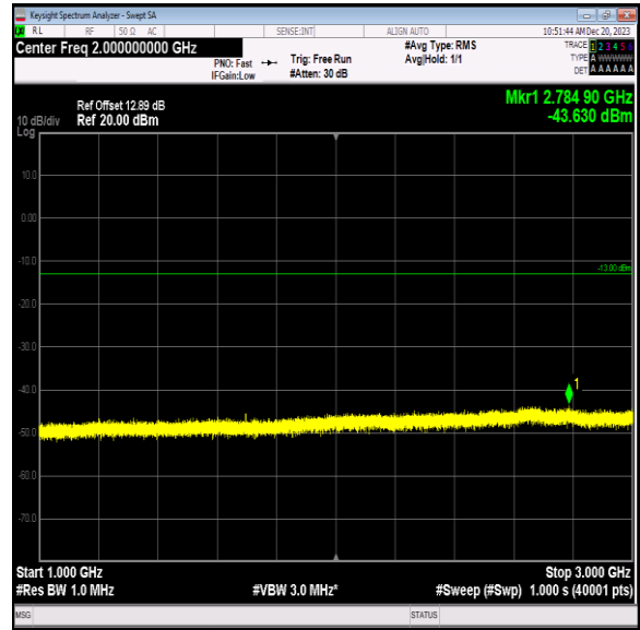
Band5_1.4MHz_QPSK_20643_1RB#0_1000~3000_1000~3000
