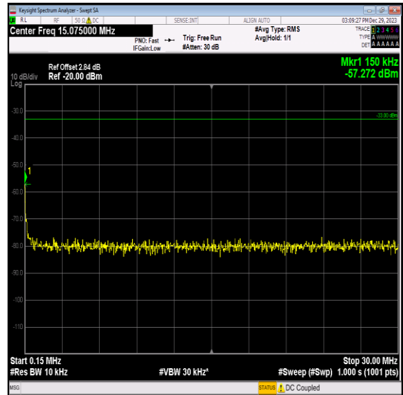
Band2_15MHz_64QAM_18675_1RB#0_0.15~30_0.15~30
