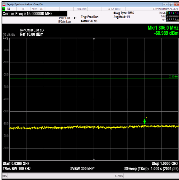
Band2_20MHz_QPSK_18900_1RB#0_30~1000_30~1000
