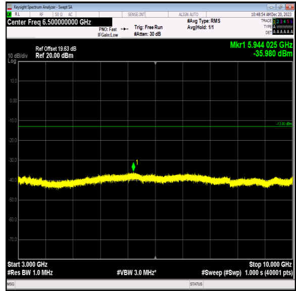
Band5_1.4MHz_QPSK_20525_1RB#0_3000~10000_3000~10000 000
