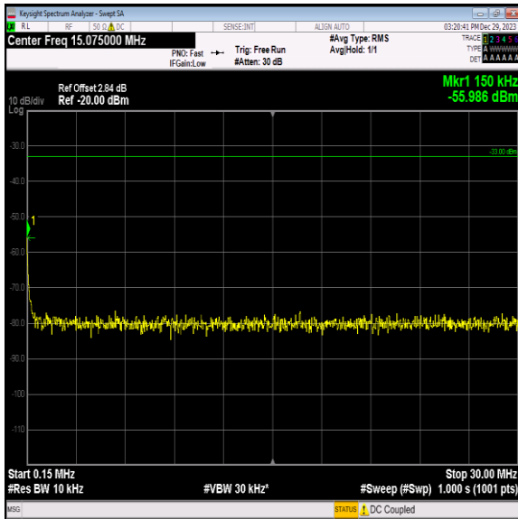
Band2_20MHz_16QAM_18900_1RB#0_0.15~30_0.15~30
