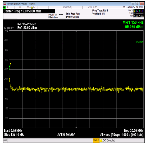
Band2_20MHz_QPSK_18900_1RB#0_0.15~30_0.15~30
