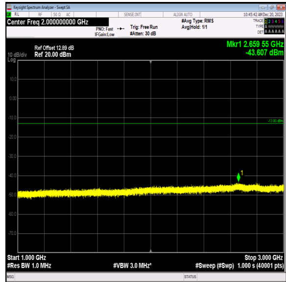
Band5_1.4MHz_QPSK_20407_1RB#0_1000~3000_1000~300 0
