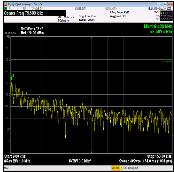
Band2_20MHz_64QAM_19100_1RB#0_0.009~0.15_0.009~0.15
