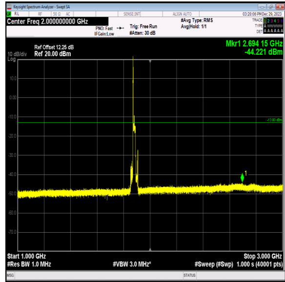
Band2_20MHz_QPSK_18900_1RB#0_1000~3000_1000~3000 0
