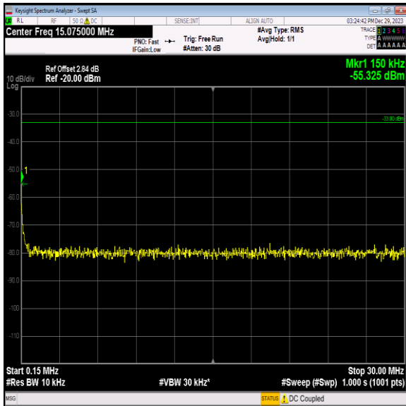
Band2_20MHz_64QAM_19100_1RB#0_0.15~30_0.15~30
