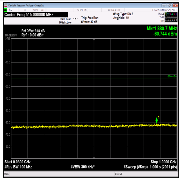
Band2_20MHz_QPSK_19100_1RB#0_30~1000_30~1000
