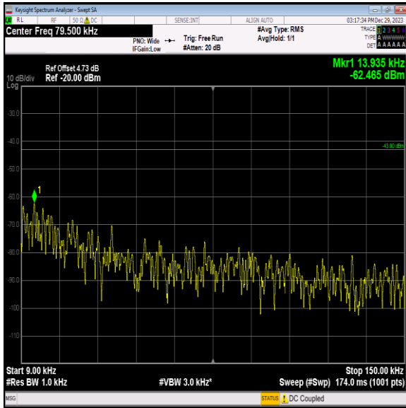
Band2_20MHz_16QAM_18700_1RB#0_0.009~0.15_0.009~0.15
