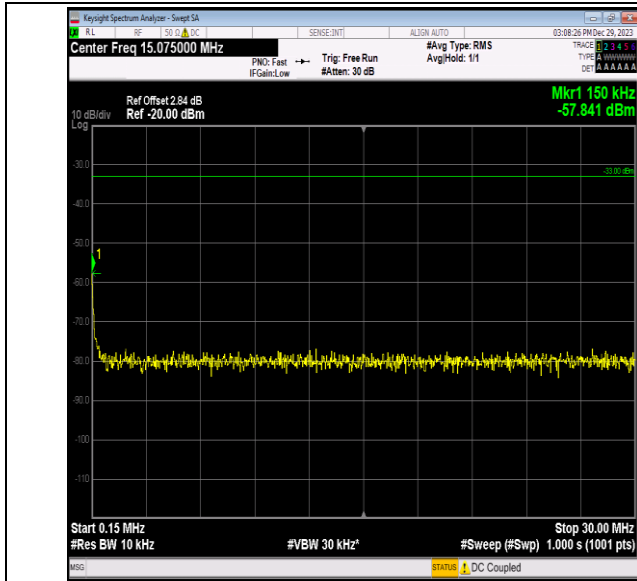
Band2_15MHz_16QAM_18675_1RB#0_0.15~30_0.15~30
