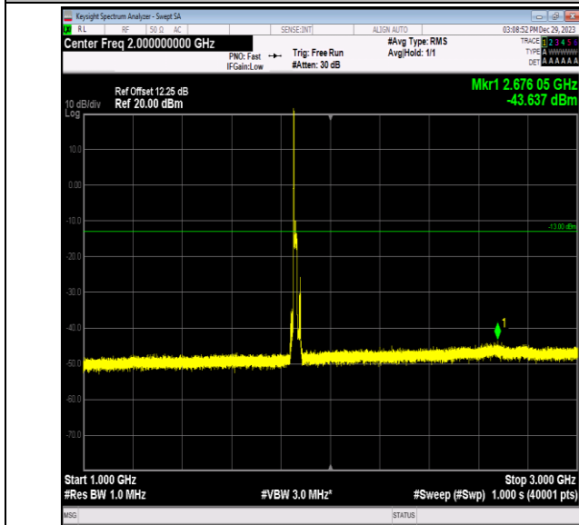
Band2_15MHz_16QAM_18675_1RB#0_1000~3000_1000~3000 00
