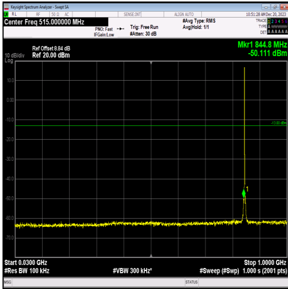
Band5_1.4MHz_QPSK_20643_1RB#0_30~1000_30~1000
