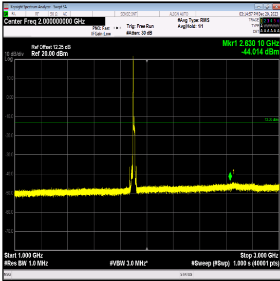
Band2_15MHz_16QAM_19125_1RB#0_1000~3000_1000~30 00
