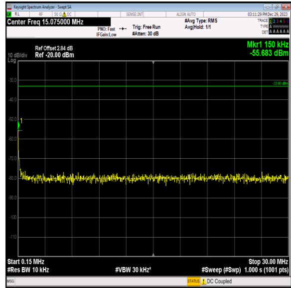
Band2_15MHz_16QAM_18900_1RB#0_0.15~30_0.15~30
