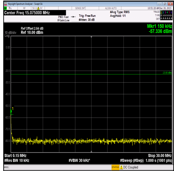
Band5_1.4MHz_QPSK_20643_1RB#0_0.15~30_0.15~30
