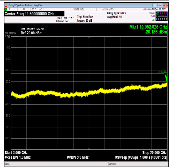
Band2_15MHz_16QAM_18675_1RB#0_3000~20000_3000~20000 0000
