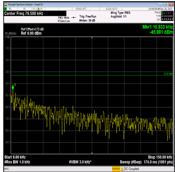
Band5_1.4MHz_16QAM_20407_1RB#0_0.009~0.15_0.009~0.15
