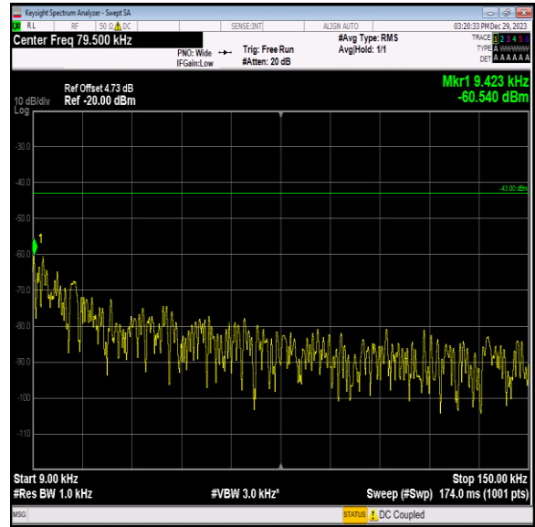
Band2_20MHz_16QAM_18900_1RB#0_0.009~0.15_0.009~0.15 15
