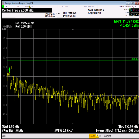
Band5_1.4MHz_QPSK_20643_1RB#0_0.009~0.15_0.009~0.15 5
