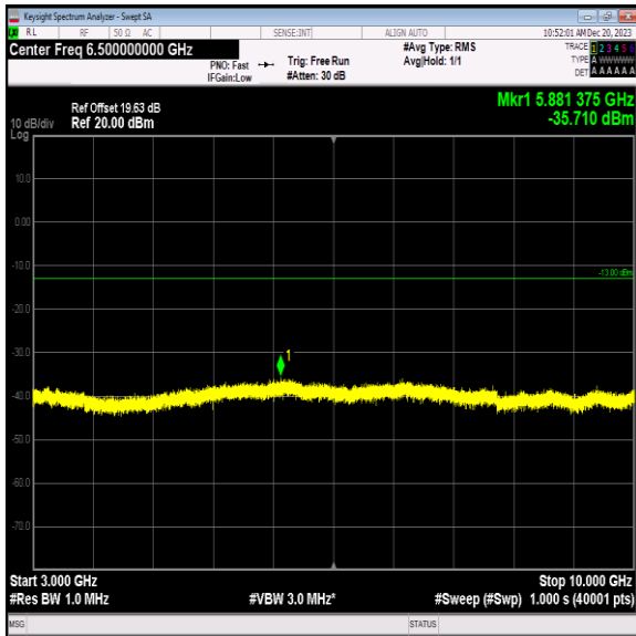
Band5_1.4MHz_QPSK_20643_1RB#0_3000~10000_3000~10000
