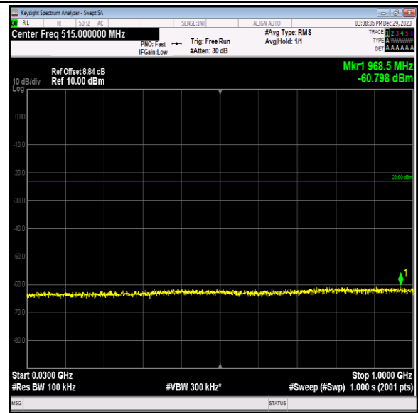
Band2_15MHz_16QAM_18675_1RB#0_30~1000_30~1000
