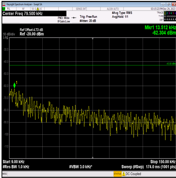
Band2_15MHz_64QAM_19125_1RB#0_0.009~0.15_0.009~0.15
