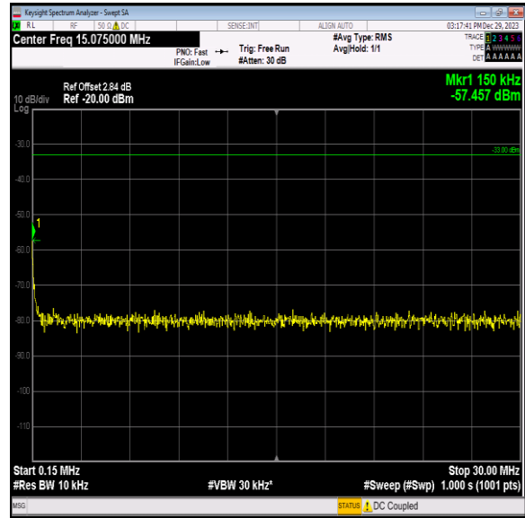
Band2_20MHz_16QAM_18700_1RB#0_0.15~30_0.15~30
