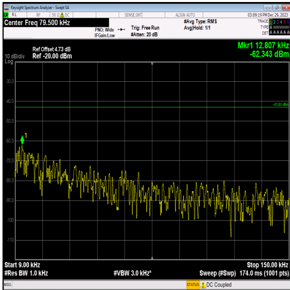
Band2_15MHz_64QAM_18675_1RB#0_0.009~0.15_0.009~0. 15
