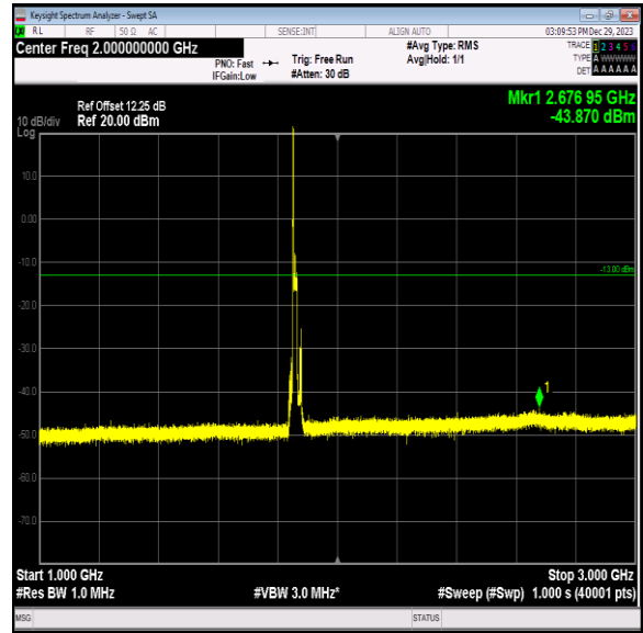
Band2_15MHz_64QAM_18675_1RB#0_1000~3000_1000~3000
