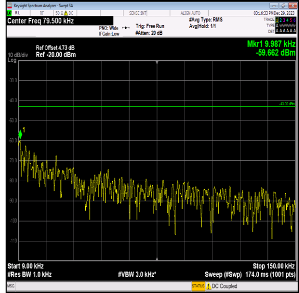
Band2_20MHz_QPSK_18700_1RB#0_0.009~0.15_0.009~0.1
