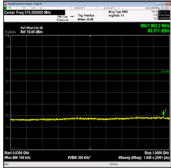
Band2_15MHz_16QAM_19125_1RB#0_30~1000_30~1000
